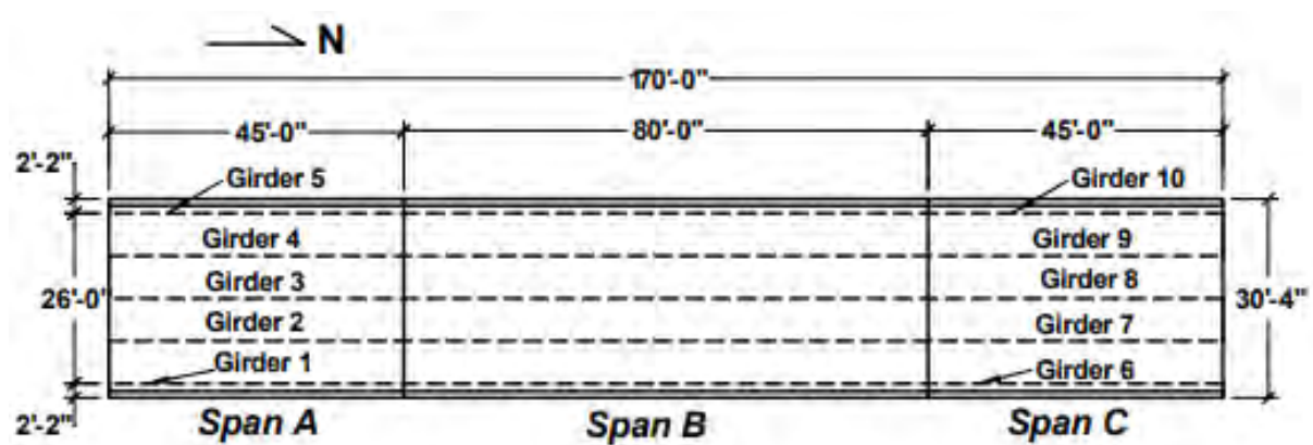
Fig. 1–Gills Creek Bridge
