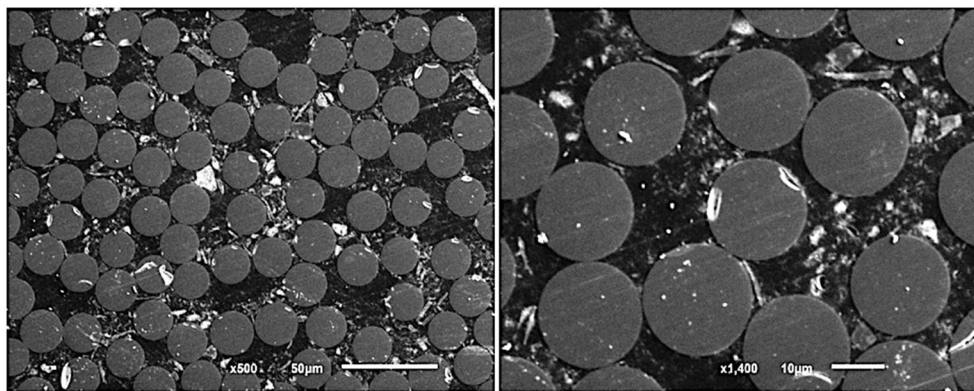
Fig. 114. SEM images of GFRP bar after 11 years of service in Southview Bridge at magnifications of 500x (left) and 1400x (right)
