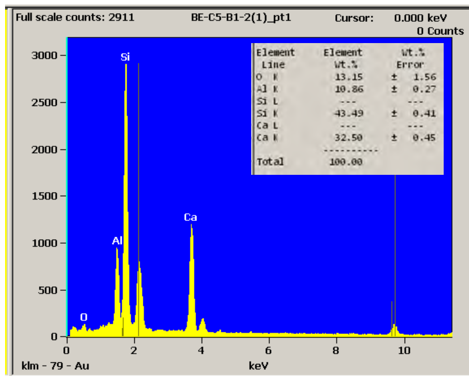
Fig. 122. BE_C5_B1-2 pt. 1 EDS result
