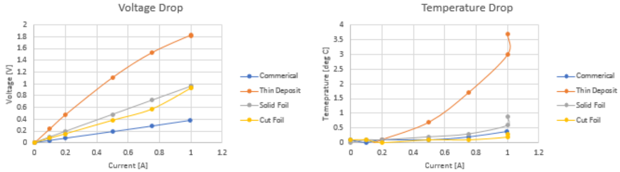
Figure 8: Results of TE couple using nickel contacts in place of silver epoxy
