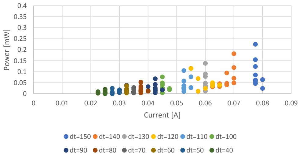
Figure 16: Nano structured bismuth telluride couple power output versus current at differing temperature differentials
