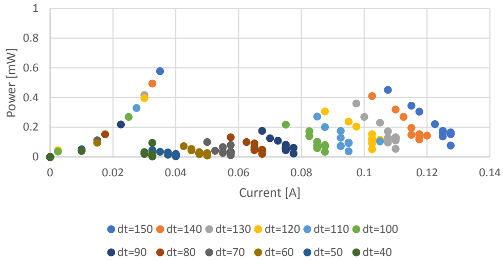
Figure 15: Bulk bismuth telluride couple power output versus current at differing temperature differentials
