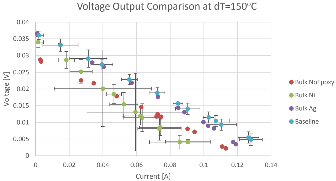
Figure 17: Voltage output versus current at dT=150^{\circ}\text{C} for bulk bismuth telluride couple as compared to commercial material
