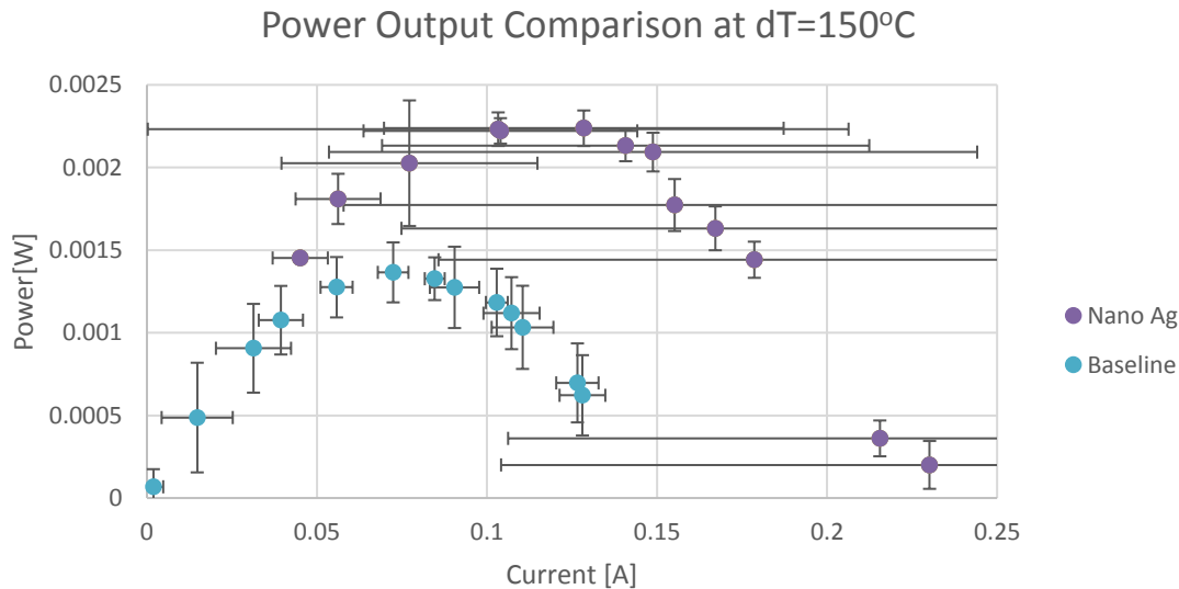
Figure 20: Power output versus current at dT=150^{\circ}\text{C} for nanostructured bismuth telluride couple as compared to commercial material
