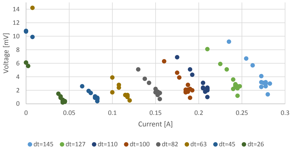
Figure 11: Commercial bismuth telluride couple voltage output versus current at differing temperature differentials
