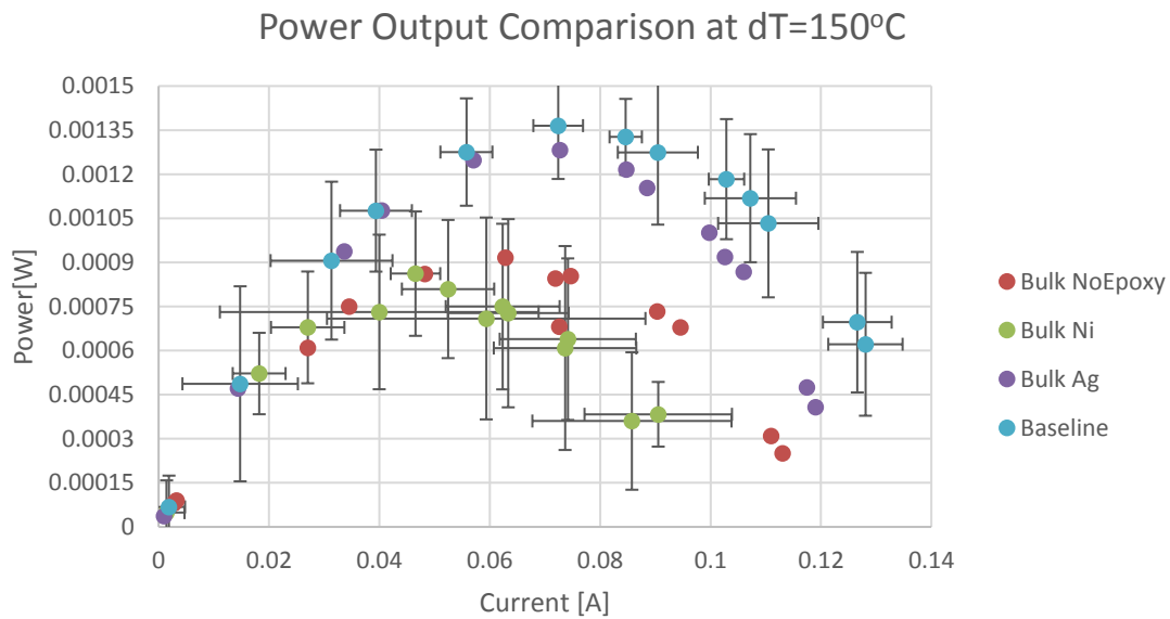
Figure 18: Power output versus current at dT=150^{\circ}\text{C} for bulk bismuth telluride couple as compared to commercial material
