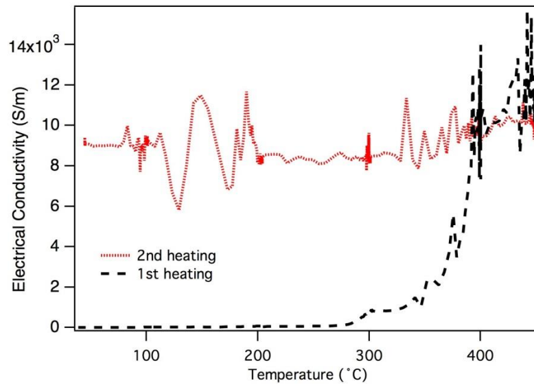
Figure 2: Graph of in-situ electrical conductivity of pellet of nanomaterial, p-type bismuth telluride versus annealing temperature
