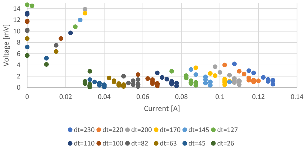
Figure 12: Bulk bismuth telluride couple voltage output versus current at differing temperature differentials
