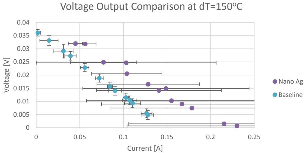
Figure 19: Voltage output versus current at dT=150^{\circ}\text{C} for nanostructured bismuth telluride couple as compared to commercial material
