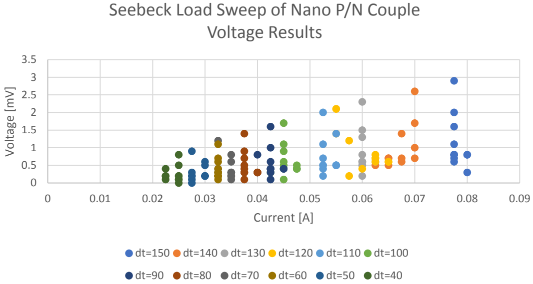
Figure 13: Nano structured bismuth telluride couple voltage output versus current at differing temperature differentials
