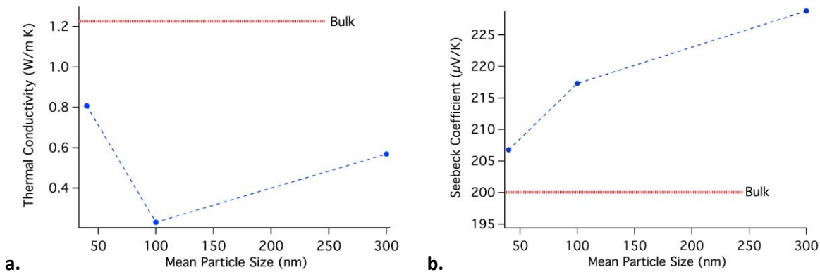
Figure 4: (left) Room temperature thermal conductivity and (right) Seebeck coefficient data from pellets made with p-type Bi 2 Te 3 powder processed to average particle diameters of 40, 100 and 300 nm.
