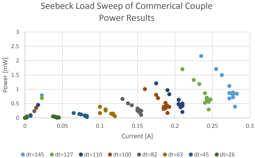
Figure 14: Commercial bismuth telluride couple power output versus current at differing temperature differentials
