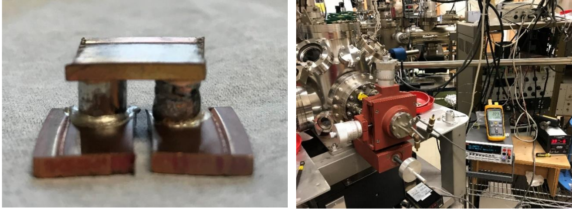
Figure 5: Thermoelectric couple Peltier testing; left, TE couple, right, vacuum chamber testing setup
