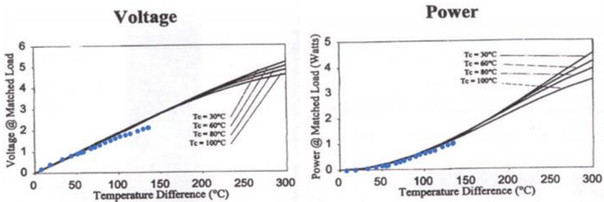
Figure 9: TE Load Bank validation against published output of HZ2 module [5]
