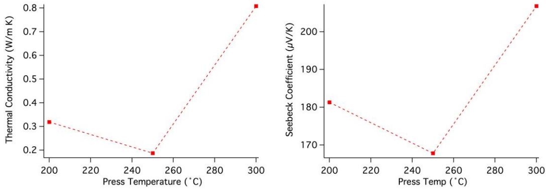
Figure 3: (left) Room temperature thermal conductivity and (right) Seebeck coefficient data from pellets made with 40 nm particle, p-type BiTe powder
