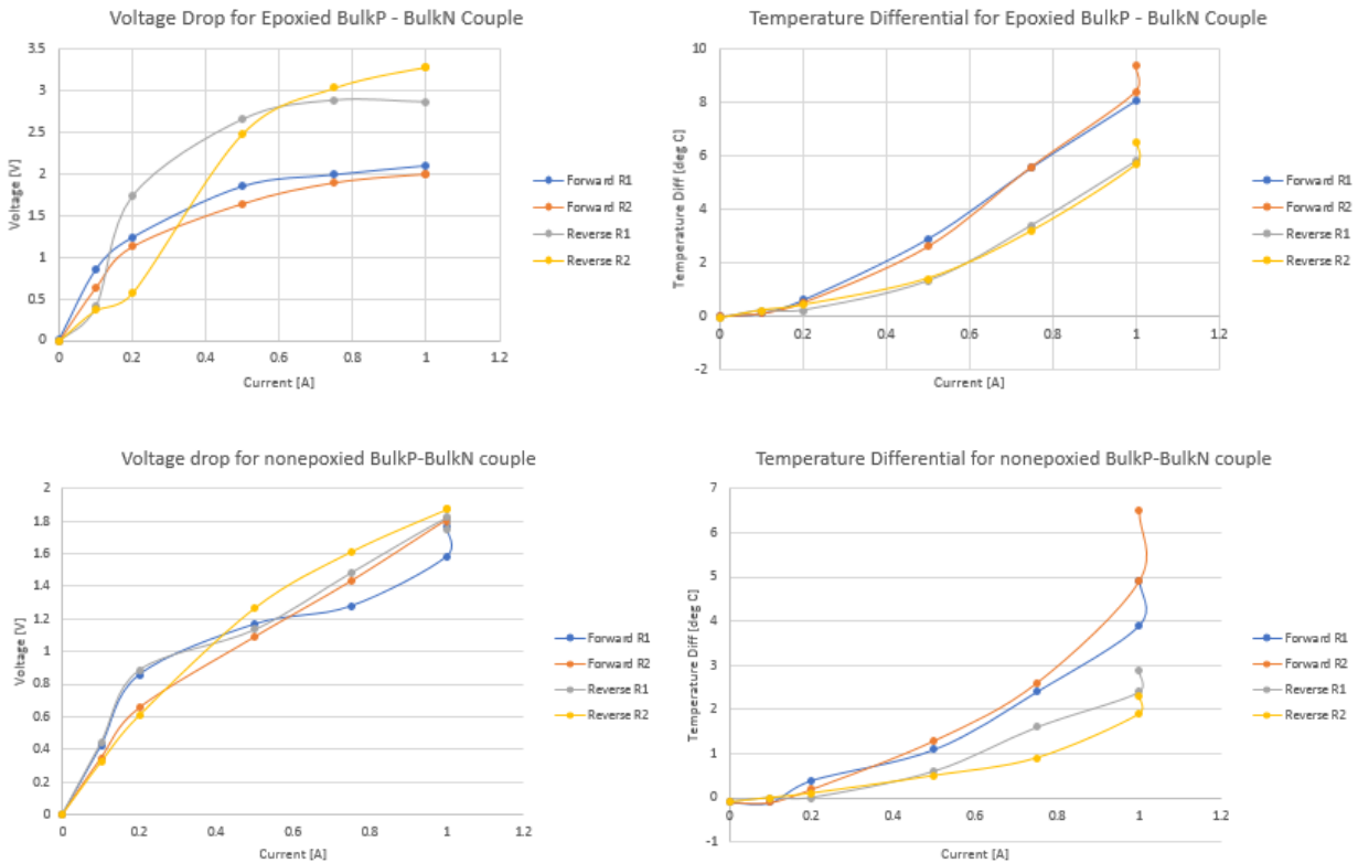
Figure 7: Results of forward and reverse polarity current through TE couple with epoxy and without epoxy
