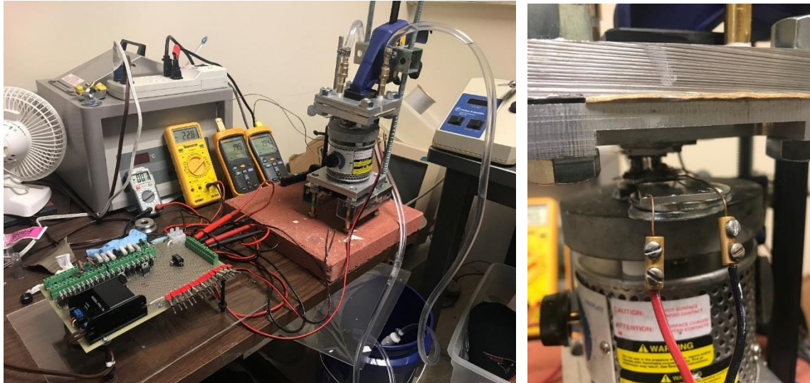
Figure 10: Seebeck TE output evaluation rig (left), TE couple installed in Seebeck test rig (right)
