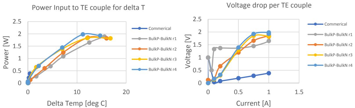
Figure 6: Results from TE Peltier testing; left, temperature differential generated per power input, right, the voltage drop across the TE couple per amp
