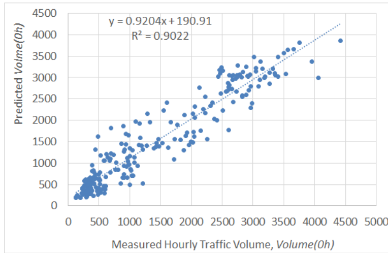
Figure 4.4: Predicted hourly traffic volume vs. actual Volume(0h) from the training dataset
