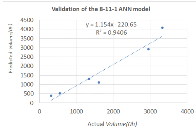
Figure 4.5: Predicted hourly traffic volume vs. actual Volume(0h) from the testing dataset
