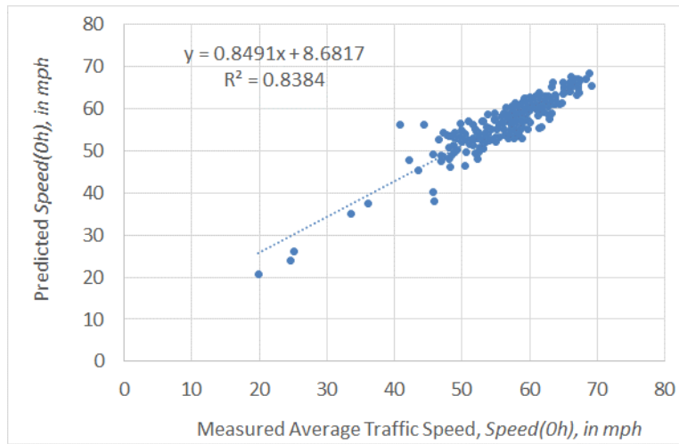
Figure 4.6: Predicted average traffic speed vs. actual Speed(0h) from the training dataset
