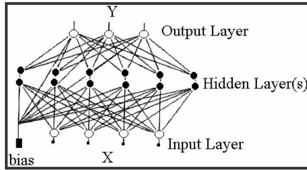
Figure 3.1: Typical Multiplayer Feed-forward Neural Network Architecture (Shi et al. 2004)
