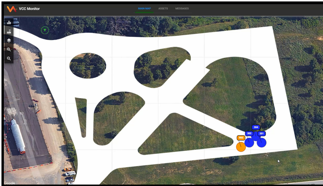
Figure 3. A picture of VCC Monitor, VTTI’s web-based situational awareness tool that displays the real-time locations of UWB anchors and mobile tags (blue circles) and CAVs (orange circle).
