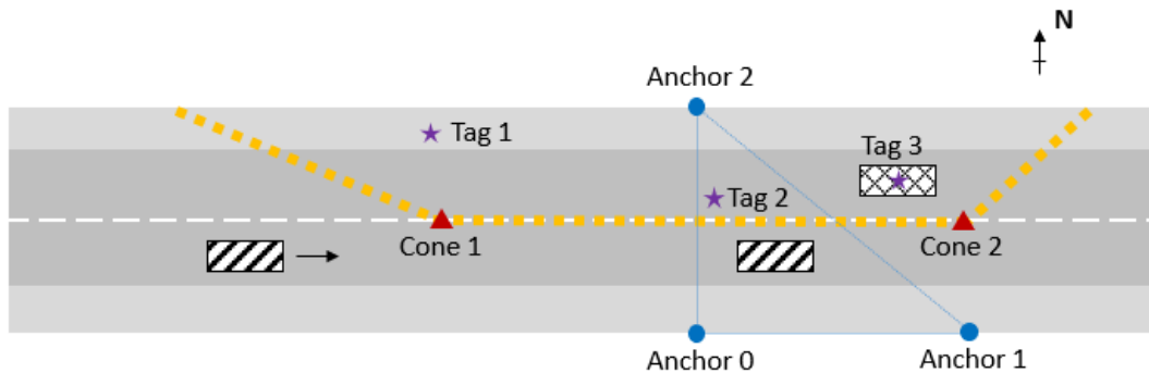
Figure 5. An example of the UWB system setup on the straight roadway section.
