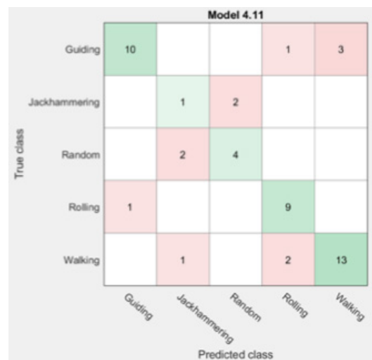
Figure 10. Confusion matrix of ensemble bagged trees.
