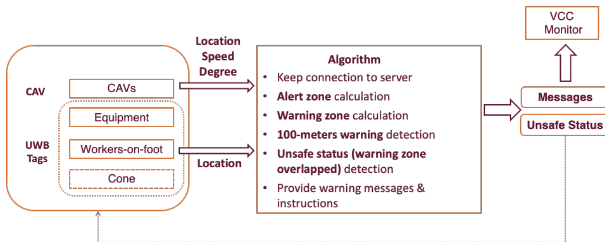
Figure 6. A diagram showing the flow of data in the algorithm.
