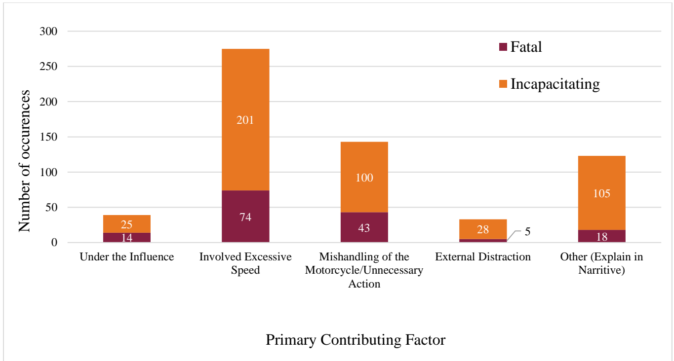
Figure 20. Chart. Various primary contributing factors resulting in KA on curves.
