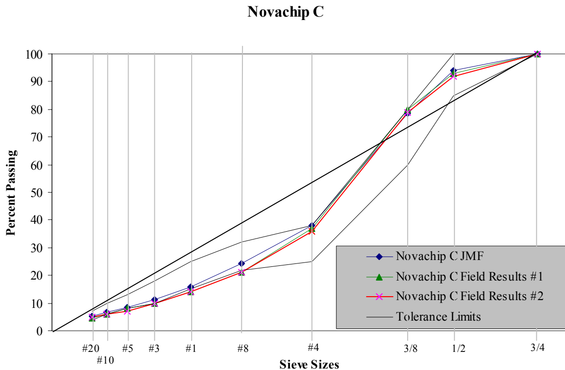
Figure 2. Sieve Sizes 0.45 Power Chart with NovaChip® “C” Job Mix Formula and Production Test Results.
