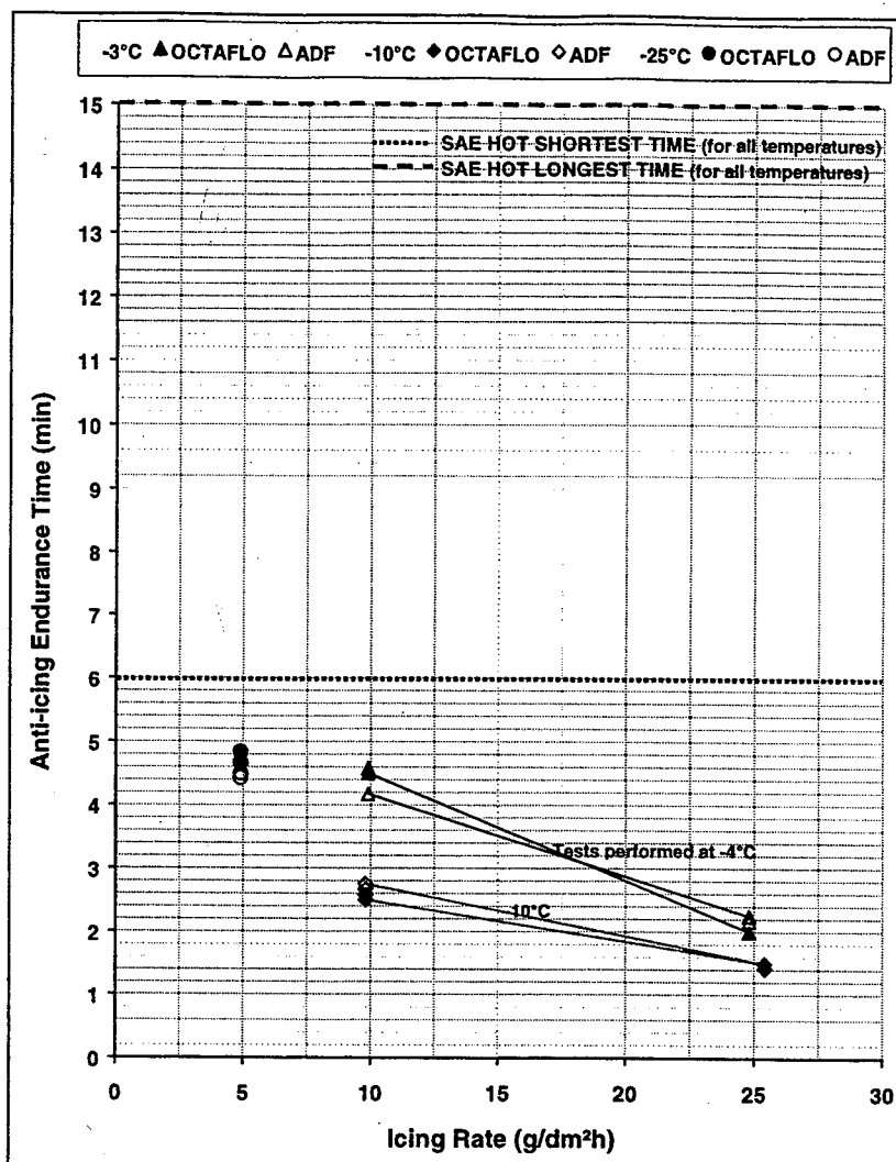
FIGURE 21. SNOW ANTI-ICING ENDURANCE TIMES
