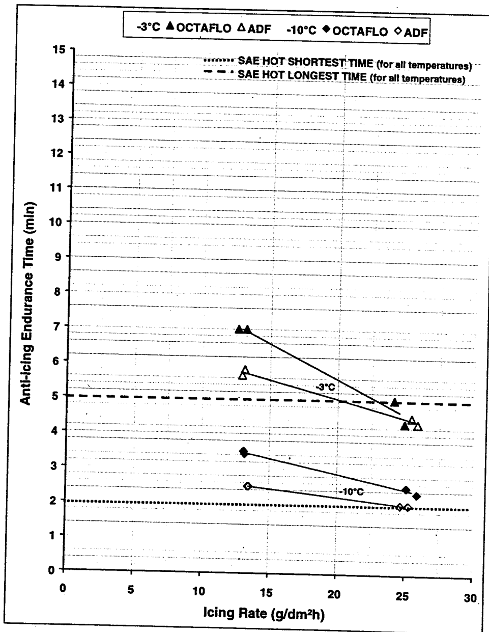
FIGURE 25. LIGHT FREEZING RAIN ENDURANCE TIMES
