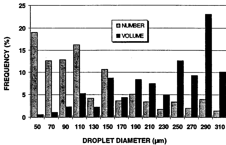
(a) Droplet Size Histogram
