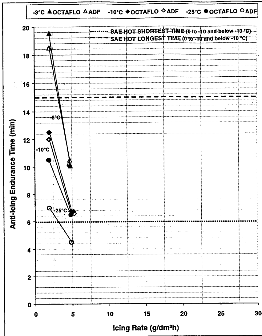
FIGURE 20. FREEZING FOG ENDURANCE TIMES
