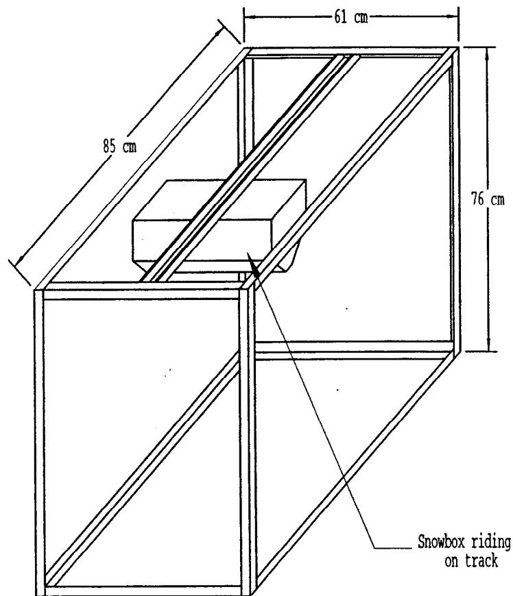
FIGURE 5. SNOW BOX MOUNTED IN ITS SUPPORT ABOVE TEST PLATE
