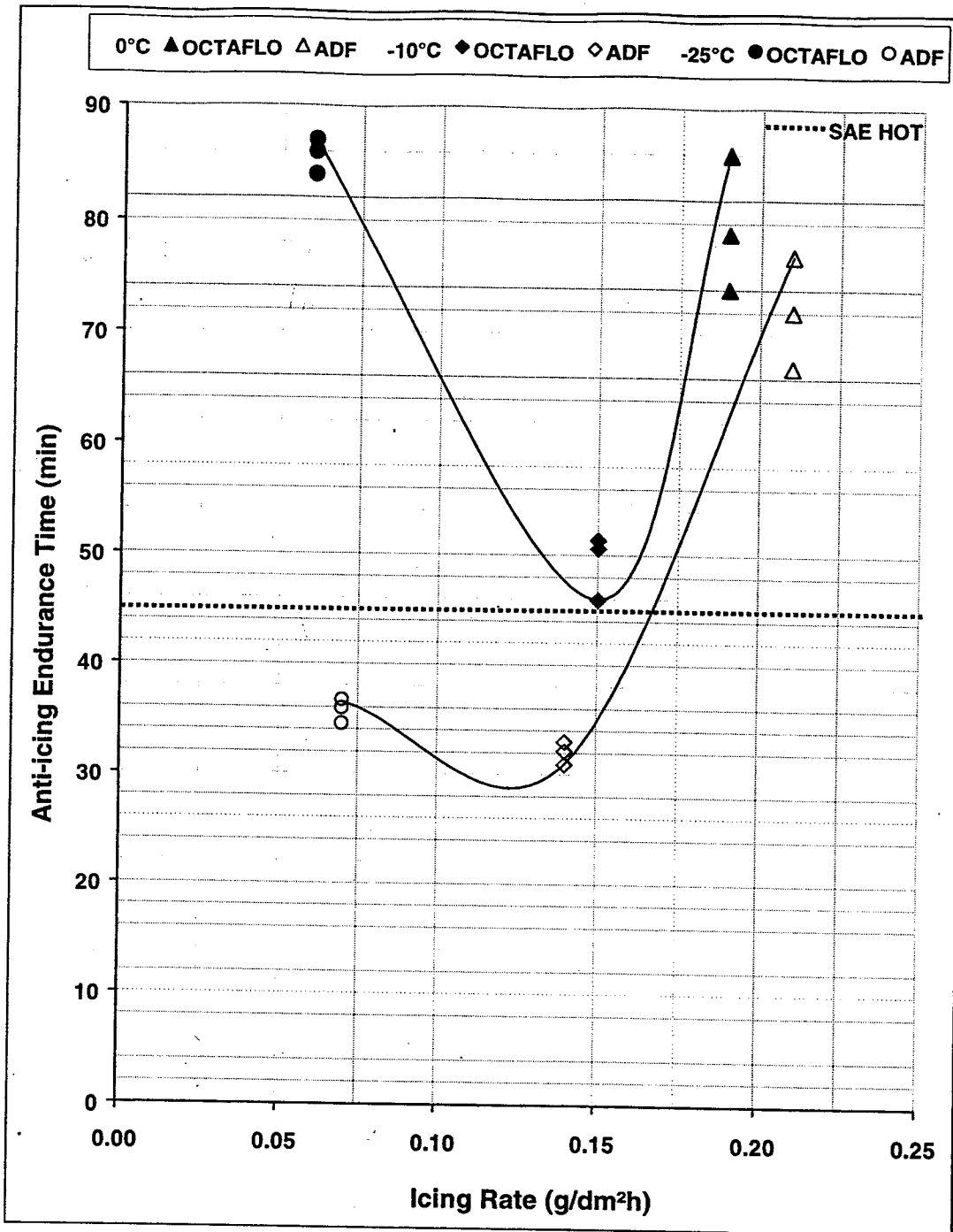
FIGURE 17. FROST ANTI-ICING ENDURANCE TIMES
