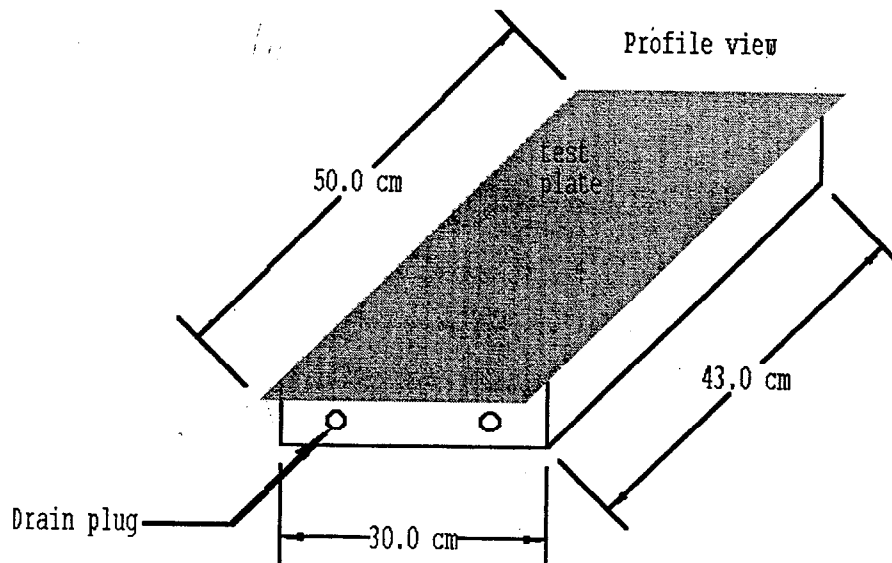
FIGURE 14. COLD SOAK BOX PLATE SETUP
