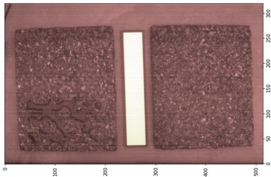
Figure 33: Pika L 320 at 36 °F (2.2 °C). Water visible. 100th wavelength band.
