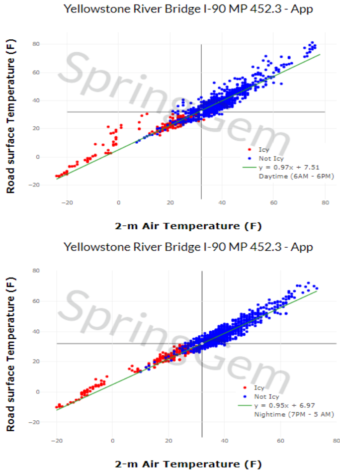
Figure 16: Same as Figure 15, except for (a) daytime (6 AM – 6 PM) and (b) nighttime (7 PM to 5 AM), respectively.
