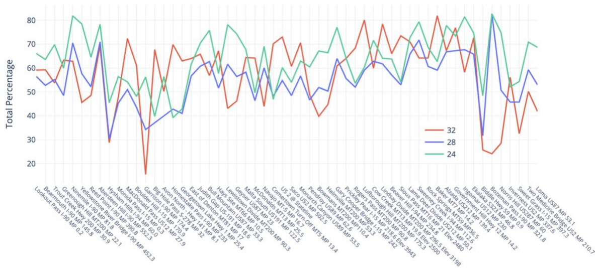
Figure 9: Same as Figure 8 except for March 2020.
