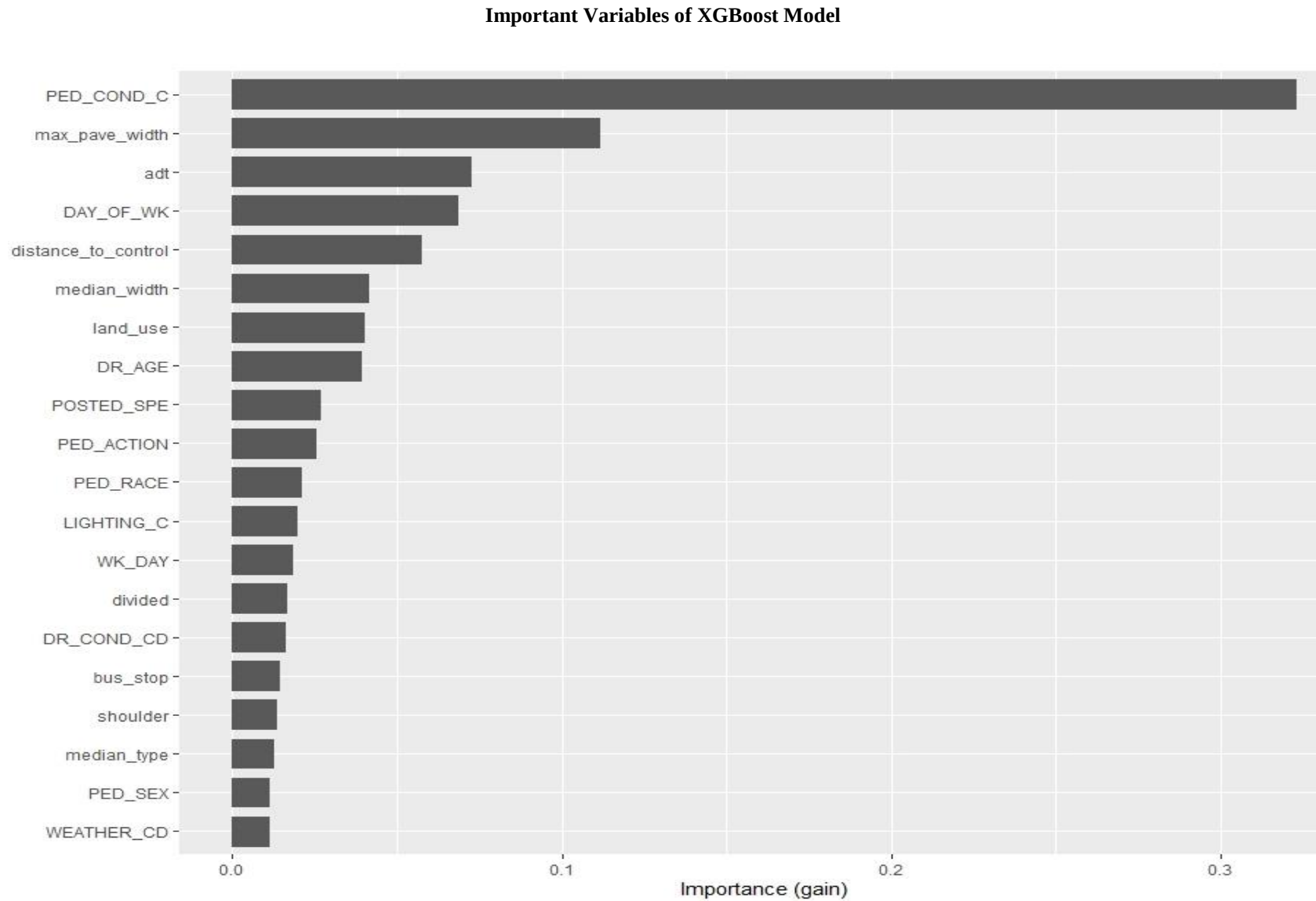
Figure F3. Ranking of importance of predictors for XGBoost model
