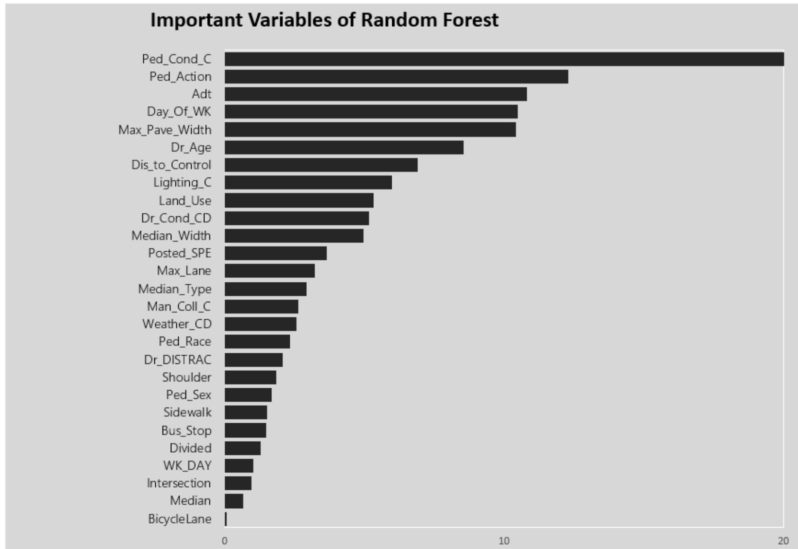
Figure F2. Ranking of importance of predictors for random forest (RF) model
