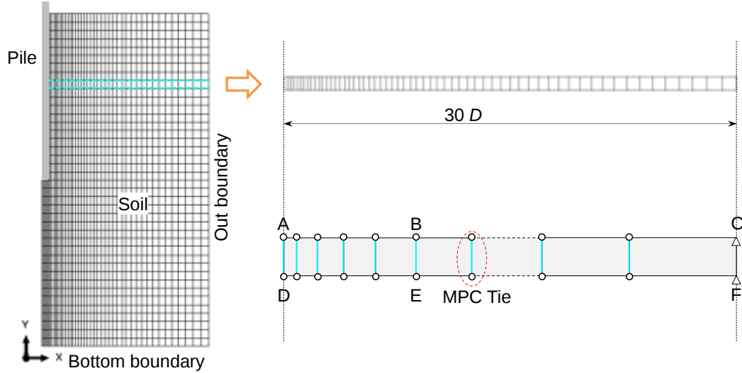
Figure 3. Geometry and boundary condition of finite element model
