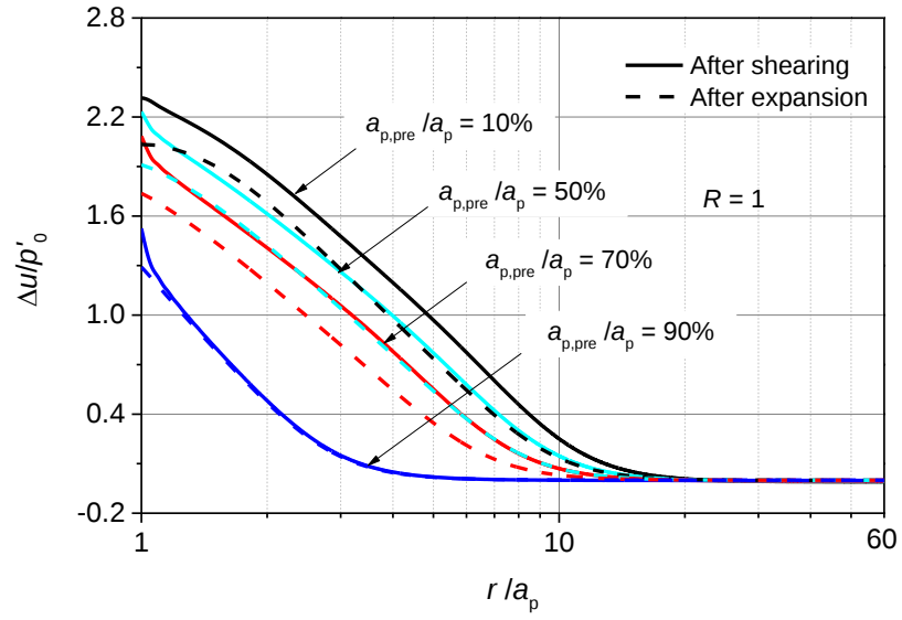
Figure 41. Distribution of excess pore water pressure around piles with different sizes of pre-bored hole immediately after expansion and after shearing: (a) R = 1 ; (b) R = 3
