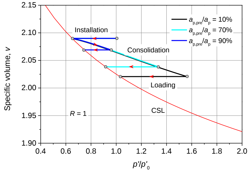
Figure 53. p' - v curve of a soil element at pile shaft for different sizes of pre-bored hole: (a) R = 1 ; (b) R = 3
