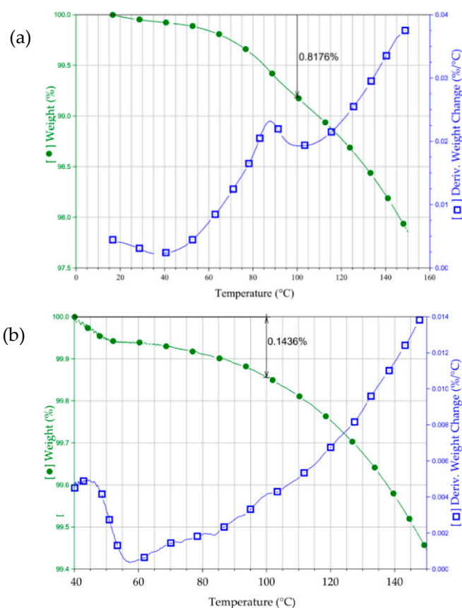
Figure 8. Moisture investigation of guayule resin by TGA: (a) As-received material, and (b) after 4 h heat treatment at 160 °C, and 600 rpm.
