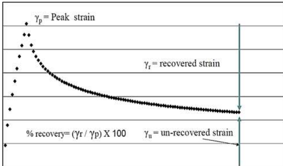
Figure 4 Details of MSCR loading cycle
