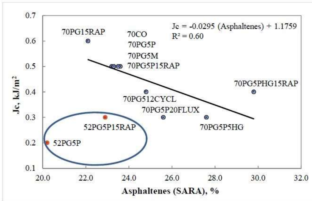
Figure 39 Mixture critical strain energy release rate ( J_c ) vs. asphaltenes content obtained from SARA fractionation
