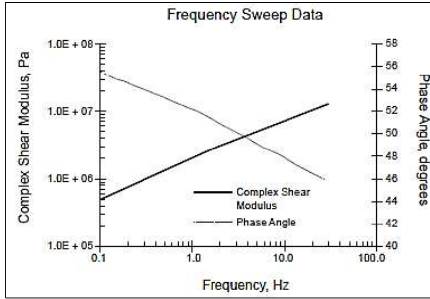
Figure 6 Example output from frequency sweep test (AASHTO TP 101)
