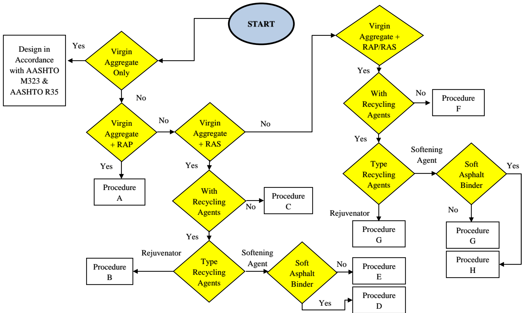
Figure 19 Mix design flow chart
