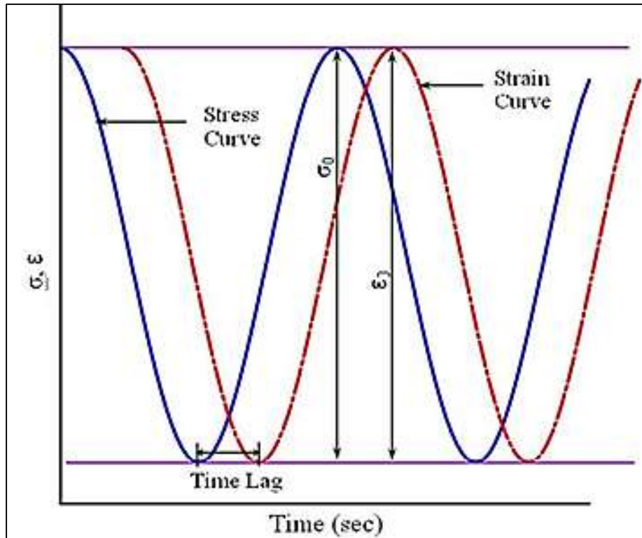
Figure 12 Mixture stress-strain response under sinusoidal load
