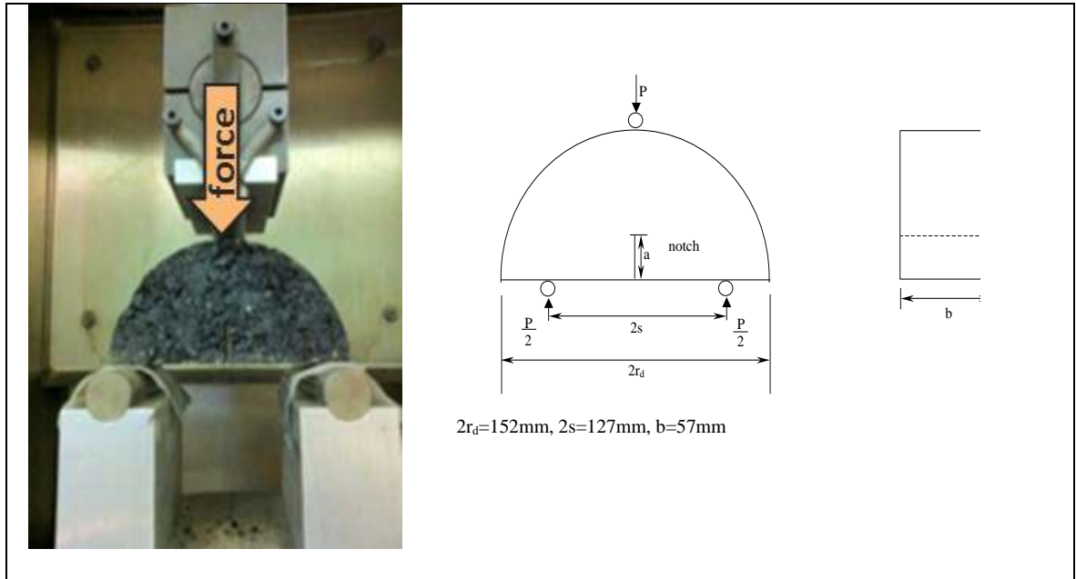
Figure 16 Set-up of semi-circular bending test
