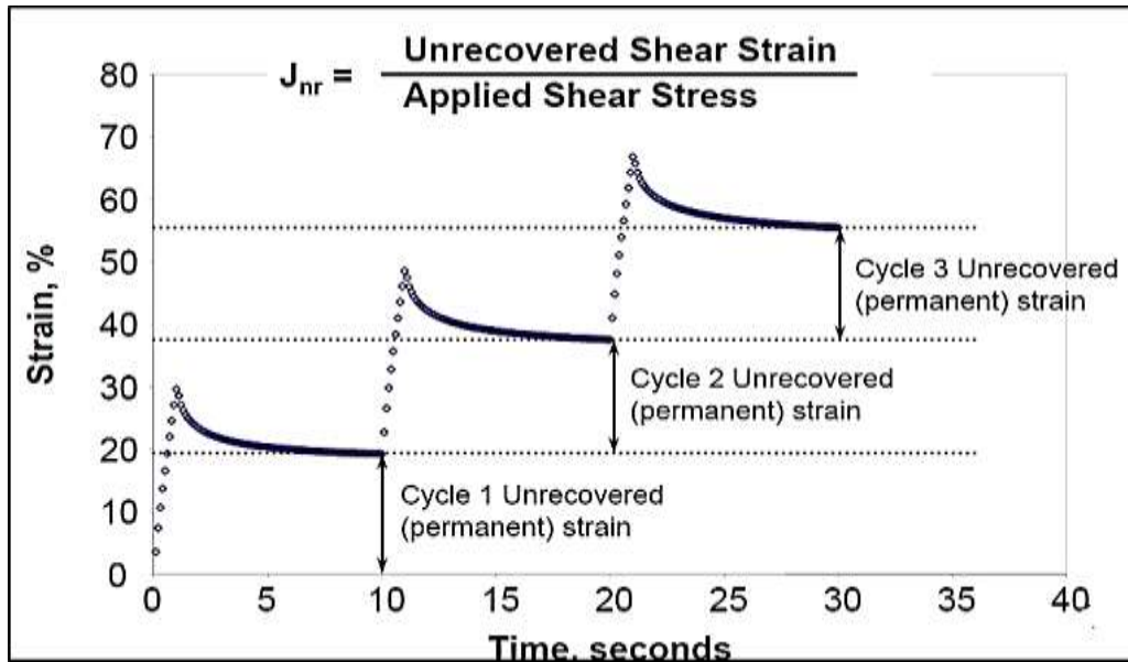
Figure 3 MSCR loading vs. unloading sequence
