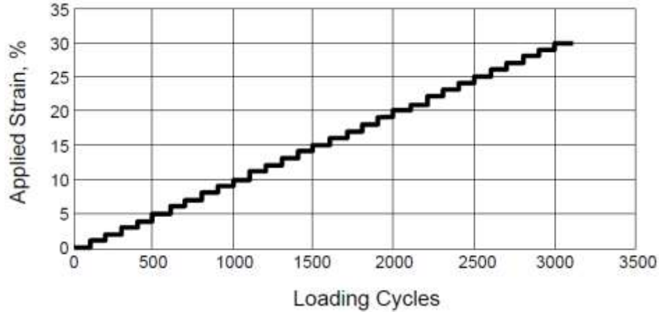
Figure 7 Loading scheme of linear amplitude sweep test (AASHTO TP 101)
