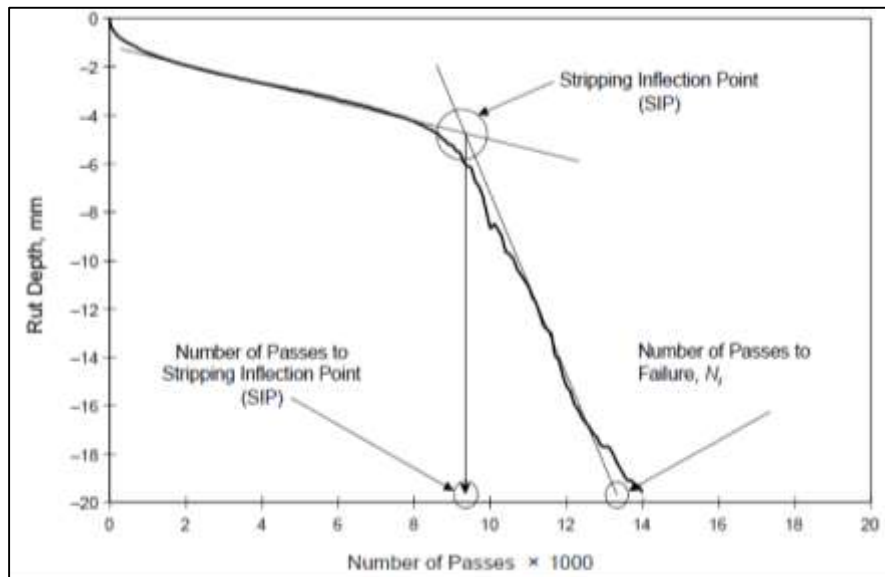
Figure 15 Hamburg curve with test parameters, (AASHTO T 324)
