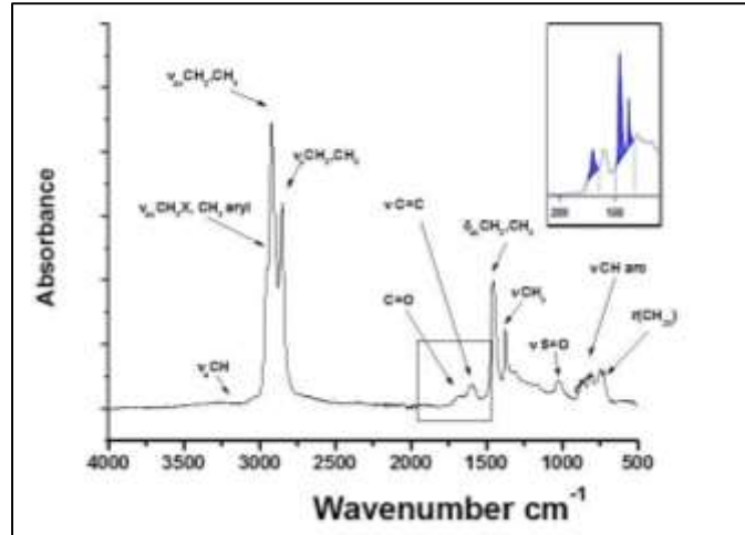
Figure 9 Typical FTIR spectrum of an aged asphalt
