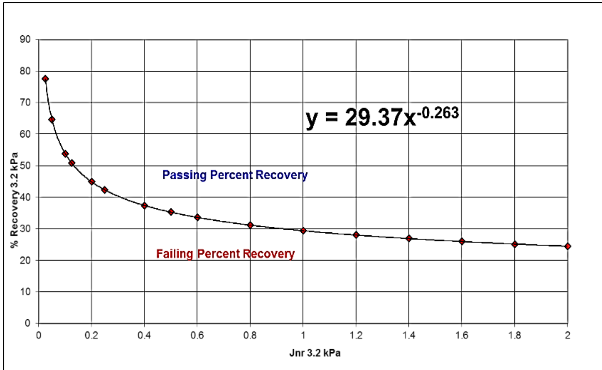
Figure 5 Elastic response curve (AASHTO TP 70)
