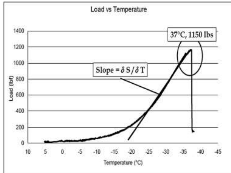
Figure 17 Typical load vs. temperature graph
