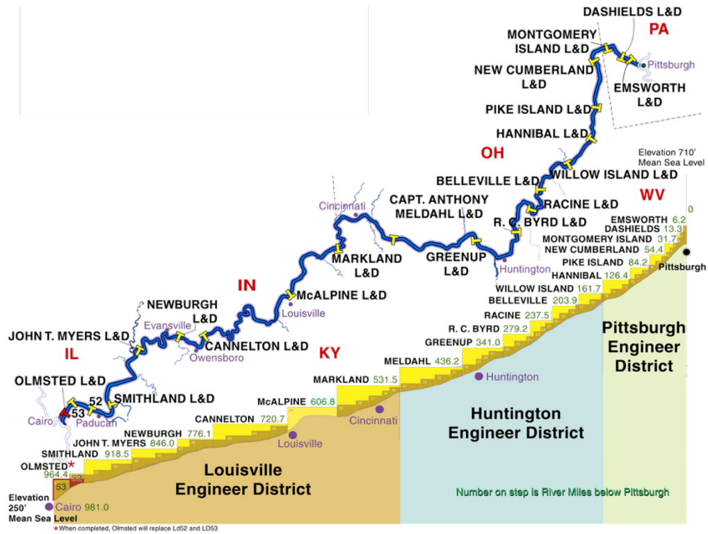
Figure 1 The Ohio River Corridor (Source: (U.S. Army Corps of Engineers, 2012))
