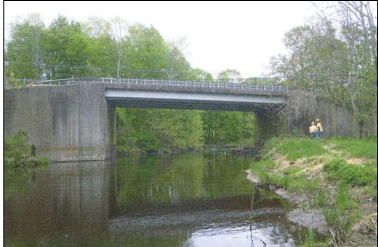
Like the previous bridge, Bridge 01527 consists of parallel steel I-beams set on concrete abutments. Built in 1949, it carries Route 191 over the Scantic River in Enfield.
