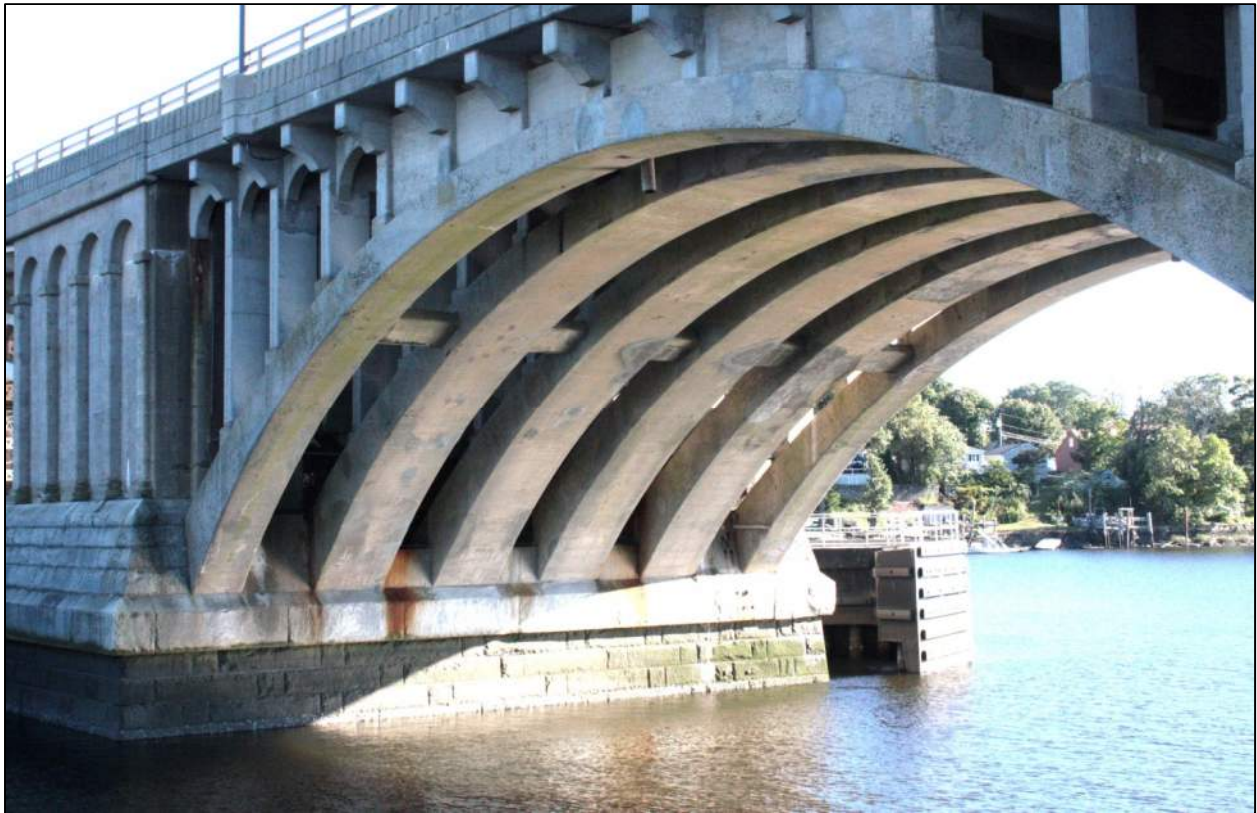
Closer view of concrete arch ribs, typical open-spandrel span, camera facing southeast.
