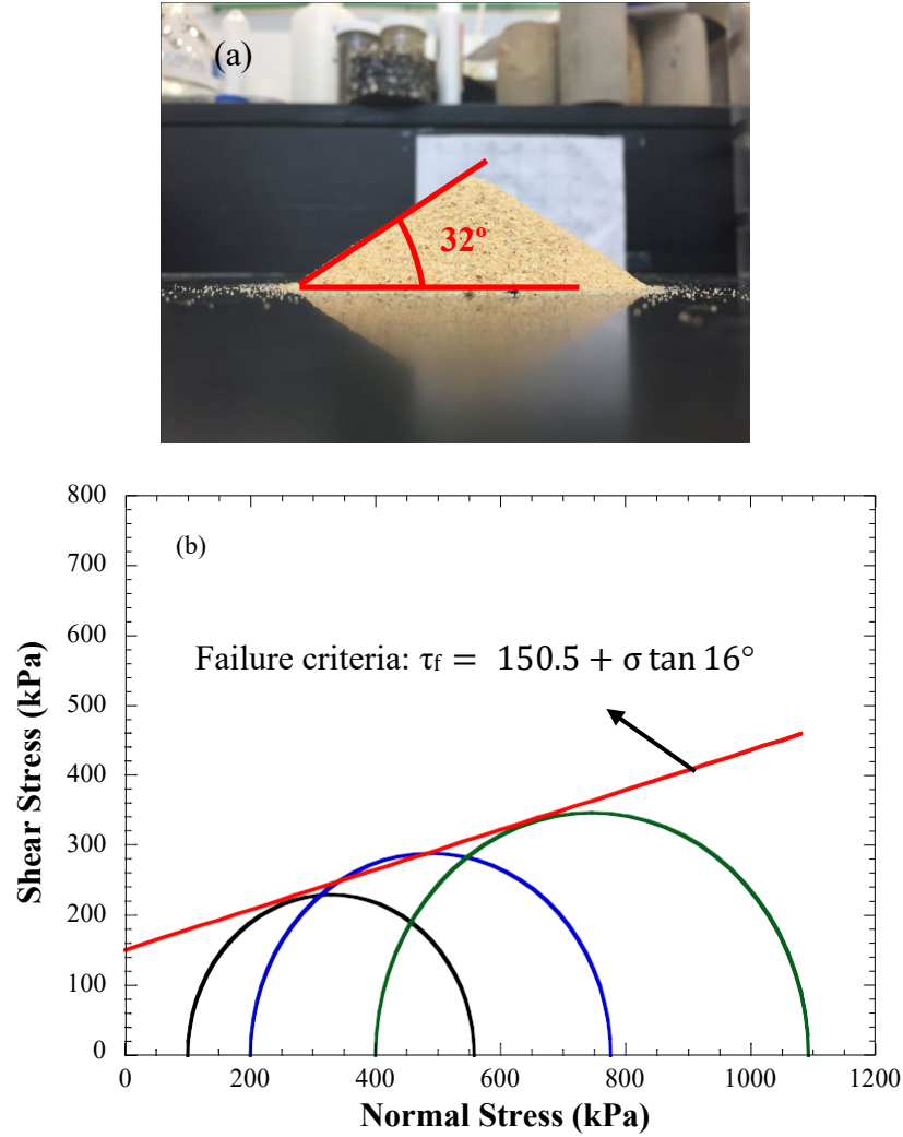
Fig. 11 (a) The nature repose angle of Mississippi sand; (b) Mohr circle and failure envelop of hydrogel-impregnated sand with 0.4% sodium alginate.
