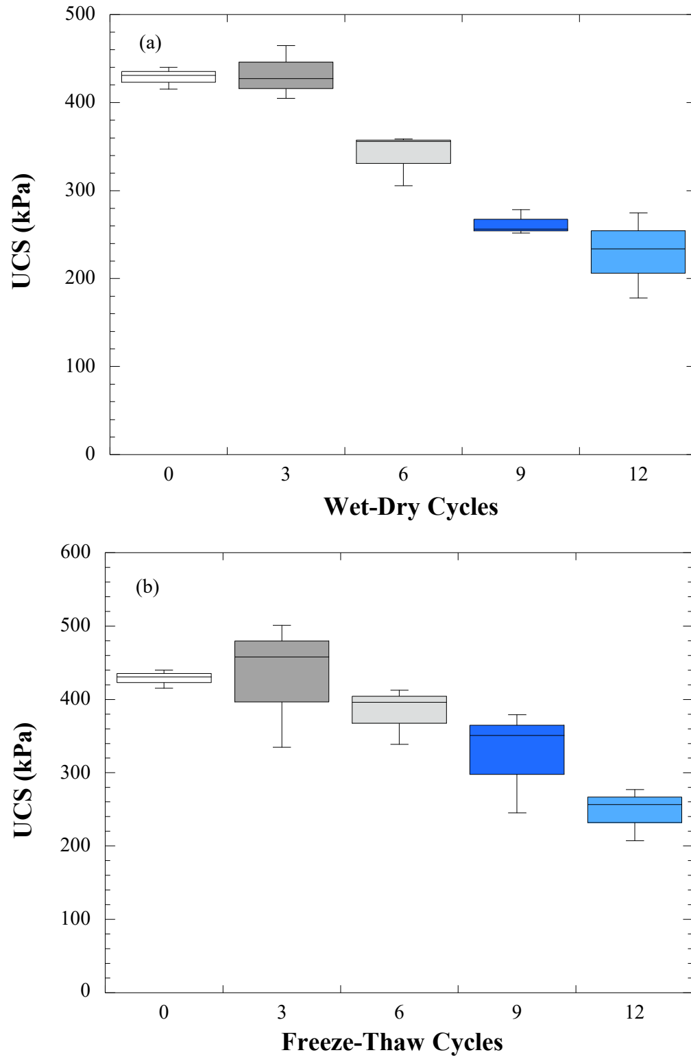
Fig. 12 The effect of wet-dry (a) and freeze-thaw (b) cycles on unconfined compressive strength of hydrogel-impregnated sand
