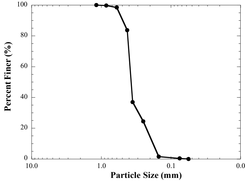
Fig. 3 Particle distribution curve of Mississippi local sand.
