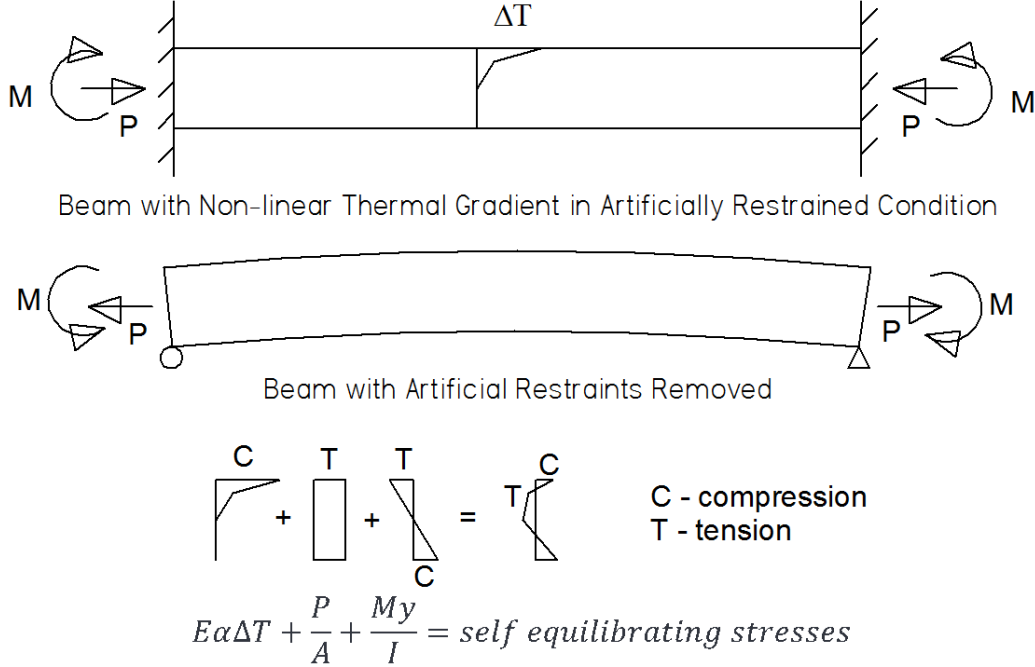
Figure 3. Calculation of Self-Equilibrating Stresses from a Non-Linear Thermal Gradient. M = moment, P = axial force, E = modulus of elasticity, α = coefficient of thermal expansion, ΔT = temperature difference with respect to reference temperature, A = cross-sectional area, I = moment of inertia, y = distance from centroid of section to point under consideration
