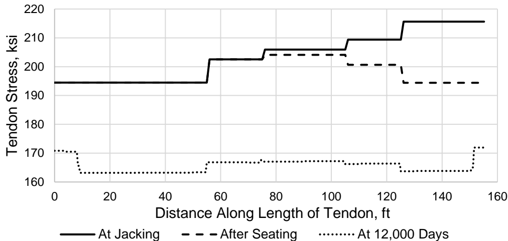
Figure 19. Tendon T9 Left in Span 6 Stress Profile
