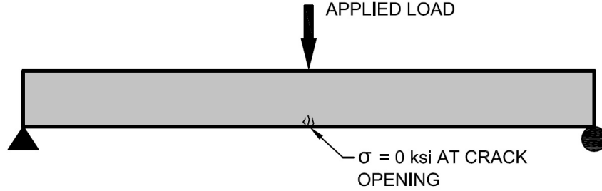
Figure 23. Testing Configuration Employed by Pessiki et al. (1996)
