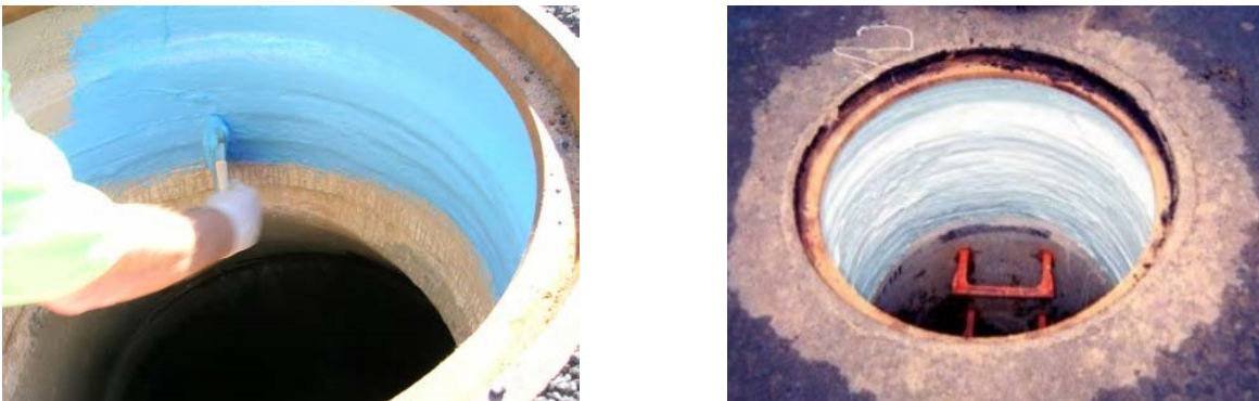
Figure 13. (a) Flex Seal being applied to a manhole chimney interior; (b) Chimney interior after Flex Seal application.
