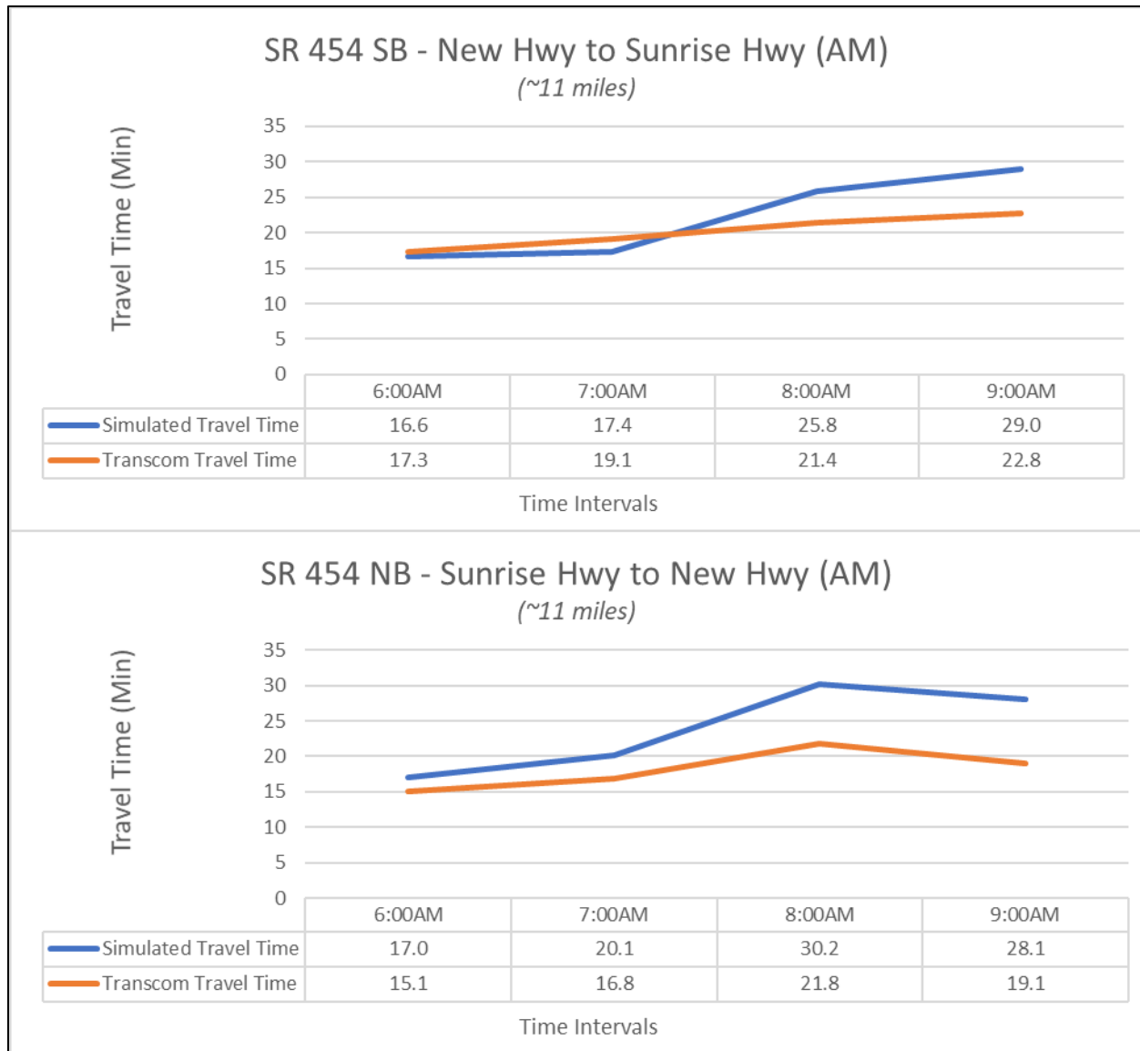
Figure A-12. AM Travel Time Validation—SR 454 from New Hwy to Sunrise Hwy
