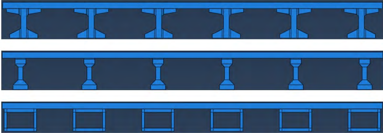
Figure 6.1. Typical Idealized Bridge Cross-Sections.
