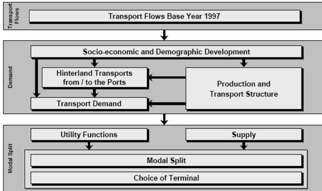
Figure 5: SIMUGV structure
