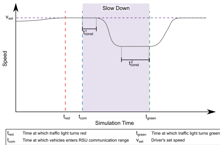
Figure 39: Idealized Vehicle Behavior for the Slow-down Scenario
