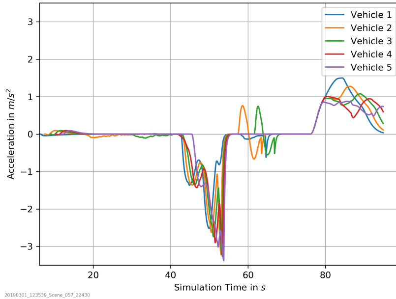
Figure 81: Coordinated Stop and Launch with Dissipating Queue at Intersection Scenario: Simulation Time vs. Acceleration for TOSCo-enabled Vehicles at 35 mph Speed Limit
