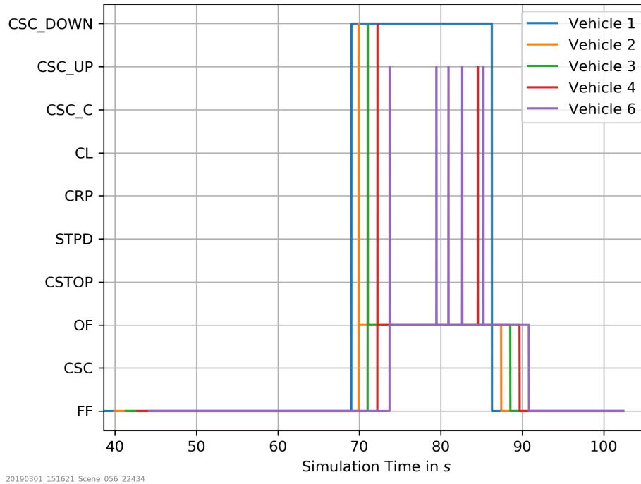
Figure 72: Slow-down with Dissipating Queue at Intersection Scenario: Simulation Time vs. TOSCo Operating Mode for TOSCo-enabled Vehicles at 0.6 s Time Gap at Vehicle 1 Introduction Time of 39 s
