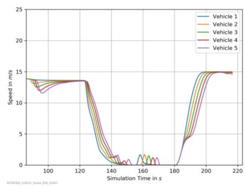
Figure 86: Creep at Intersection Scenario: Simulation Time vs. Speed for TOSCo-enabled Vehicles at 1.5 s Time Gap with Large Distance Gap
