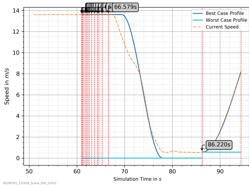
Figure 76: Slow-down with Dissipating Queue at Intersection Scenario: Simulation Time vs. Computed Speed Profiles for Vehicle 1 for 0.6 s Time Gap and Vehicle 1 Introduction Time of 32 s
