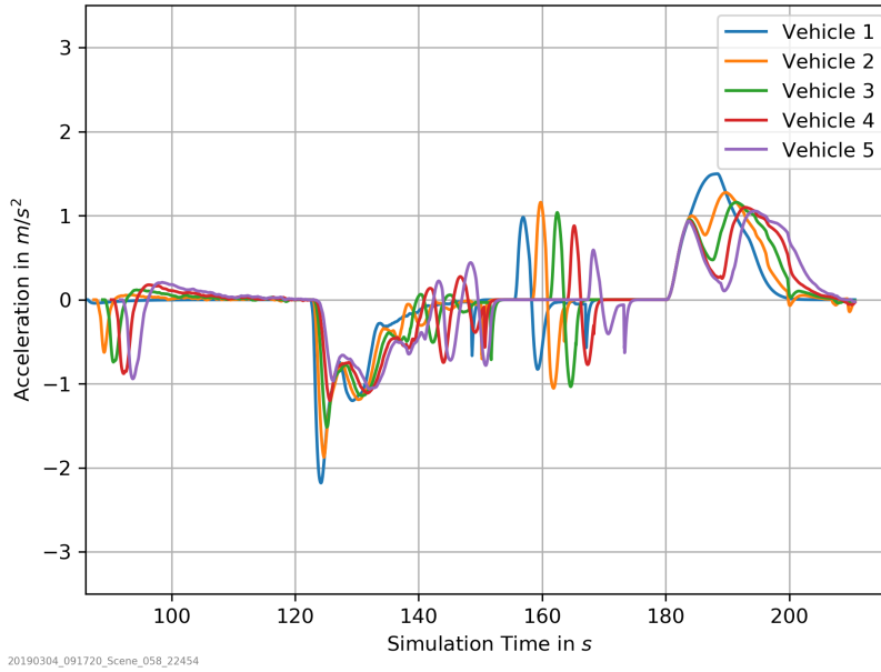
Figure 125: Creep at Intersection Scenario: Simulation Time vs. Acceleration for TOSCo-enabled Vehicles at 1.5 s Time Gap and Small Distance Gap
