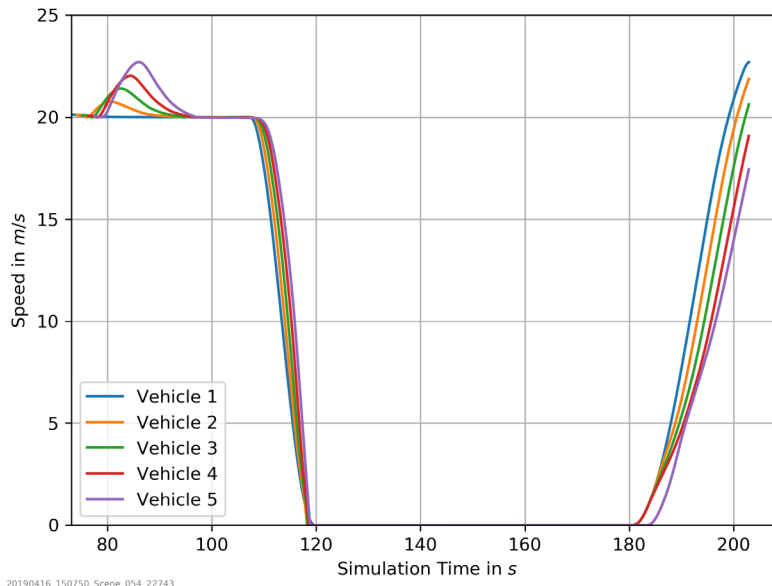
Figure 109: Coordinated Stop and Launch Scenario: Simulation Time vs. Speed for TOSCo-enabled Vehicles at 0.6 s Time Gap and 55 mph Speed Limit
