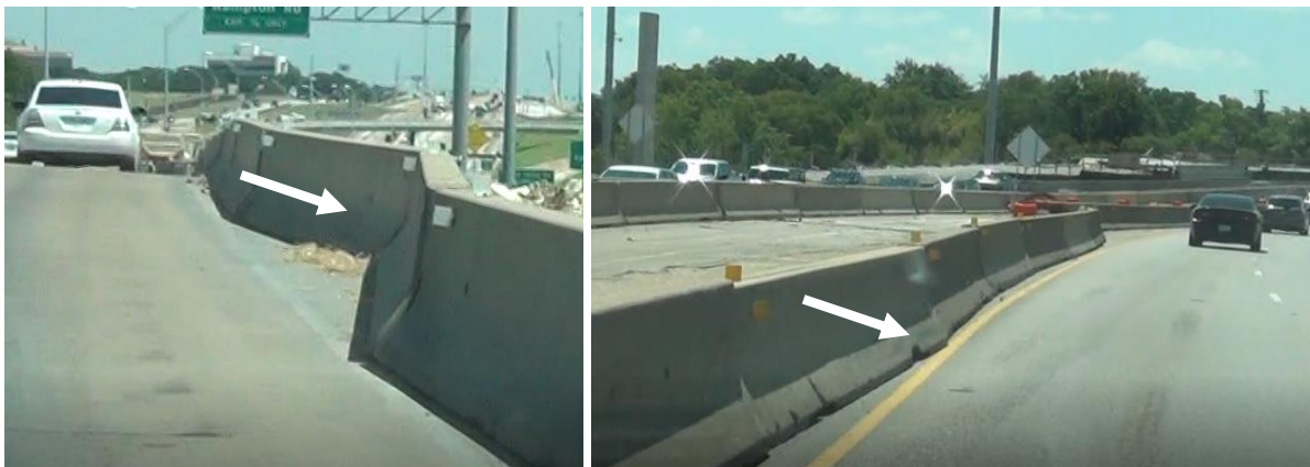
Figure 9. Examples of Barriers Deflected by Traffic Impacts (Left) or Construction Equipment (Right).
