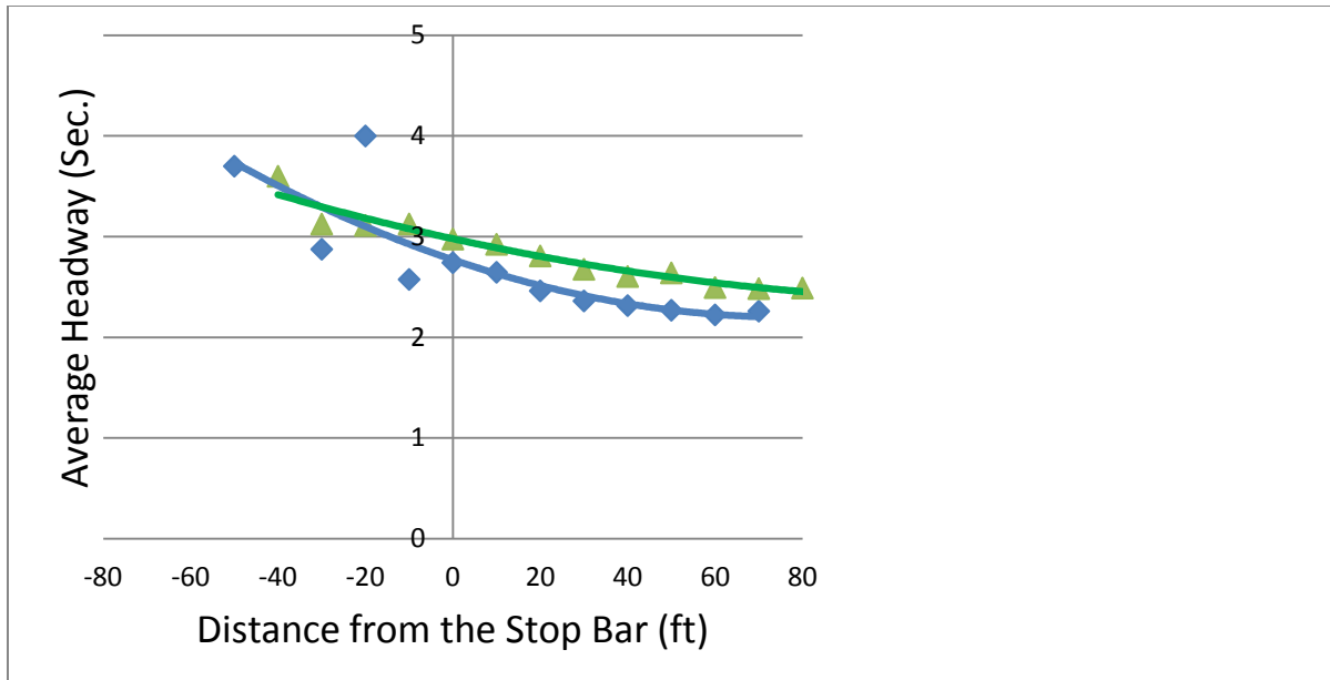
Figure 16: Average time headway versus distance from the stop bar (queue position 4).
