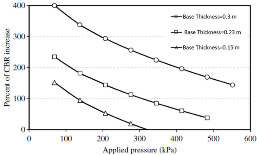
Figure 2.6 Percent increase of equivalent subgrade CBR due to the addition of aggregate layer for different aggregate thicknesses (adapted from Sun et al., 2018).
