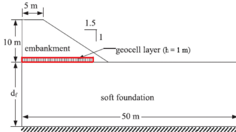
Figure 2.24 Embankment model used for parametric analysis (adapted from Madhavi Latha & Rajagopal, 2007).
