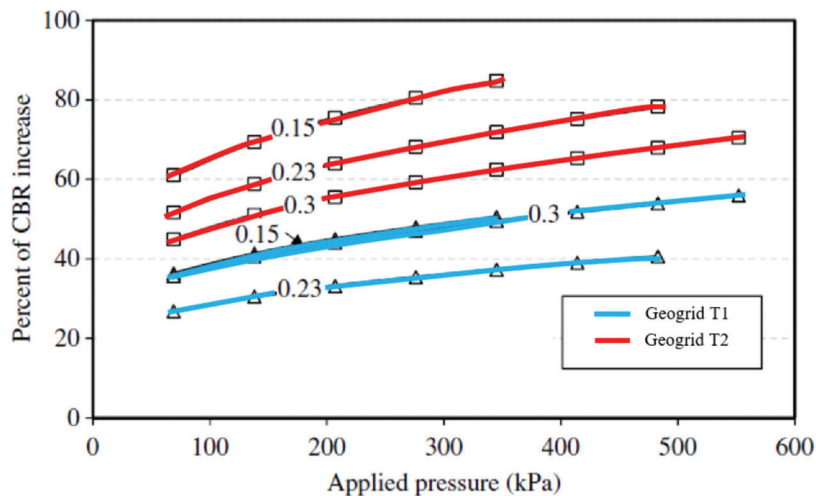
Figure 2.7 Percent increase of equivalent subgrade CBR due to the addition of a geogrid for different aggregate thicknesses (adapted from Sun et al., 2018).
