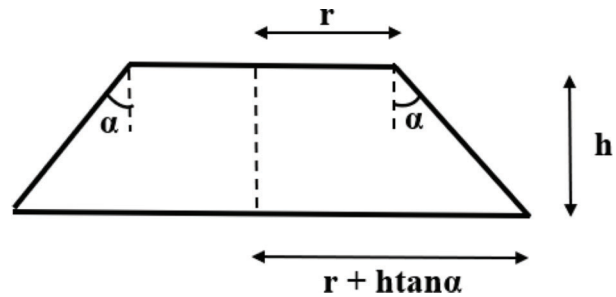
Figure 2.20 Vertical stress dispersion effect in the base course layer.
