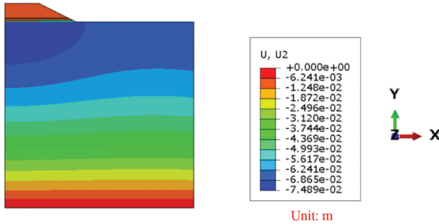
Figure 4.5 Vertical displacement contours for the unreinforced model with W.Z. = 0 .
