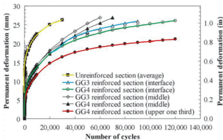
Figure 2.2 Surface permanent deformation of the pavement for different types and locations of geogrids (adapted from Abu-Farsakh & Chen, 2011).
