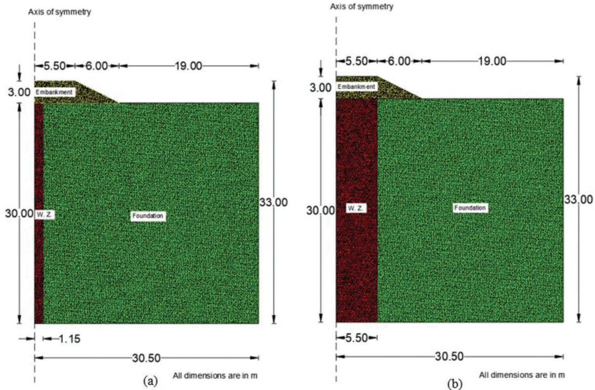
Figure 4.7 Cross-section of the unreinforced embankment model with (a) W.Z. = 0.1 B and (b) W.Z. = 0.48 B .
