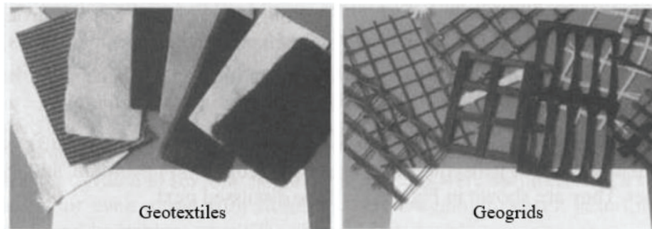
Figure 2.1 Geotextiles and geogrids (adapted from Koerner, 2005).
