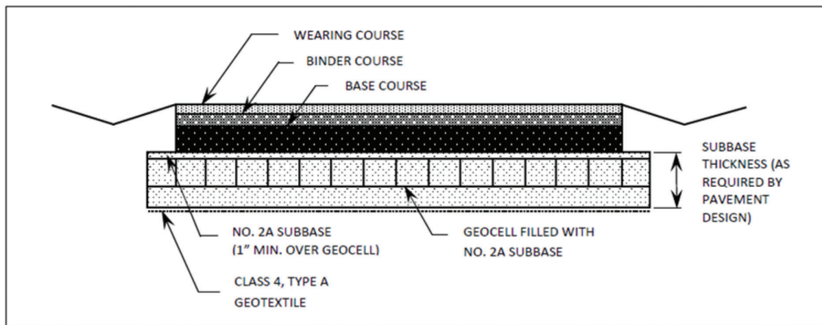
Figure 2.26 Typical pavement section with geocell layer (adapted from PennDOT, 2018).
