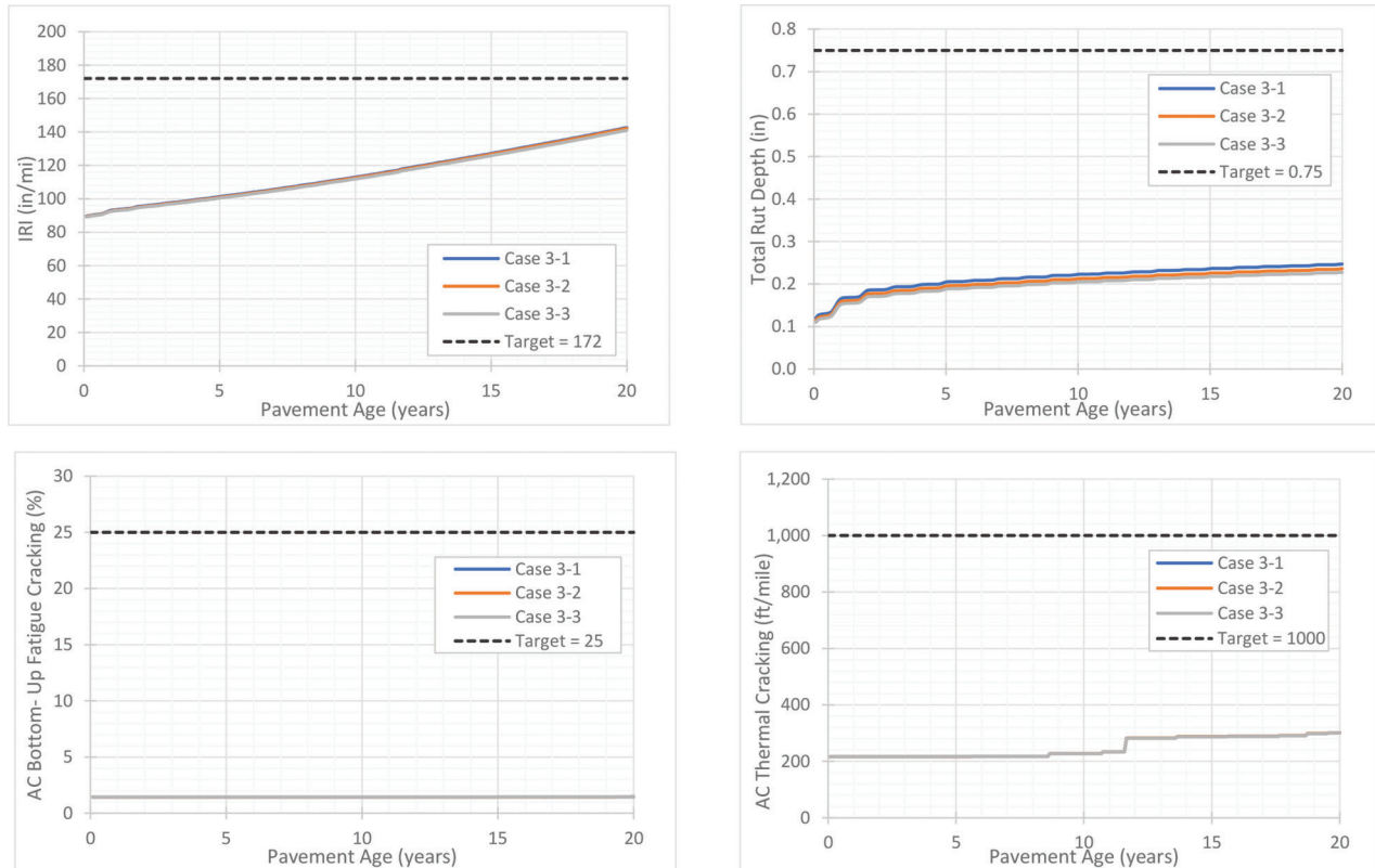
Figure 3.7 Development of IRI, rut depth, AC bottom-up cracking, and AC thermal cracking with pavement age (Cases 3-1 to 3-3).
