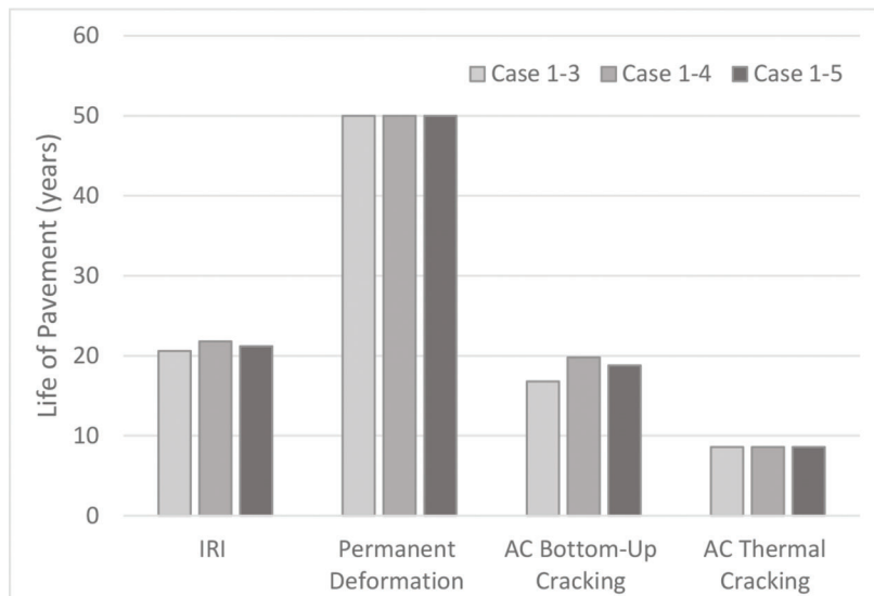
Figure 3.4 Pavement life for each distress category (Cases 1-3 to 1-5).
