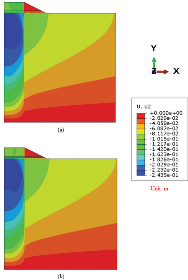
Figure 4.14 Vertical displacement contours for (a) unreinforced and (b) reinforced models with two geogrids ( E = 400 MPa) (noncentral W.Z. = 0.3 B, E_{w.z.} = 7 MPa).
