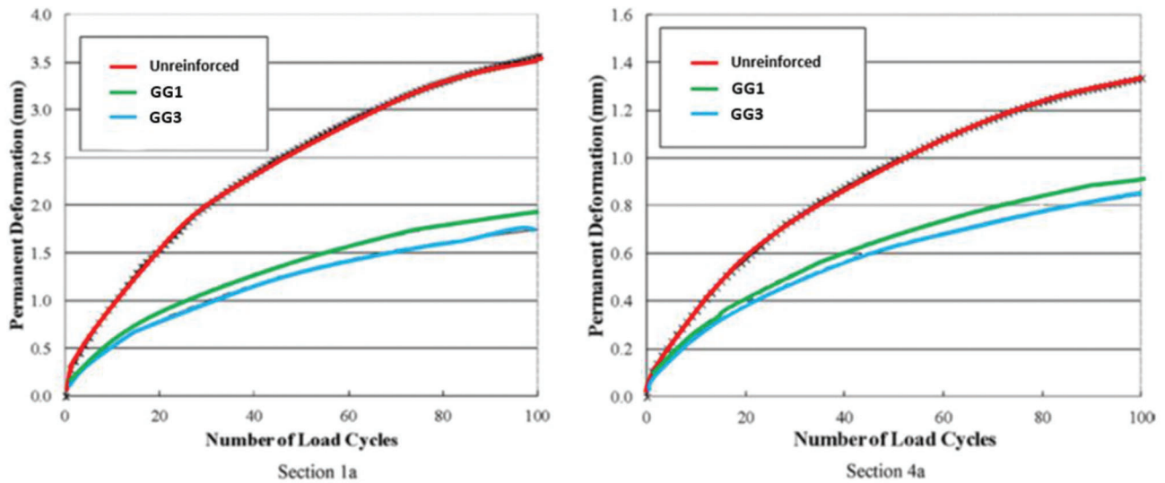
Figure 2.3 Development of permanent deformation for different pavement sections (geogrid placed at the interface between subgrade and base course)–Sections 1a and 4a (adapted from Abu-Farsakh et al., 2014).
