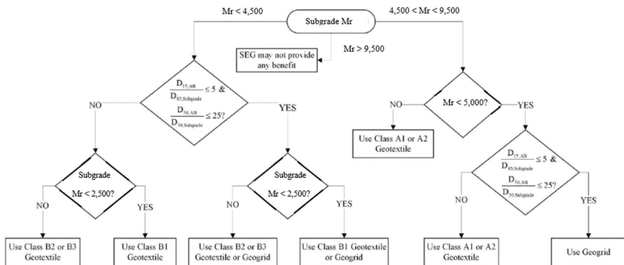
Figure 2.25 Flowchart for the selection of SEG, Subgrade Enhancement Geosynthetic ( M_r is the resilient modulus) (adapted from Caltrans, 2020).
