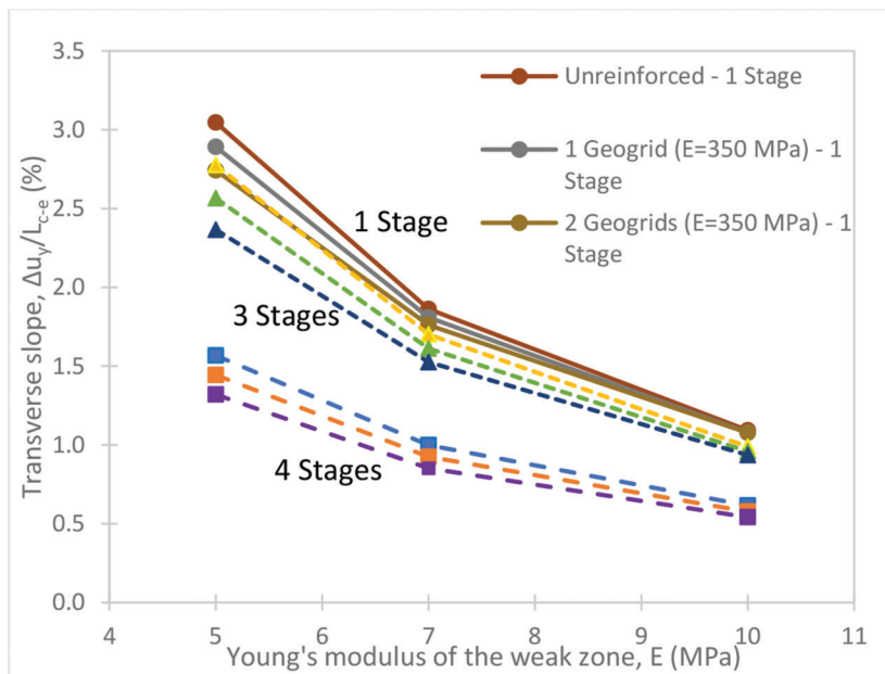
Figure 4.12 Dependence of transverse slope on the Young's modulus of the weak zone for the unreinforced and reinforced models with W.Z. = 0.3 B (embankment construction in 1, 3, and 4 stages).
