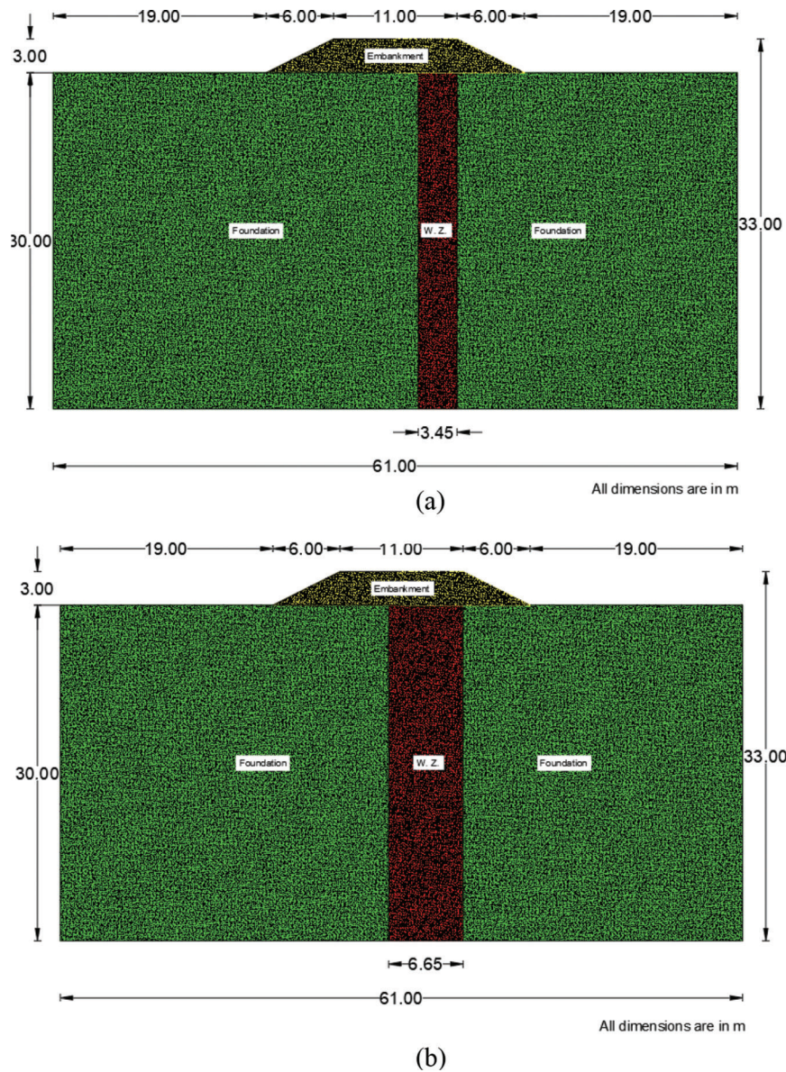
Figure 4.15 Cross-section of the unreinforced embankment model with (a) W.Z. = 0.15 B and (b) W.Z. = 0.29 B.
