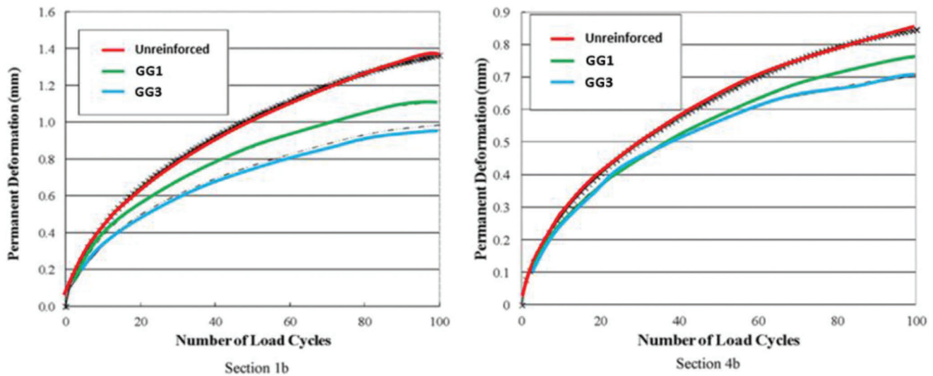
Figure 2.4 Development of permanent deformation for different pavement sections (geogrid placed at the interface between subgrade and base course)–Sections 1b and 4b (adapted from Abu-Farsakh et al., 2014).
