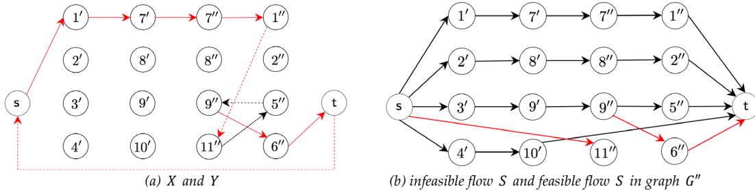
Figure 5: Cycle X , subsequence Y , graph G''=(V,S) , and the final flow S_m
