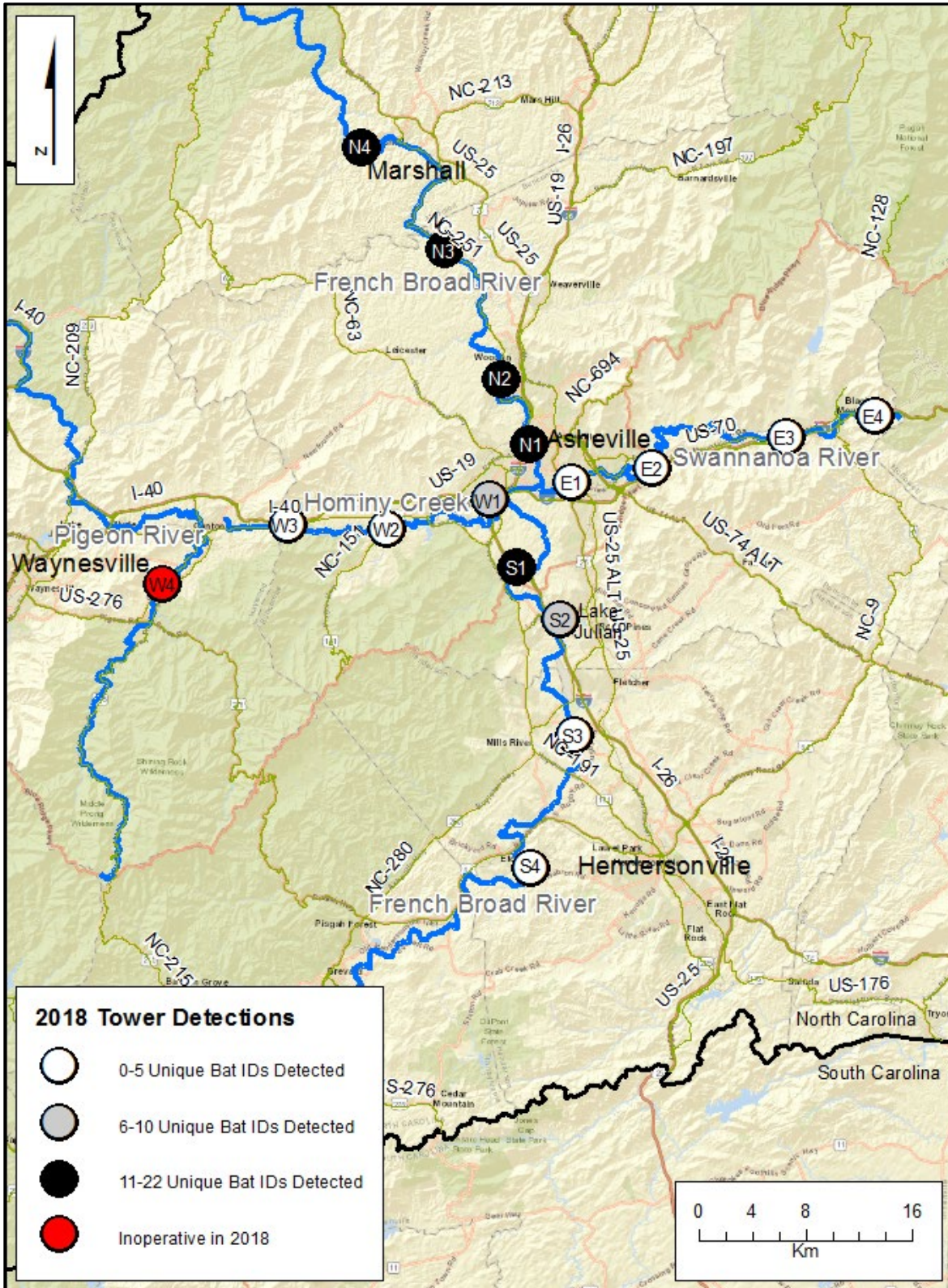
Figure 19. Locations of 16 radio-telemetry towers used to detect foraging gray bats in the French Broad River Basin of western North Carolina in 2018. The towers are distinguished by the number of unique individual radio-tagged bats detected during the period, April– October 2018.
