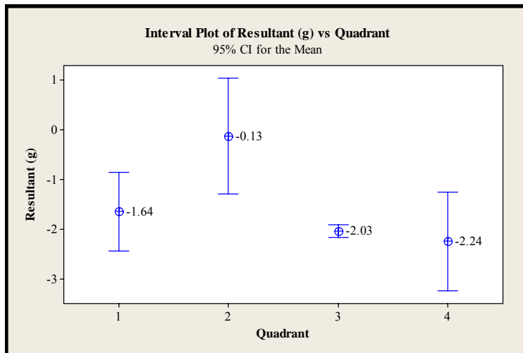
Figure 24. Interval Plot of Resultant in g's at Quadrant Locations
