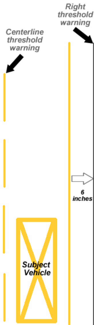
Figure 20. Diagram of Warning Threshold Locations
