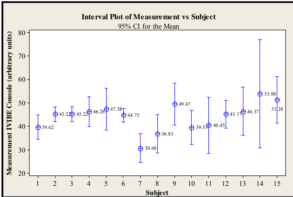
Figure 25. Interval plot of IVIBE® Haptic Seat Measurement
