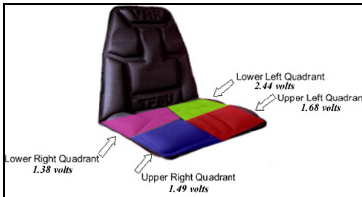
Figure 23. Vibration Intensity Measurements at Seat Quadrant Locations
