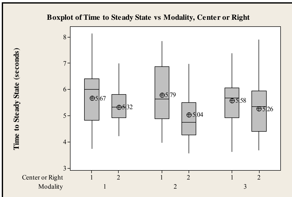
Figure 38. Time to Steady State (sec)
