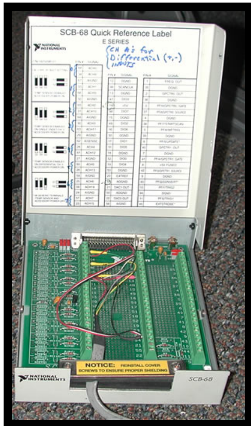
Figure 9. National Instruments SCB-68 Connector Block
