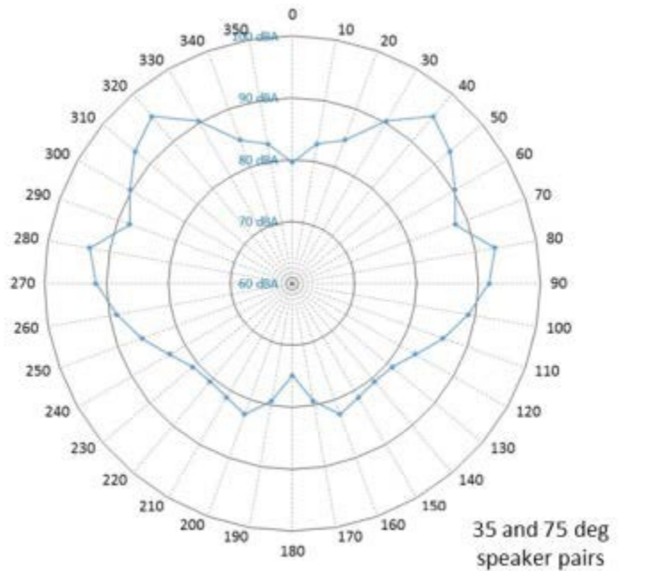
Figure 38. Combined Directivity Pattern of AWD \pm 35 and \pm 75 Degree Loudspeakers at 100 Feet from Locomotive
