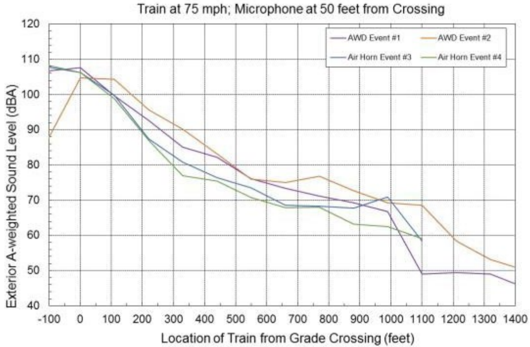
Figure 52. Exterior Sound Level at Grade Crossing 50 Feet from Track with Train at 75 mph for Comparably Scaled Systems
