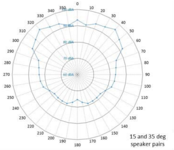
Figure 37. Combined Directivity Pattern of AWD \pm 15 and \pm 35 Degree Loudspeakers at 100 Feet from Locomotive
