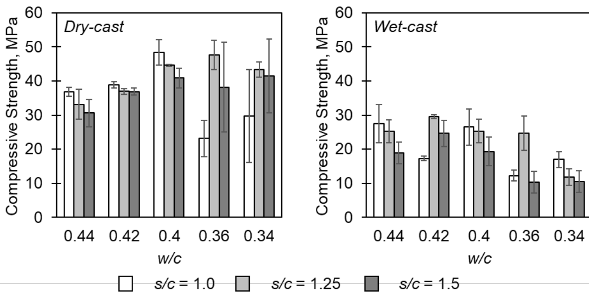
Figure 10: Comparison of 3-hour compressive strengths of mortar cubes
