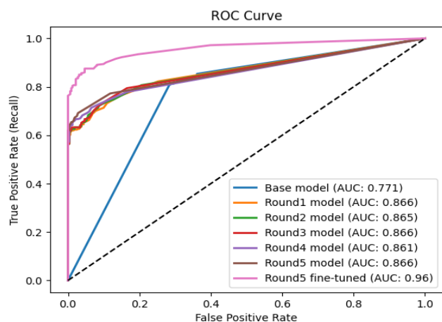
Figure 6. ROC Curve of Guardrail Models through AL
