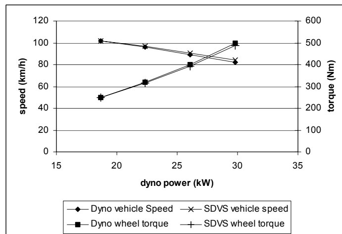
Figure 10 Test 1: Comparison of SDV with vehicle data collected on a dynamometer.
