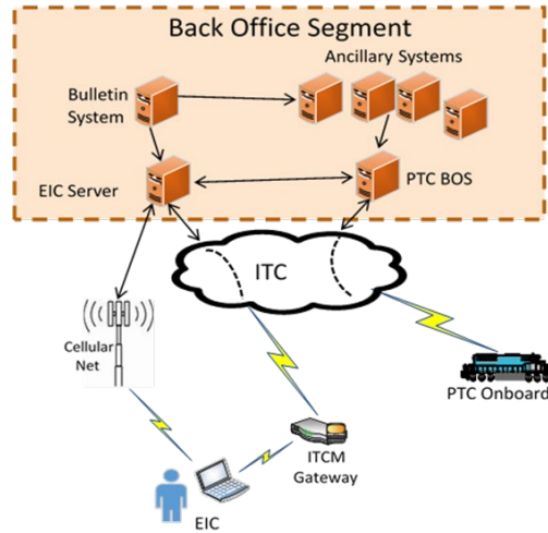
Figure 2 illustrates how an EIC uses the EIC-PRT system to provide instructions to a PTC-equipped train as it approaches a WZ. Note that, as illustrated, the EIC-PRT is an overlay to existing operating practices; thus, voice communication between an EIC and a train crew is maintained.
