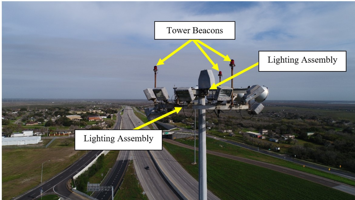
Figure 3. Inspection of the lighting assembly and pulley system from south of the high mast tower before the pulley operation
