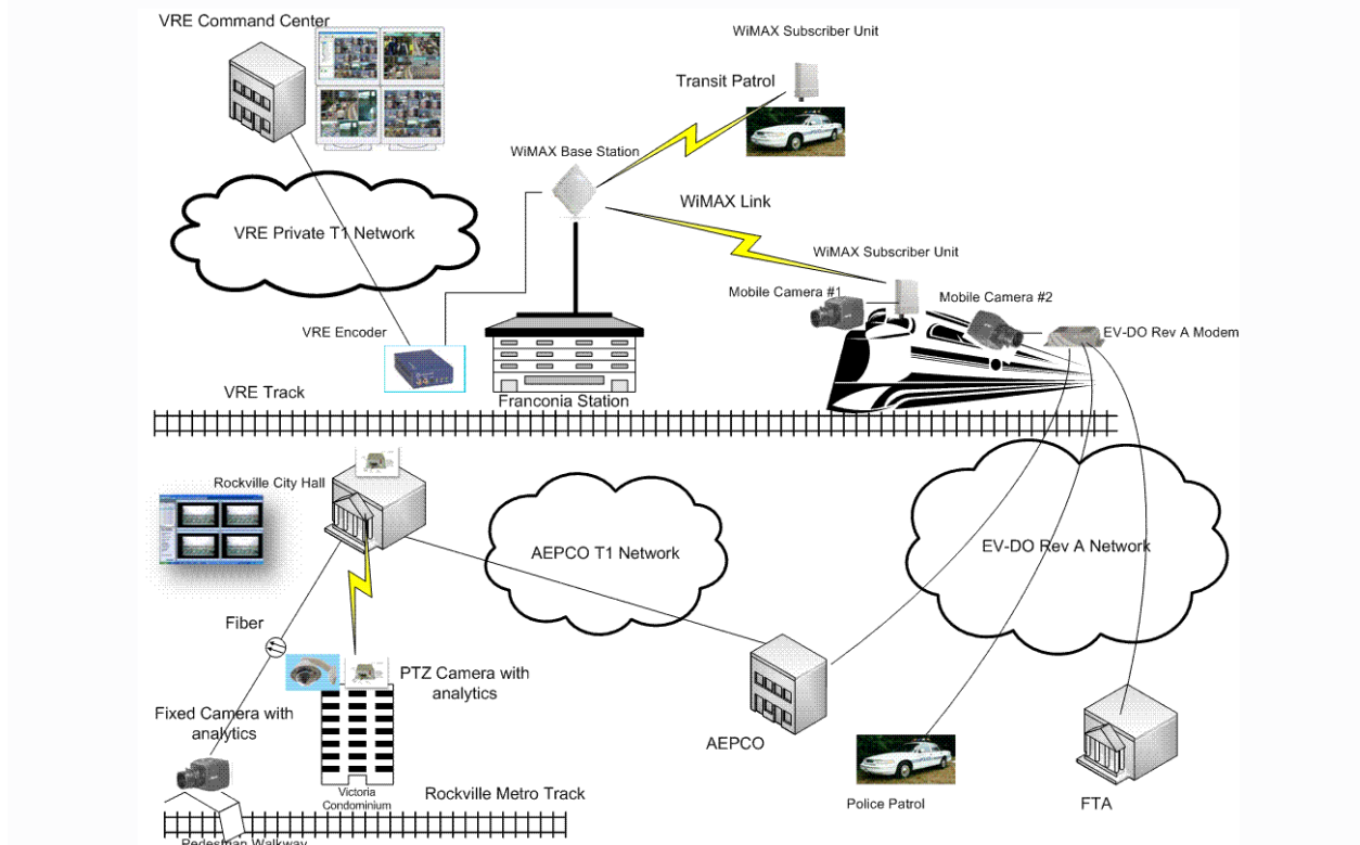
Figure 4: Final SharpRAIL Architecture
