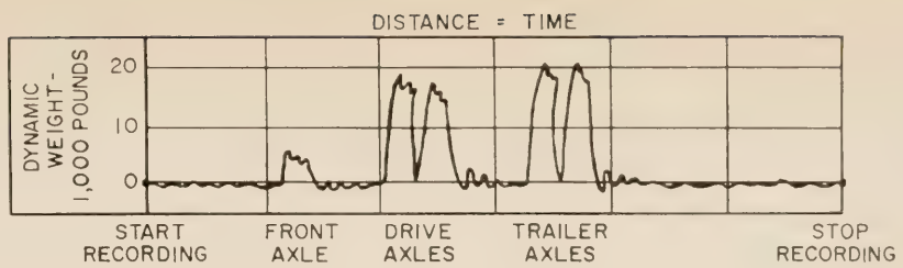
TYPICAL OSCILLOGRAPH RECORDING (5-AXLE TRUCK - TRAILER)
