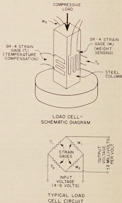
Figure 1.—The strain gage load cell.
