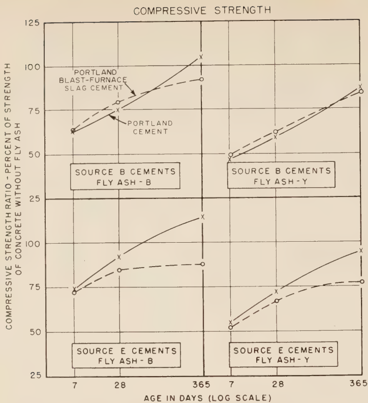
Figure 1.—Effect of replacement of one-third of portland or portland blast-furnace slag cement by fly ash on strength of concrete.
