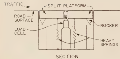
Figure 4.—“Broken bridge” scale.
