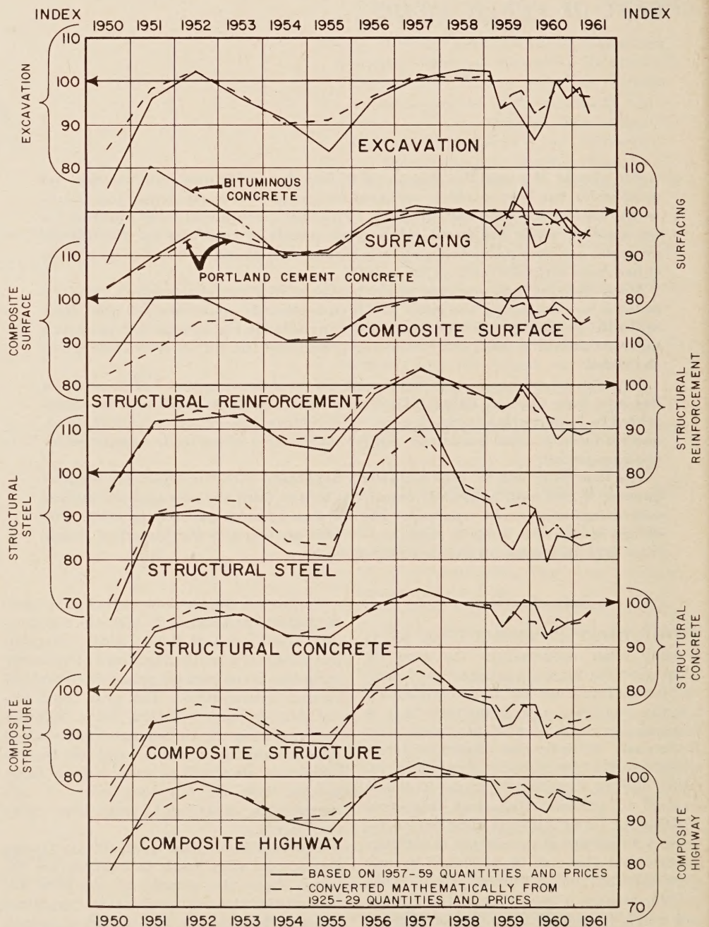
Figure 1.—Comparison of trends of the original and new bid price indexes, 1950 to date.
