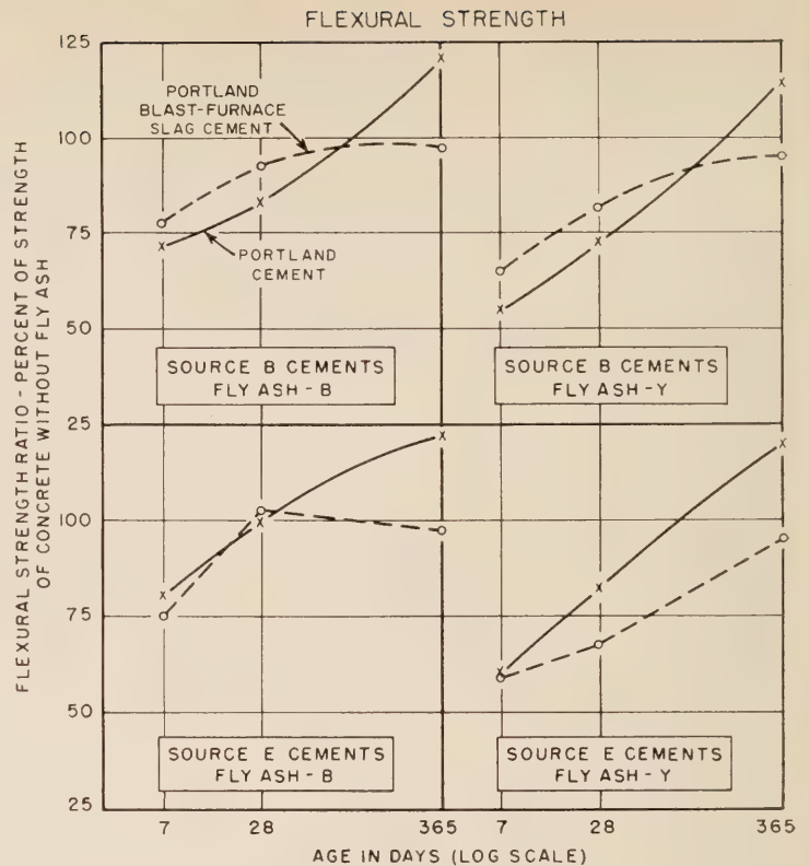
Figure 1.—Effect of replacement of one-third of portland or portland blast-furnace slag cement by fly ash on strength of concrete.
