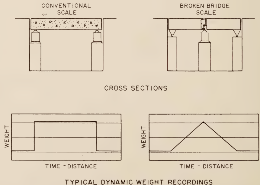
Figure 5.—Comparison of conventional and broken bridge scale dynamic weight recordings.
