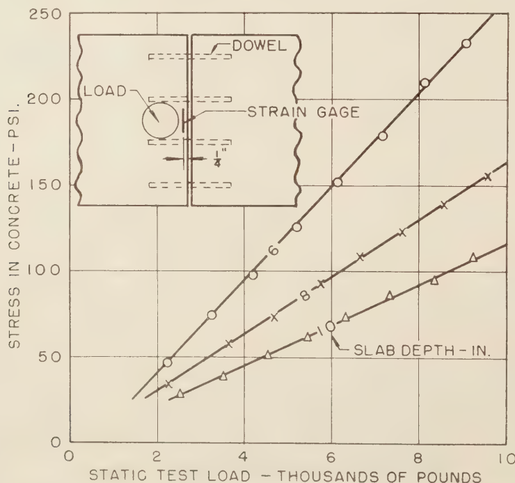
Figure 44.—Typical relations between applied load and stress in concrete along the joint edge. (Each value is the average of 10 observations.)
