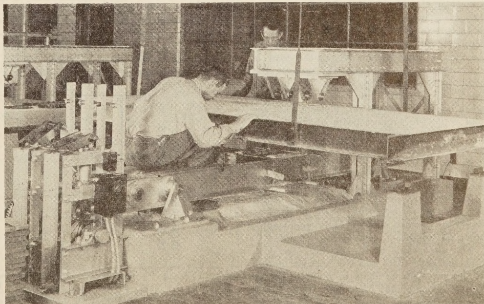
Figure 4.—Lowering a cured specimen into the testing machine in the channel frame in which it was cast; the loading levers have been removed for this operation.
