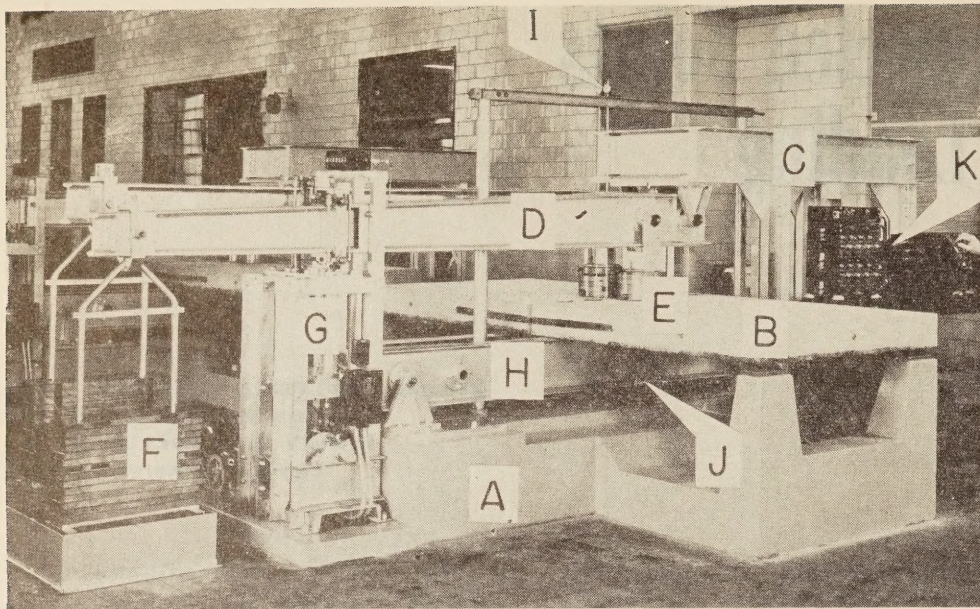
Figure 1.—Testing machine (A, reinforced concrete base; B, test specimen; C, structural steel frame; D, loading lever; E, loading pad; F, adjustable load of lead weights; G, cam and lift-rod mechanism; H, specimen support beam; I, micrometer dials; J, SR-4 strain gages; and K, oscillograph recording equipment).
