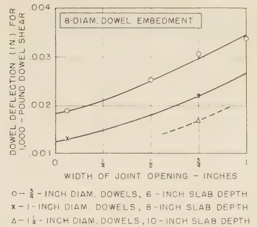
Figure 14.—Relations between width of joint opening and dowel deflection.
