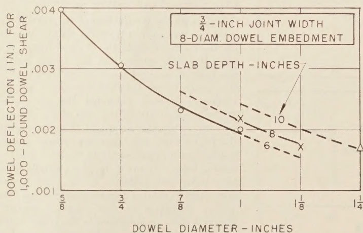
Figure 11.—Relations between dowel diameter and dowel deflection.
