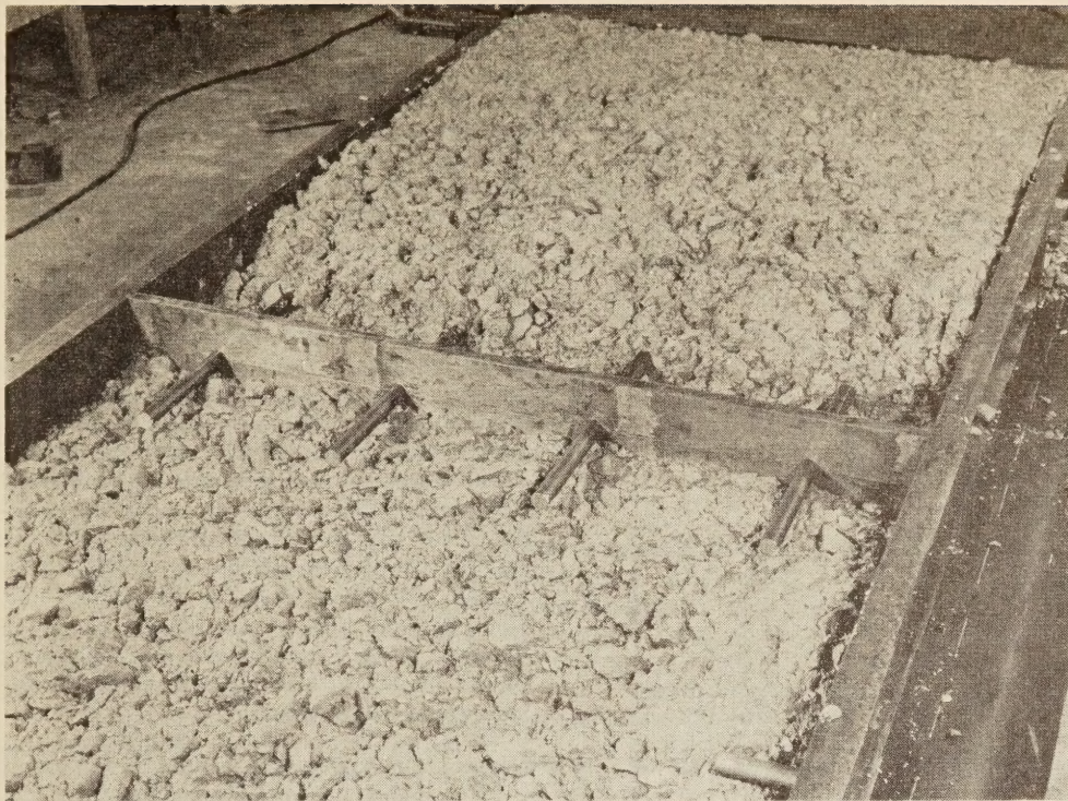
Figure 3.—Appearance of concrete during fabrication of a specimen; fluidity was obtained with internal vibrators.
