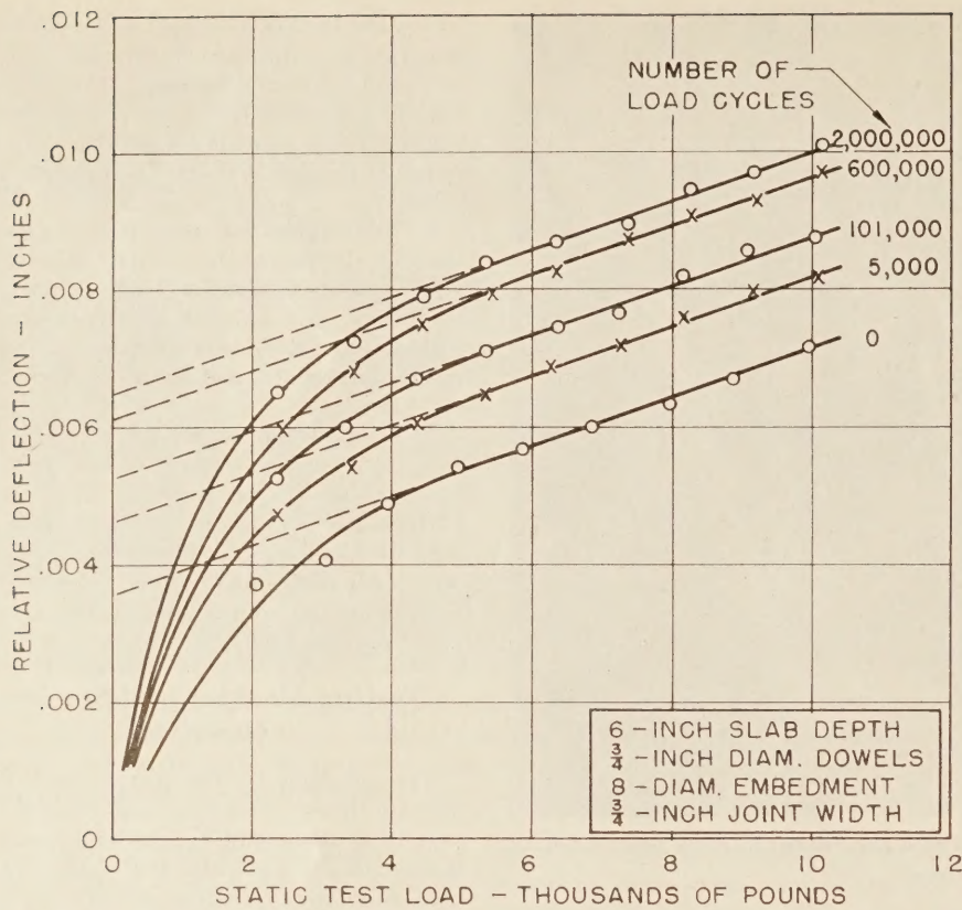
Figure 5.—Relation between applied load and relative deflection, after various numbers of load cycles.
