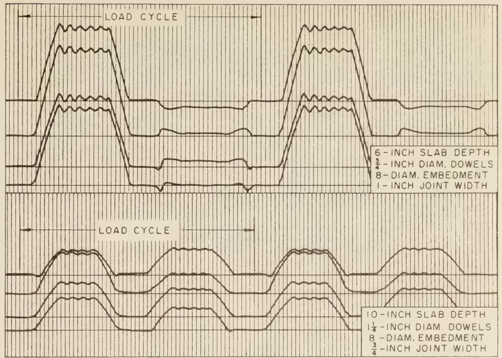
Figure 41.—Oscillograms of strain in individual dowels for a 10,000-pound load.
