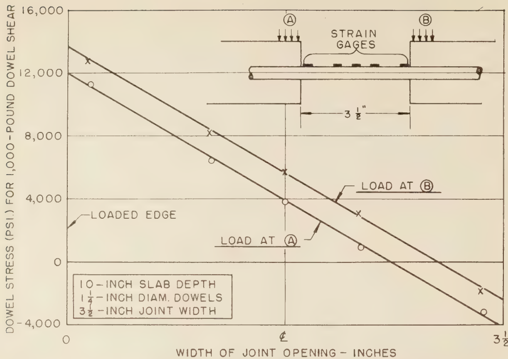
Figure 47.—Distribution of dowel stresses within the width of a 3\frac{1}{2} -inch joint opening.
