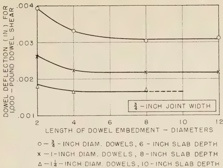
Figure 13.—Relations between length of dowel embedment and dowel deflection.
