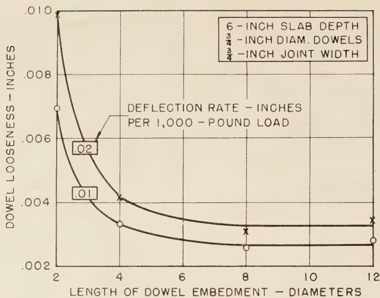
Figure 30.—Comparison of dowel looseness developed at 0.01- and 0.02-inch free joint-edge deflection rates after 600,000 cycles of a 10,000-pound load.
