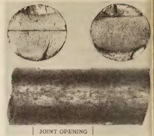
Figure 48.—Fatigue failure of a \frac{3}{4} -inch diameter dowel. The cross-section views at the top correspond to the left and right ends of the fractured dowel.
