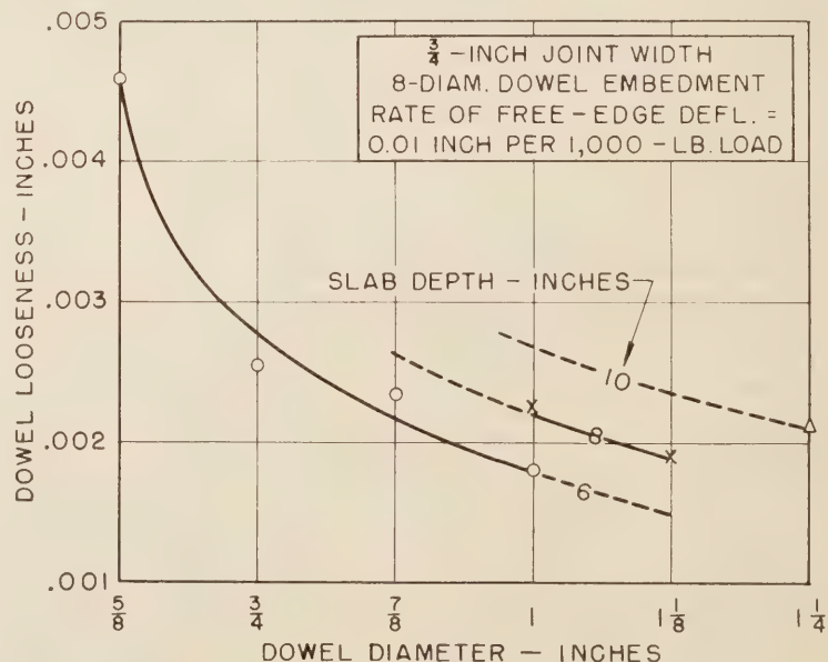
Figure 27.—Relations between dowel diameter and dowel looseness resulting from 600,000 cycles of a 10,000-pound load (base measurements obtained at first cycle).
