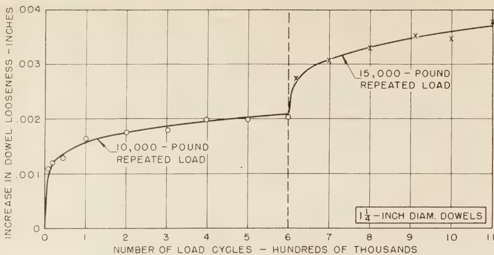
Figure 26.—Effect of increasing the magnitude of the repeated load on the development of dowel looseness.
