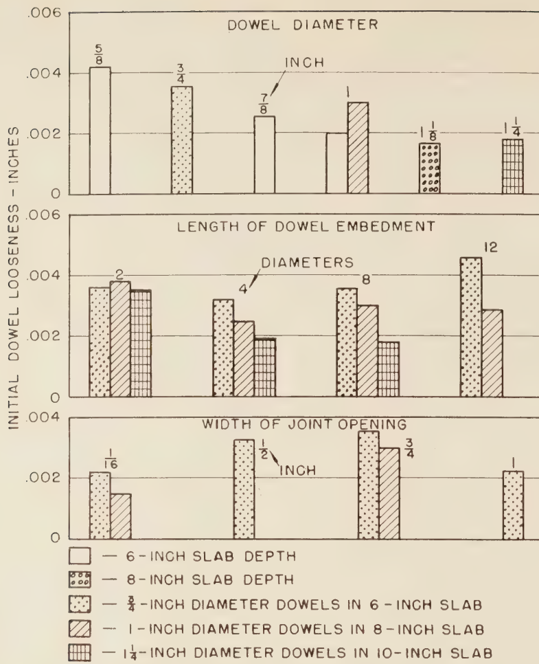
Figure 22.—Data on initial dowel looseness.
