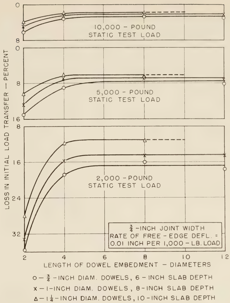
Figure 32.—Relations between length of dowel embedment and loss in initial capacity to transfer load resulting from 600,000 cycles of a 10,000-pound load (base measurements obtained at first cycle).
