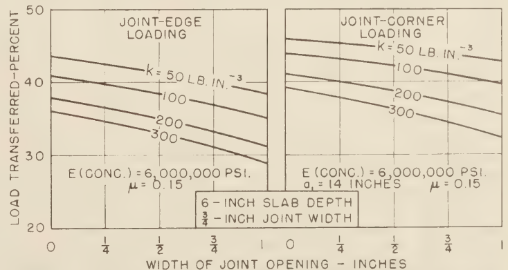
Figure 16.—Effect of width of joint opening on load transfer in the case of a single dowel.
