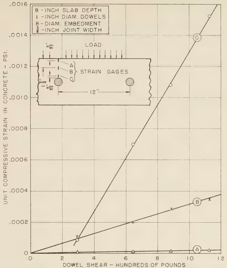
Figure 45.—Dowel shear-concrete strain relations for the indicated points (A, B, and C) at the face of the loaded joint edge. (Each value is the average of 10 observations.)
