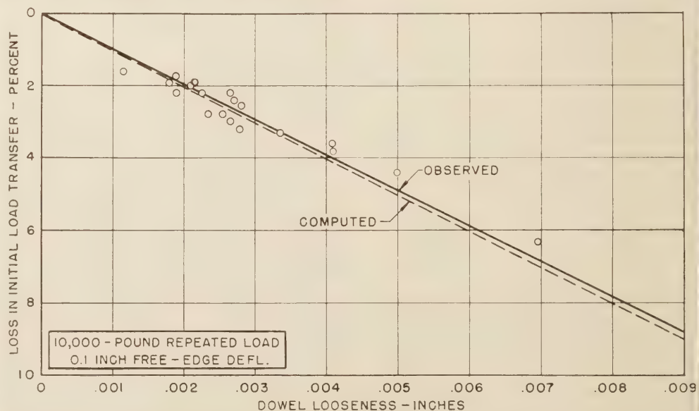
Figure 34.—Relation between dowel looseness and loss in initial capacity to transfer load after 600,000 cycles of a 10,000-pound load.
