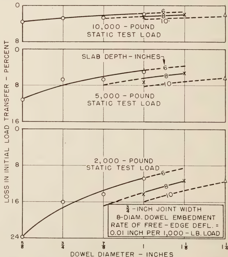
Figure 31.—Relations between dowel diameter and loss in initial capacity to transfer load resulting from 600,000 cycles of a 10,000-pound load (base measurements obtained at first cycle).
