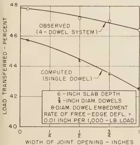
Figure 20.—Observed percentages of load transfer of 4-dowel system compared with computed values of a single dowel for a range in widths of joint opening.
