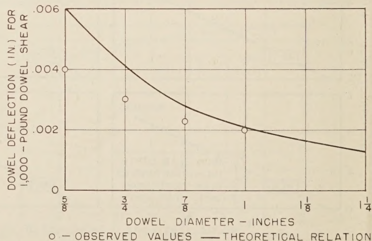
Figure 12.—Comparison of theoretical and observed relations between dowel diameter and dowel deflection.
