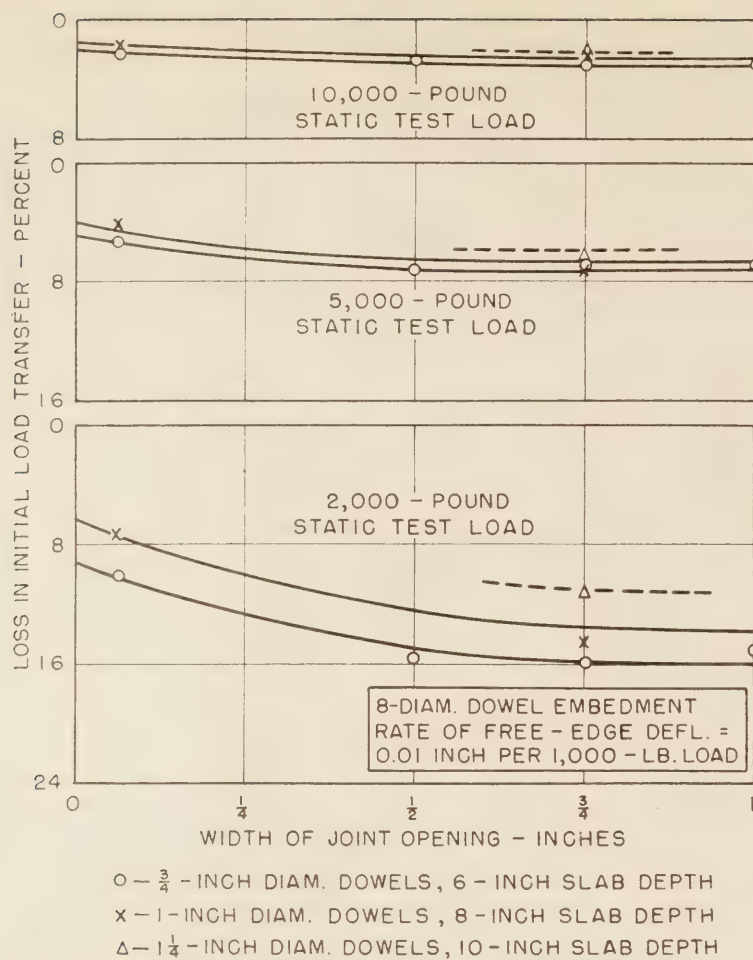
Figure 33.—Relations between width of joint opening and loss in initial capacity to transfer load resulting from 600,000 cycles of a 10,000-pound load (base measurements obtained at first cycle).
