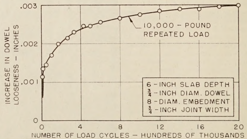
Figure 6.—Effect of repetitive loading on the development of dowel looseness.
