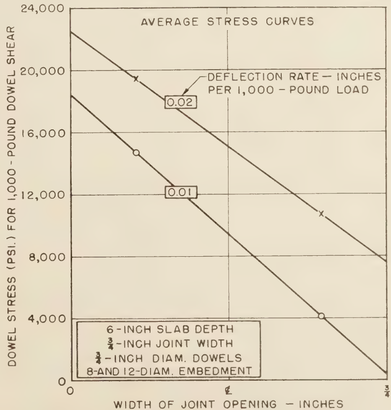
Figure 42.—Effect of deflection rate on dowel stress.
