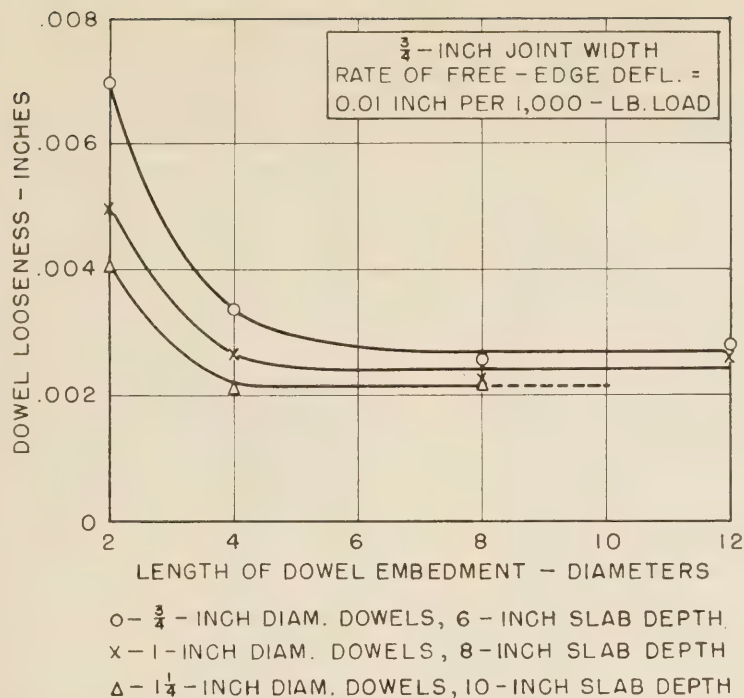
Figure 28.—Relations between length of dowel embedment and dowel looseness resulting from 600,000 cycles of a 10,000-pound load (base measurements obtained at first cycle).
