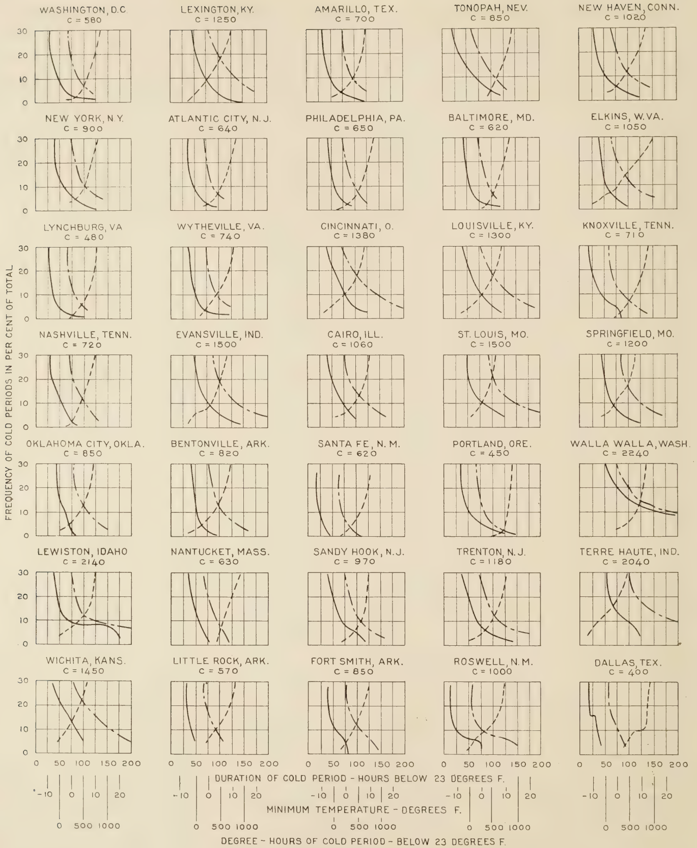
DURATION - FREQUENCY ——— MINIMUM TEMPERATURE FREQUENCY - - - - - DEGREE - HOUR FREQUENCY - - - - - FIGURE 7.—DURATION-FREQUENCY CURVES, MINIMUM TEMPERATURE-FREQUENCY CURVES, AND DEGREE-HOUR-FREQUENCY CURVES FOR 35 SELECTED WEATHER BUREAU STATIONS
