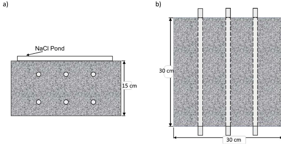
Figure 3.18: Schematic illustration of stainless steel-reinforced concrete specimen obtained from FAU: a) side view, b) top view.
