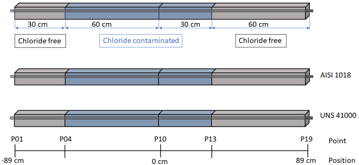
Figure 3.3: Longitudinal profile for UNSS41000SS/ AISI1018CS specimens in concrete. “0 cm” represents the central point of the specimens, representing the longitudinal midpoint position. Spatial distribution of two types of concrete is shown as well.
