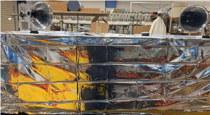
Figure 3.31: Experimental set-up of locally-deficient specimens in enclosed glass container covered in reflective wrap and heat lamps on top, (a) front view and (b) top view.
