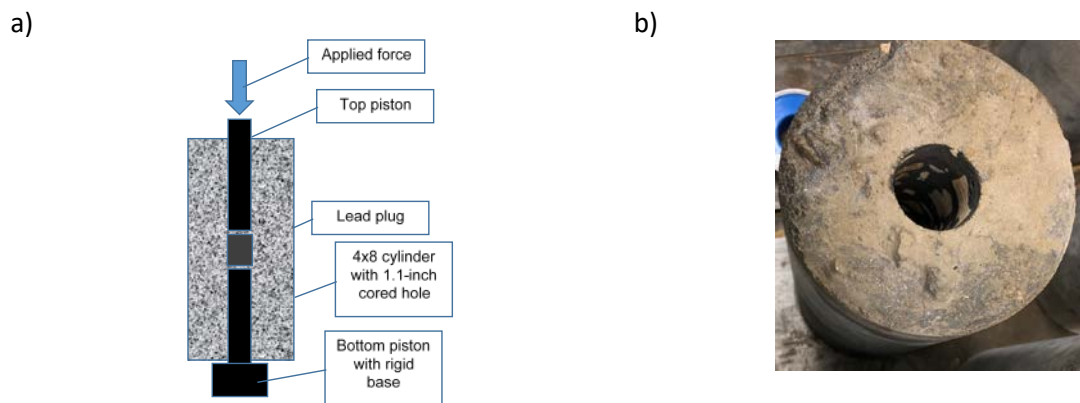
Figure 4.5: 4 x 8-inch concrete cylinder with 1.1-inch core hole.
