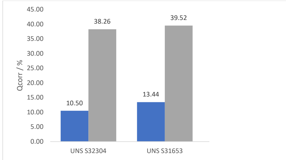
Figure 4.14: Comparison of corrosion degree to reach the IS limit state for the indicated percentage strength loss criteria. Each color illustrates a case of insufficient strength, in which blue represents ~21% strength loss and gray represents ~66% strength loss.
