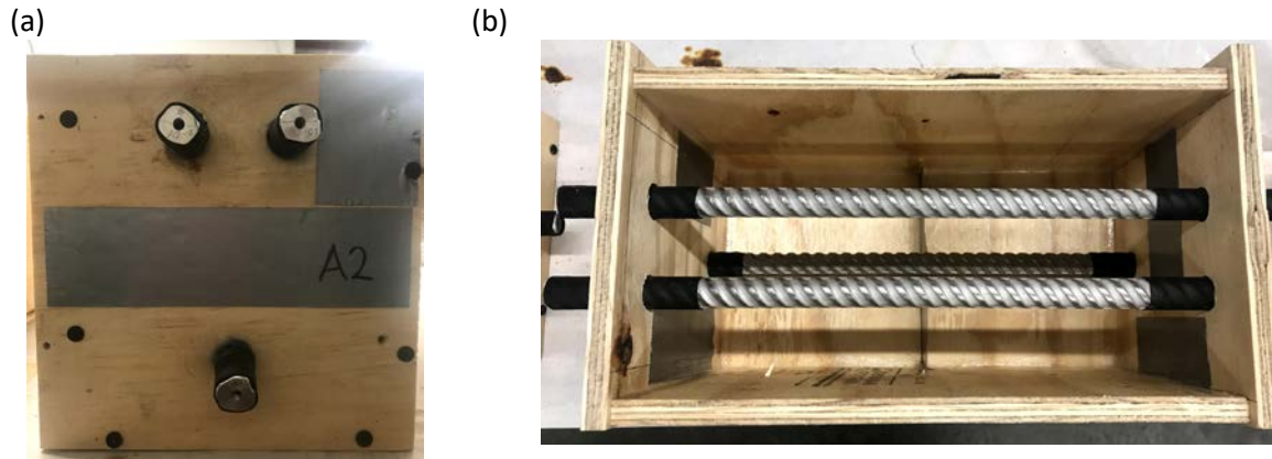
Figure 3.25: Steel placement in wood form prior to casting (a) front view of mold. Stainless steel reinforcement was tapped and drilled, and (b) top view of mold. Stainless-steel shim was placed parallel to the rebar.
