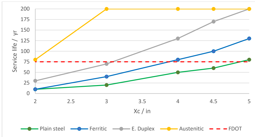
Figure 6.3: First scenario: life cycle analysis under moderately aggressive conditions as a function of concrete cover for each type of steel.
