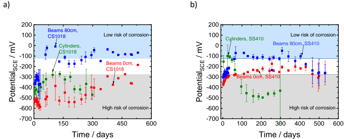
Figure 5.2: HCP results of specimens as a function of time considering different locations (i.e. end and center) in simulated beams compared to those of the cylindrical specimens reinforced with (a) carbon steel and (b) stainless steel.
