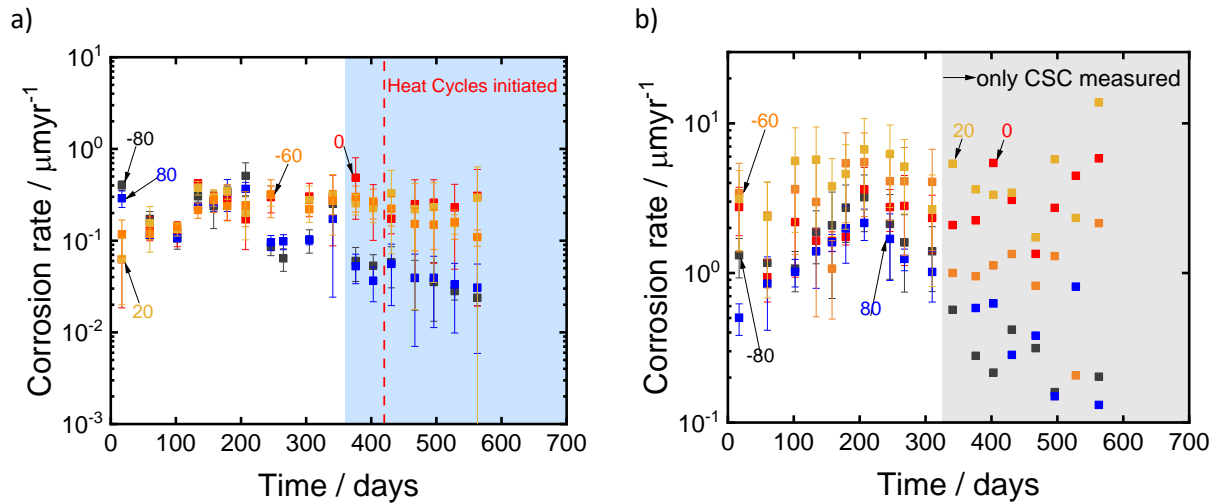
Figure 4.3: Behavior of the corrosion rate over time in (a) stainless steel (SS01, SS02, and SS03), and (b) carbon steel (CSA, CSB and CSC) specimens. Each data point represents the average value for the three specimens and the error bars the standard deviation. Black, orange, red, yellow and blue represented data points at locations -80 cm, -60 cm, 0 cm, 20 cm and 80 cm, respectively. Dashed line indicates initiation of elevated temperature exposure. Blue-shaded region designates the point at which low frequency limit of the impedance was extended to 1 mHz for points -80 cm and 80 cm. The number pointing to each series represents the position along the beam as described by number line shown in Figure 3.3.
