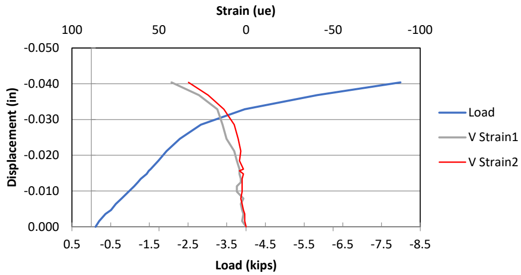
Figure 4.8: Vertical strain.
