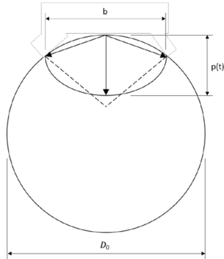
Figure 4.12: Schematic illustration of cross-sectional loss of rebar subjected to pitting corrosion. 66
