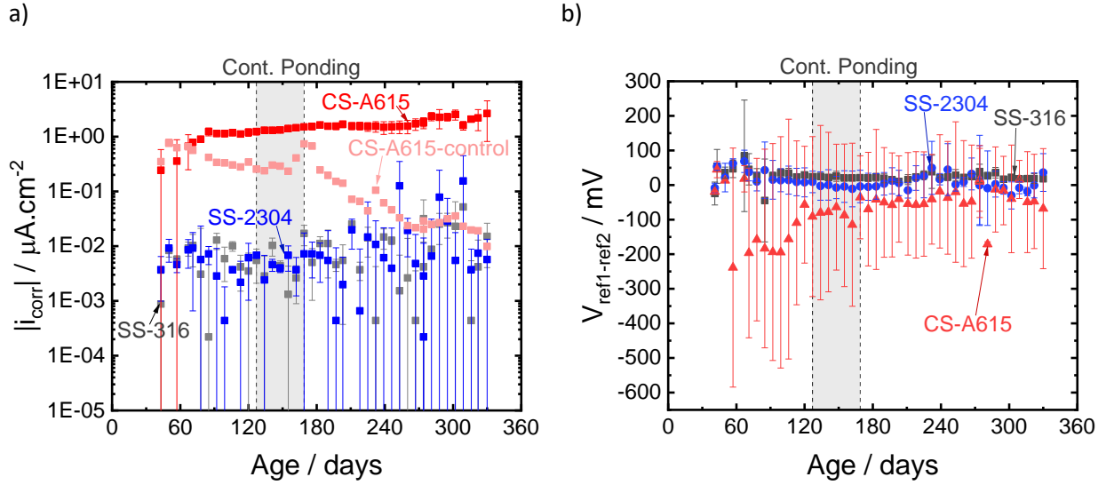
Figure 4.16: Preliminary results of specimens with concrete deficiencies (a) macrocell current density and (b) potential difference between defective and sound concrete region.
