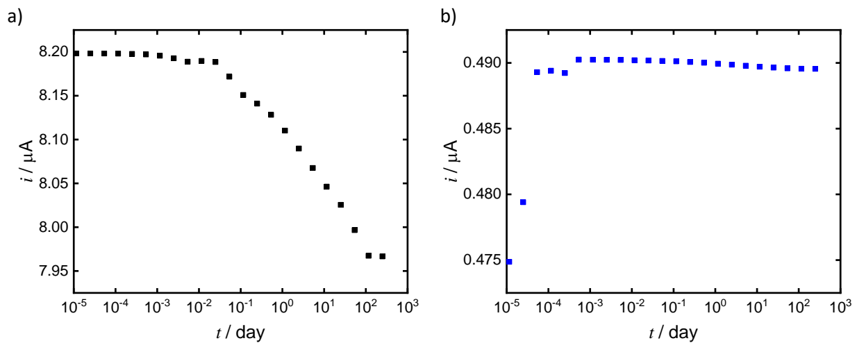
Figure 4.19. Macrocell corrosion rates as a function of time in cracked concrete: (a) CS and (b) SS.
