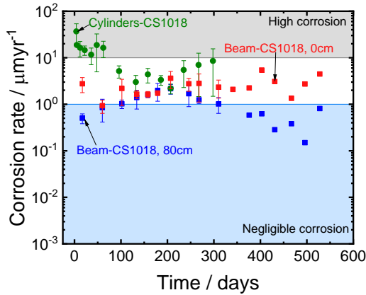
Figure 4.4: Corrosion rate as a function of time at different locations (i.e. end and center) of beams compared to cylindrical specimens reinforced with (a) SS and (b) CS.
