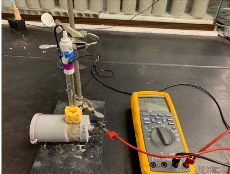
Figure 3.15: Half-cell potential titanium vs. SCE reference electrode measurement on specimen SS410-III. Multimeter, titanium electrode, reference electrode (SCE), and electrical junction device (yellow sponge).
