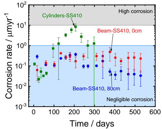
Figure 4.4: Corrosion rate as a function of time at different locations (i.e. end and center) of beams compared to cylindrical specimens reinforced with (a) SS and (b) CS.
