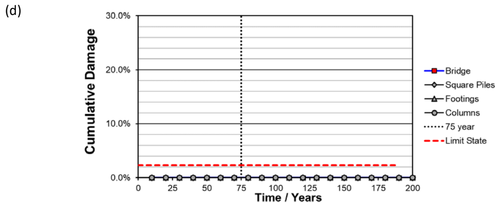
Figure 6.2 (continued): Second scenario (extremely aggressive): life cycle analysis under moderately aggressive conditions for (a) Plain steel, (b) Ferritic SS, (c) E. Duplex SS and (d) Austenitic SS.
