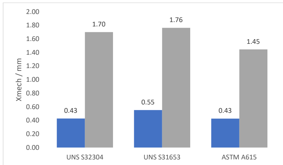
Figure 4.15: Comparison of corrosion penetration X_{mech_{IS}} required to reach the IS limit state for the indicated percentage strength loss criteria. In the onset of brittleness case, a threshold corrosion degree value 8.6% 81 was selected given that it was the most critical and the only experimental value obtained for stainless steel. In this scenario, X_{mech_{OB}} was estimated to be 350 \mu m . The X_{mech_{IS}} and X_{mech_{OB}} values are summarized in Table 4.10.
