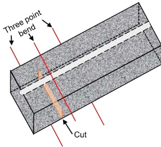
Figure 3.23: Schematic illustration of a) cross-sectional cut and b) three point bend-cross section.
