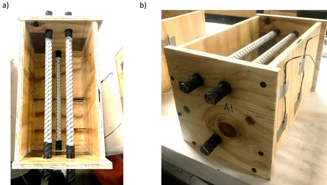
Figure 3.24: Final setup of specimens before casting. Wood mold was coated with a mold release agent, titanium reference electrodes and steel rebars were in place. (a) Top view, and (b) side view.
