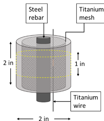
Figure 3.14: Schematic of cylindrical specimen showing the electrode configuration and a region shaded in yellow representing an opening where air flow was allowed (bounded by dashed yellow lines).
