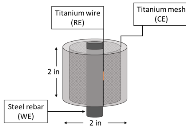
Figure 3.16: Schematic illustration of EIS measurement experimental setup of cylindrical specimen.
