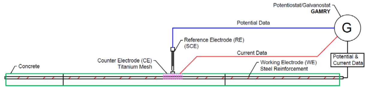
Figure 3.9: Schematic illustration of EIS measurement experimental setup.
