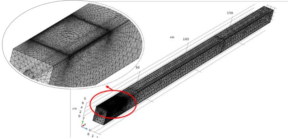
Figure 3.12: Finite-element mesh of the 3D model. Close-ups show the variation on the size in zone of high potential variation.
