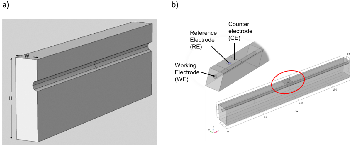
Figure 5.4: Schematic illustration of (a) HCP and (b) EIS Finite Element Model simulations.
