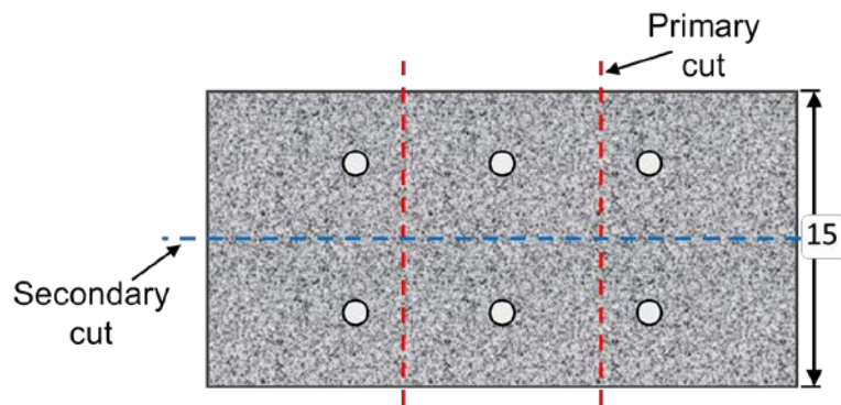
Figure 3.20: Schematic illustration of saw cuts performed in step 2 (red) and step 3 (blue).
