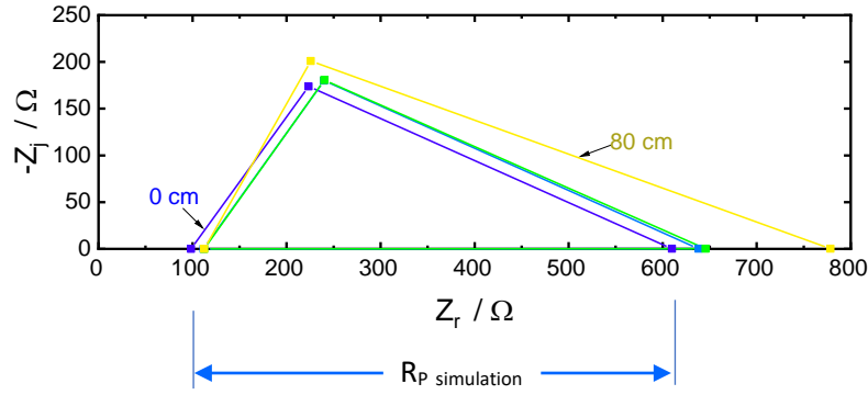
Figure 3.13: Nyquist plot from finite element model.
