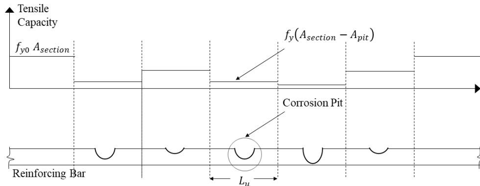
Figure 4.13: Spatial tensile capacity of non-uniformly corroding reinforcement bar.
