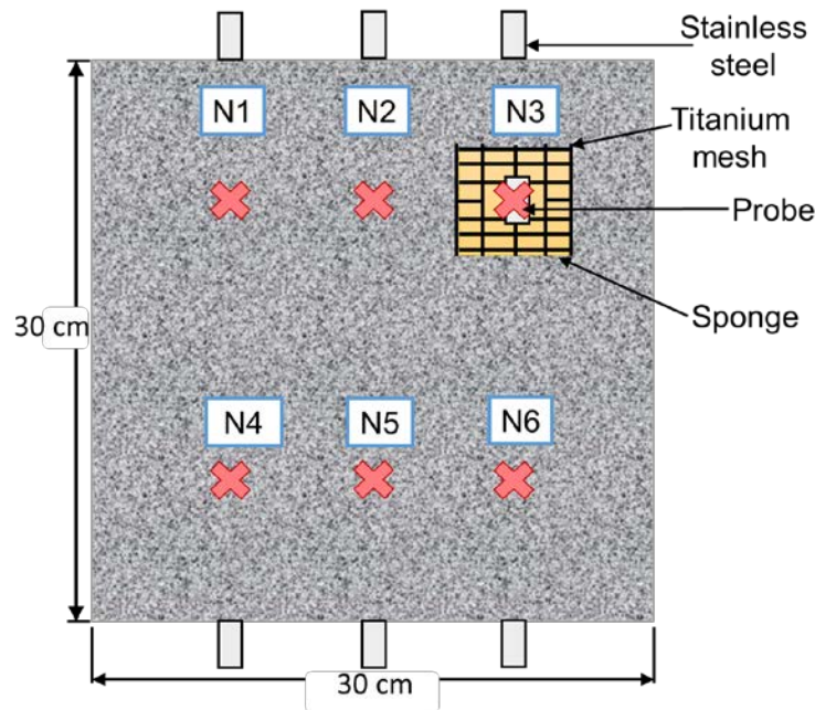
Figure 3.19: Schematic illustration of EIS experimental set-up of legacy specimen.
