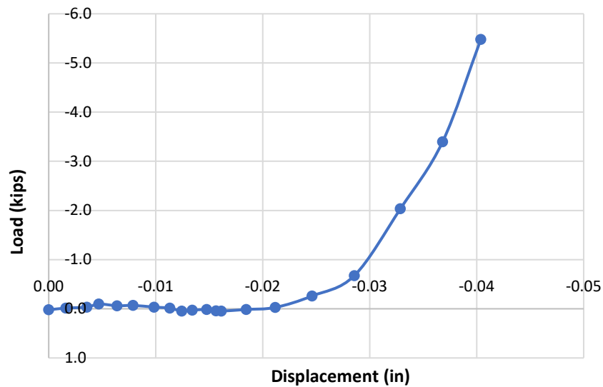
Figure 4.11: Concrete load vs. displacement.
