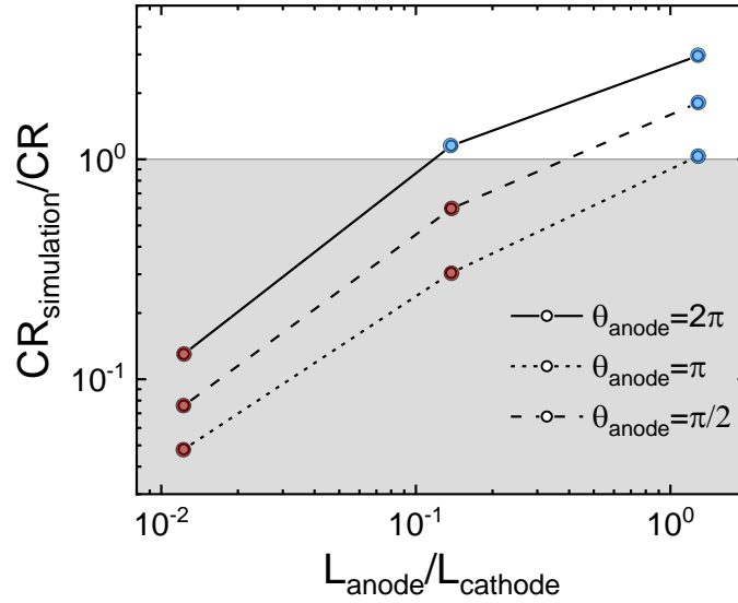
Figure 5.6: The ratio of the corrosion rate obtained from analysis of the simulated impedance and the input corrosion rate as a function of anode to cathode length ratio with anode circumference as a parameter.
