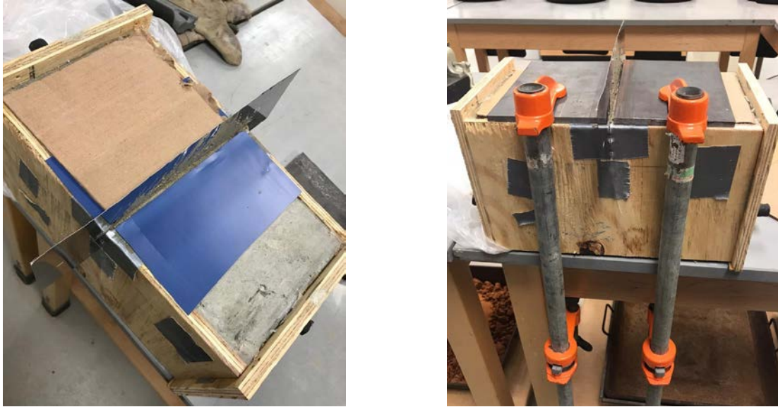
Figure 3.28: Shim removal process to generate local deficiency in concrete specimens.
