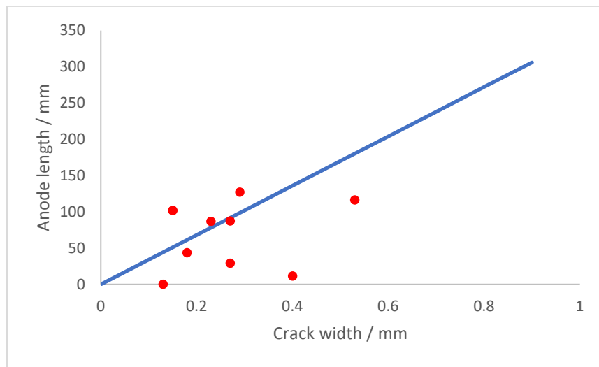
Figure 4.17: Anode length as a function of crack width. The line represents the empirical Equation (28) developed for CS. The points represent experimental results of SS taken from Niejenhuis. 35
