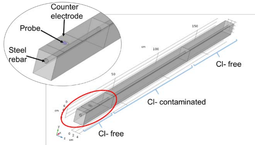
Figure 3.11: 3D model of specimens including chloride-contaminated and chloride-free regions; simulation of EIS test.
