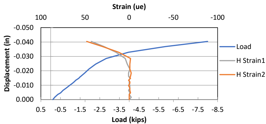
Figure 4.7: Horizontal strain.
