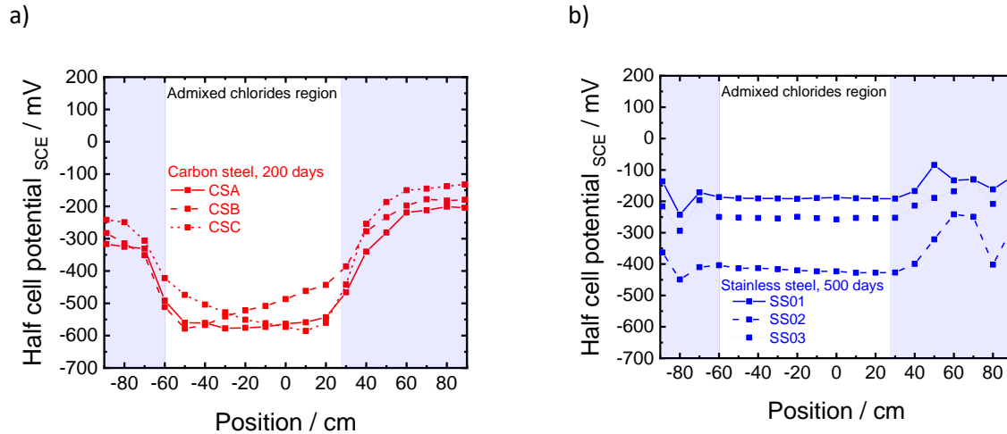
Figure 5.1: HCP results of specimens as a function of location in simulated beam specimens reinforced with (a) carbon steel at 200 days, and (b) stainless steel at 500 days (after \sim 250 days of aggressive ponding and \sim 120 days of heating).
