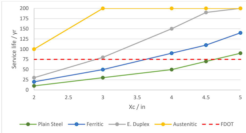
Figure 6.4: Second scenario: life cycle analysis under extremely aggressive conditions as a function of concrete cover for each type of steel.
