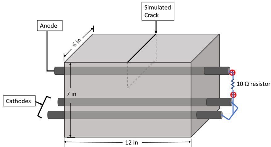
Figure 3.33: Experimental set-up of macrocell current density measurement. Measured across 10-ohm resistor.
