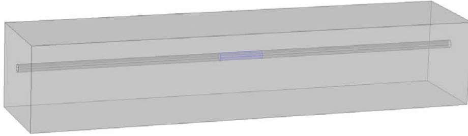
Figure 4.18: Finite element model geometry showing locally corroding anode of length 688 mm corresponding to a crack width of 0.2 mm.
