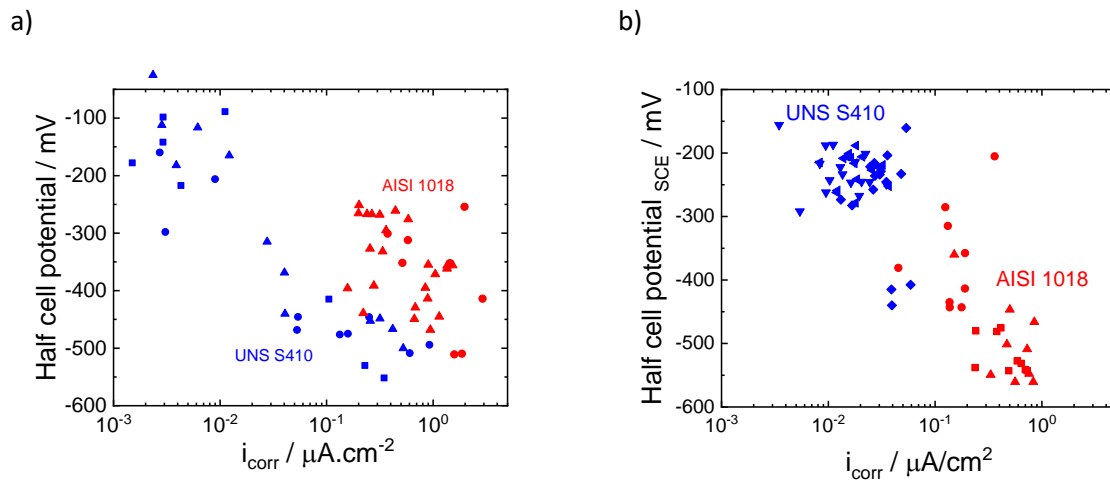
Figure 5.3: Potential as a function of corrosion current density for (a) cylindrical specimens and (b) midpoint of simulated beam with the highest potential drop.
