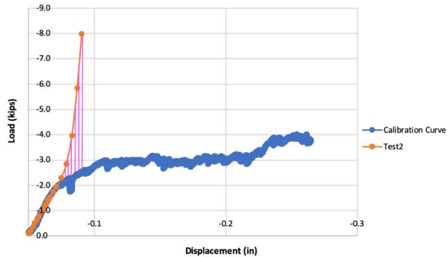
Figure 4.10: Load calibration.
