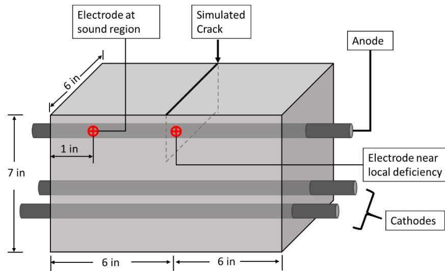
Figure 3.32: Experimental set-up of potential drop between reference electrodes placed near the local deficiency and the sound concrete region of the anode.
