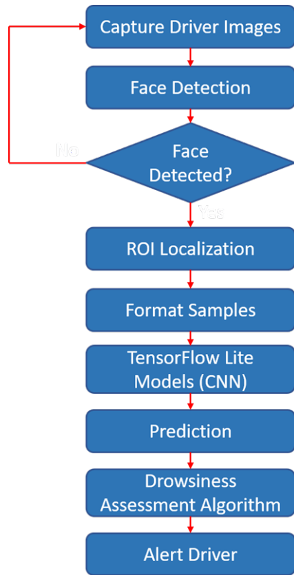
Figure 1. Block Diagram of the Drowsy Driver Detection System.
