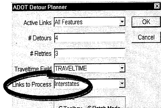
Figure 9 – Batch Mode
