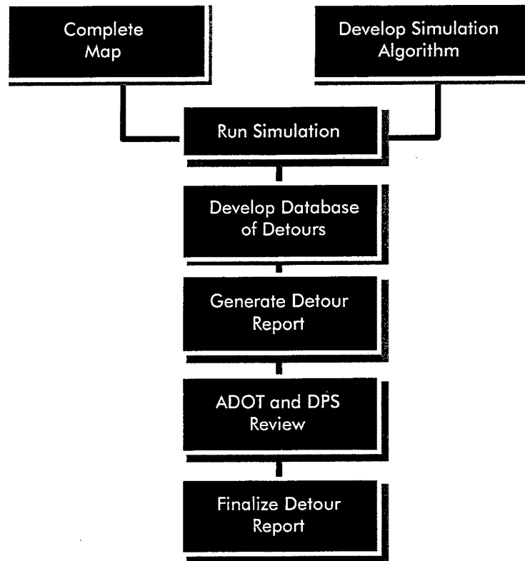
Figure 3 – Task Flowchart
