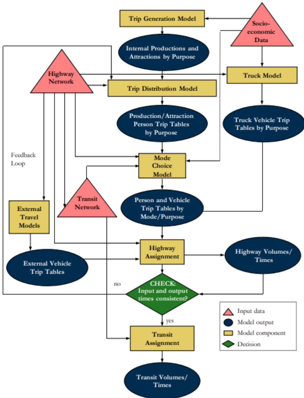
Figure 2.5 TDM Developed by the VDOT (Virginia Department of Transportation, 2014)
