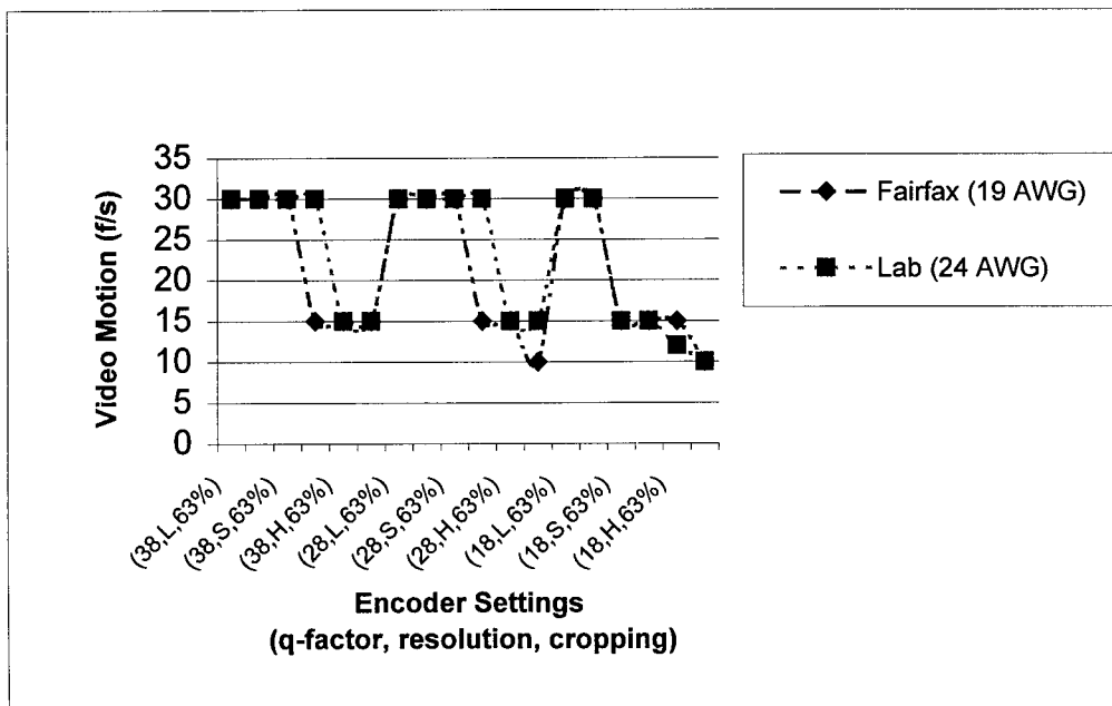
Figure C-8. Video Motion (Fairfax vs. Laboratory); Throughput = 1536 kbps
