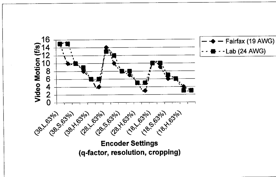
Figure 3-8. Video Motion (Fairfax vs. Laboratory); Throughput = 384 kbps
