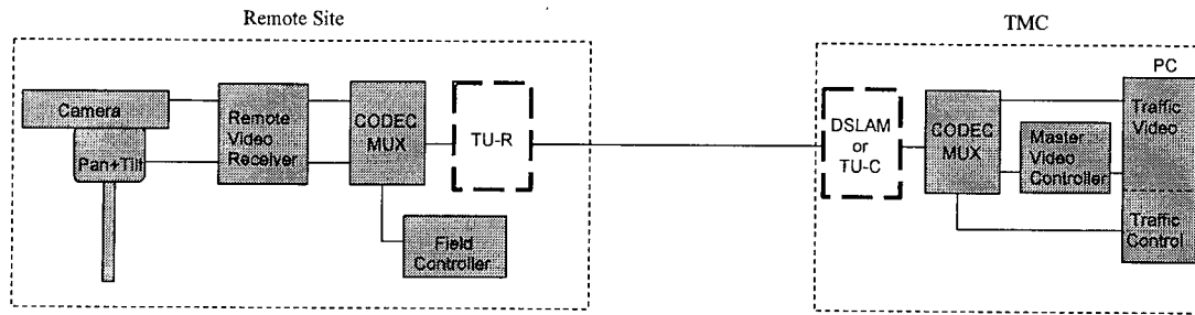
Figure A-1. Base System #2 Configuration
