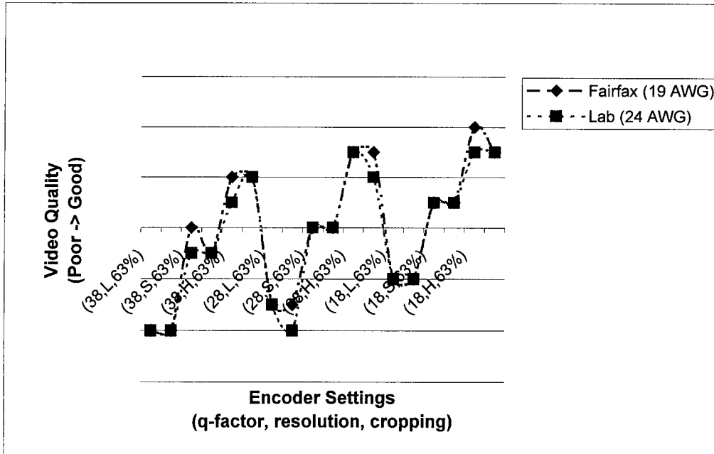
Figure C-3. Video Quality (Fairfax vs. Laboratory); Throughput = 768 kbps
