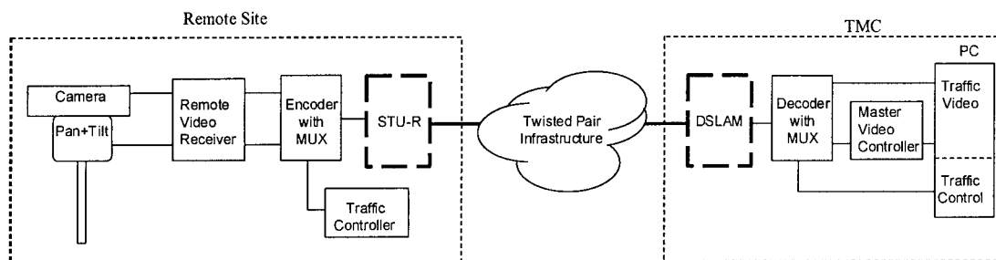
Figure 2-3. SDSL Prototype
