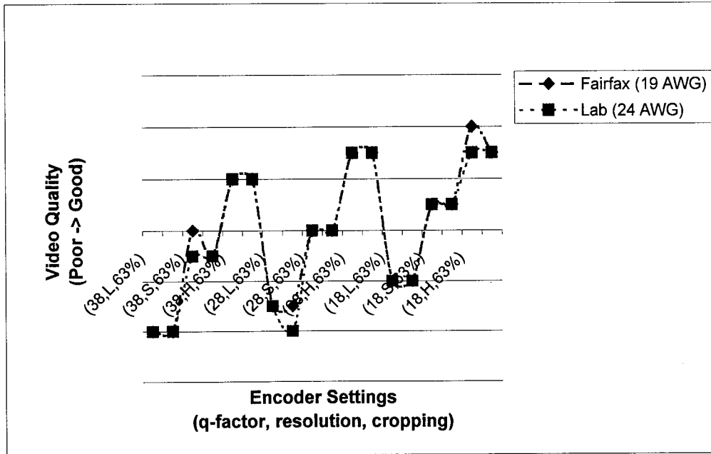
Figure C-1. Video Quality (Fairfax vs. Laboratory); Throughput = 384 kbps
