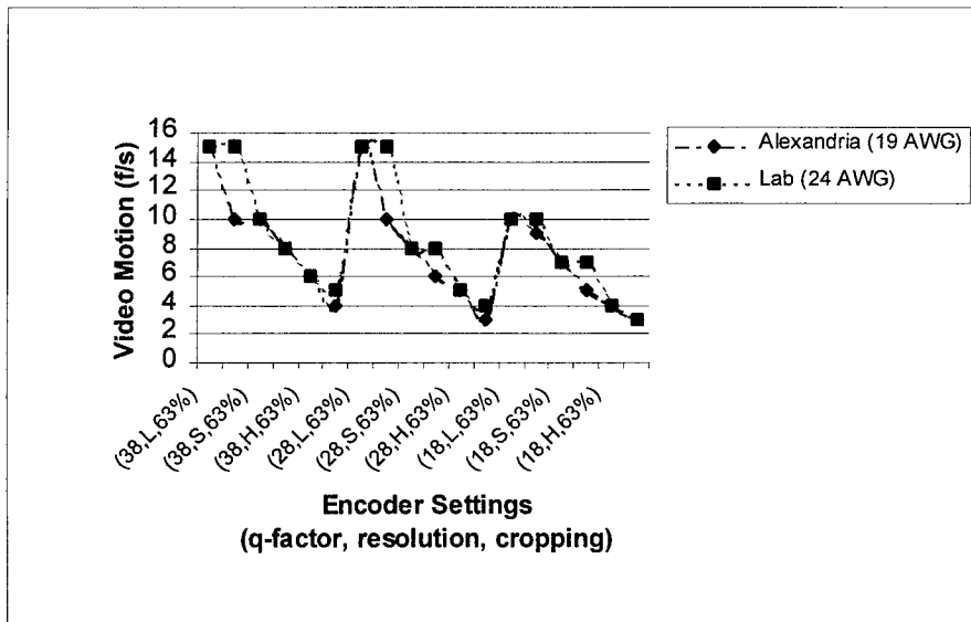
Figure 3-6. Video Motion (Alexandria vs. Laboratory); Throughput = 384 kbps
