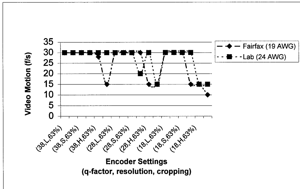
Figure C-10. Video Motion (Fairfax vs. Laboratory); Throughput = 2048 kbps
