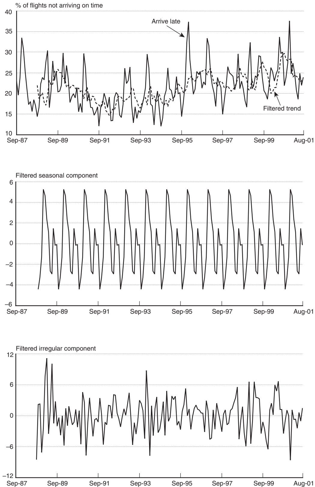
FIGURE 6 Filtered Components of the Late Arrivals Series: September 1987–August 2001 Generated by STAMP
