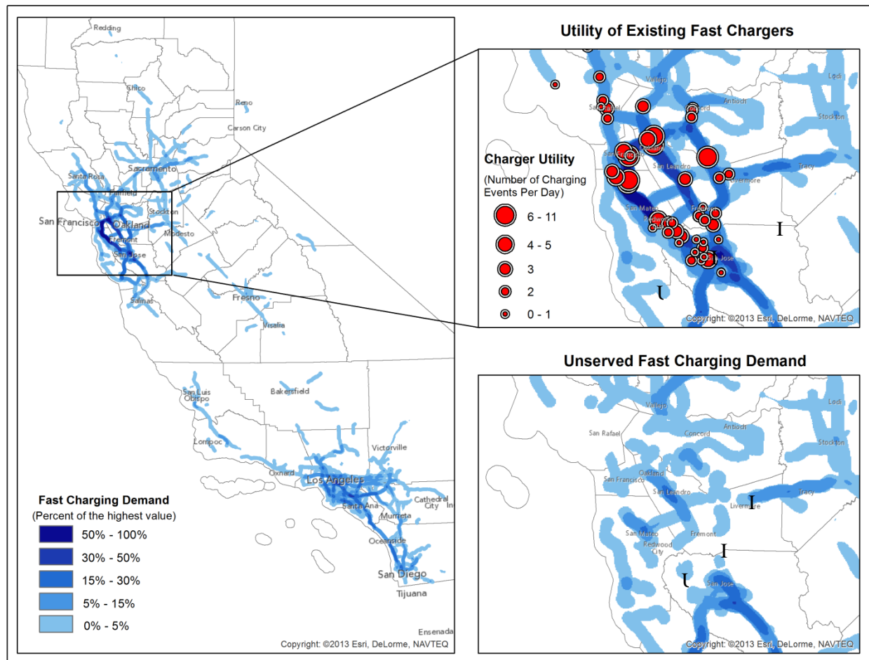
Figure 3.4 Result of present scenario with existing fast chargers
