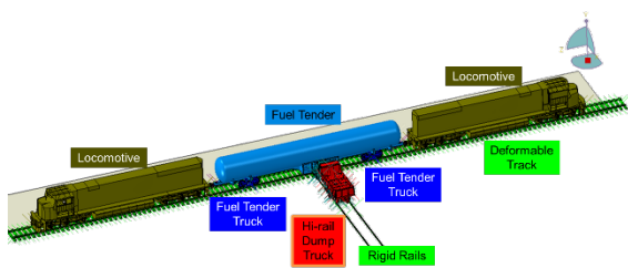
Figure 3. Grade Crossing Impact Scenario FE Model
