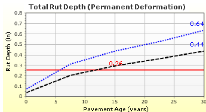
Figure C3. Rutting Prediction Using Different Rutting Coefficients: k_1 \cdot \beta_1 = -5.03118 ; k_2 \cdot \beta_2 = 1.5606 ; k_3 \cdot \beta_3 = 0.4791 .
