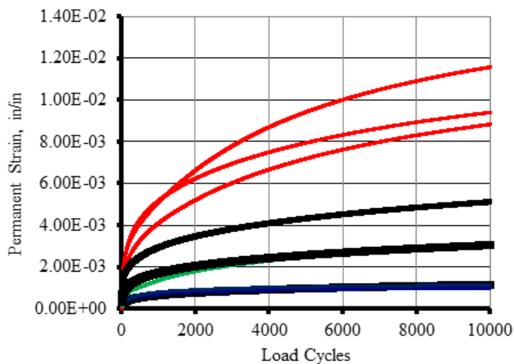
Figure 9. Typical Laboratory Repeated Load Permanent Strain Curve With Three Test Temperatures (Mix 18-1022). Red = data at 54 °C; green and black = data at 35 °C; blue = data at 20 °C.
