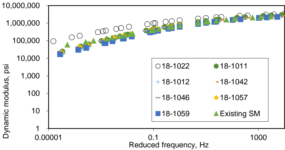
Figure 6. Dynamic Modulus Mastercurves for SM-E Mixtures (Log-Log Scale). SM-E = dense-graded polymer modified.
