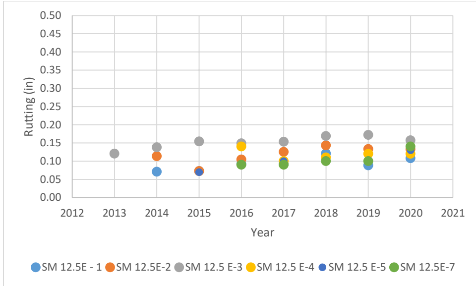
Figure 14. Field Rutting Data for SM-E Mixtures (Paved From 2012-2016). SM-E = dense-graded polymer modified.
