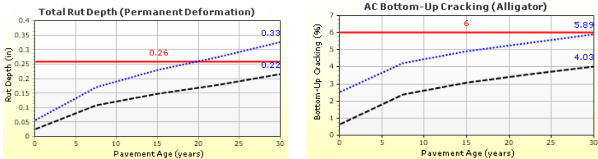
Figure B2. Predicted Rutting and Bottom-Up Cracking (With Existing Catalogued Values for SM, IM, and BM). SM = surface mix; IM = intermediate mix; BM = base mix.
