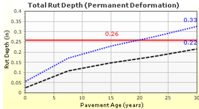
Figure C1. Rutting Prediction Using Existing Rutting Coefficients: k_1 \cdot \beta_1 = -2.304 ; k_2 \cdot \beta_2 = 1.5606 ; k_3 \cdot \beta_3 = 0.4791 .
