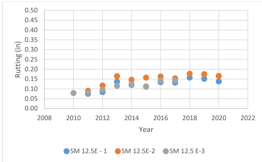
Figure 12. Field Rutting Data for SM-E Mixtures (Paved Before 2011). SM-E = dense-graded polymer modified.
