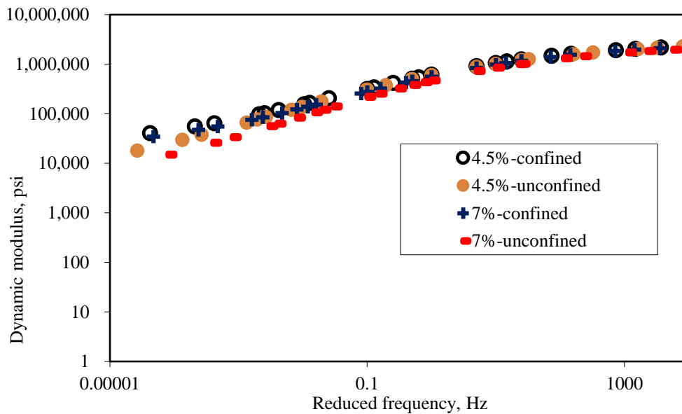
Figure 2. Dynamic Modulus of SMA Mixtures (Confined vs. Unconfined) (Log-Log Scale). SMA = stone matrix asphalt.
