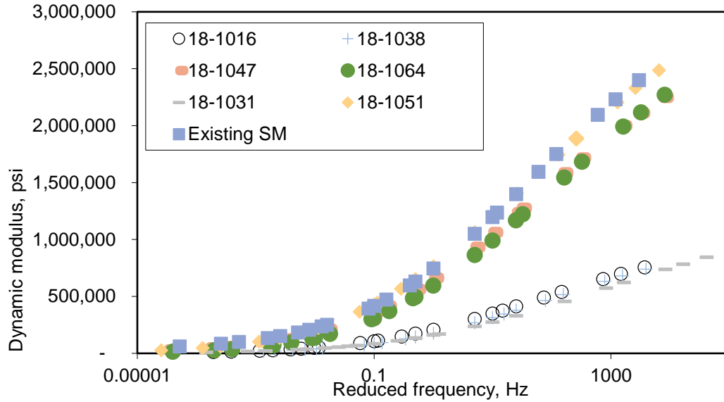
Figure 3. Dynamic Modulus Mastercurves for SMA Mixtures (Semi-Log Scale). SMA = stone matrix asphalt.
