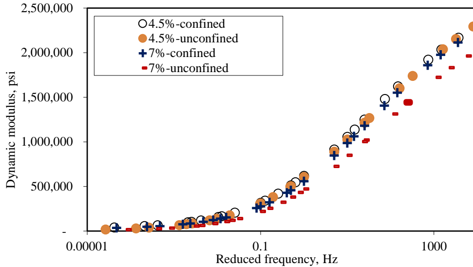
Figure 1. Dynamic Modulus of SMA Mixtures (Confined vs. Unconfined) (Semi-log Scale). SMA = stone matrix asphalt.
