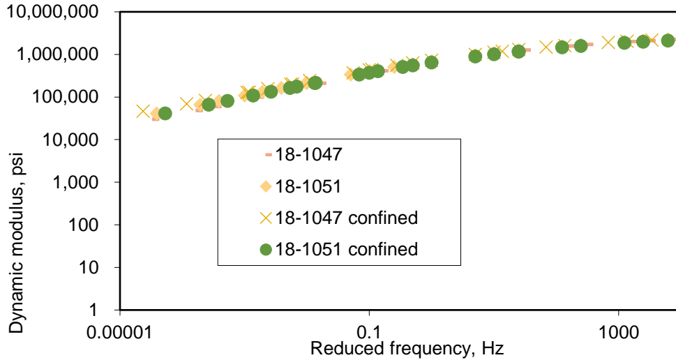
Figure 7. Dynamic Modulus of SMA Mixture (Confined vs. Unconfined) (Log-Log Scale) Using 5 \pm 0.5\% Air Voids
