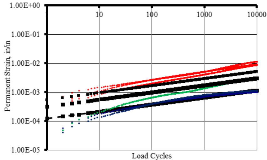
Figure 10. Log-Log Chart of Permanent Deformation Data (Mix 18-1022). Red = data at 54 °C; green and black = data at 35 °C; blue = data at 20 °C.
