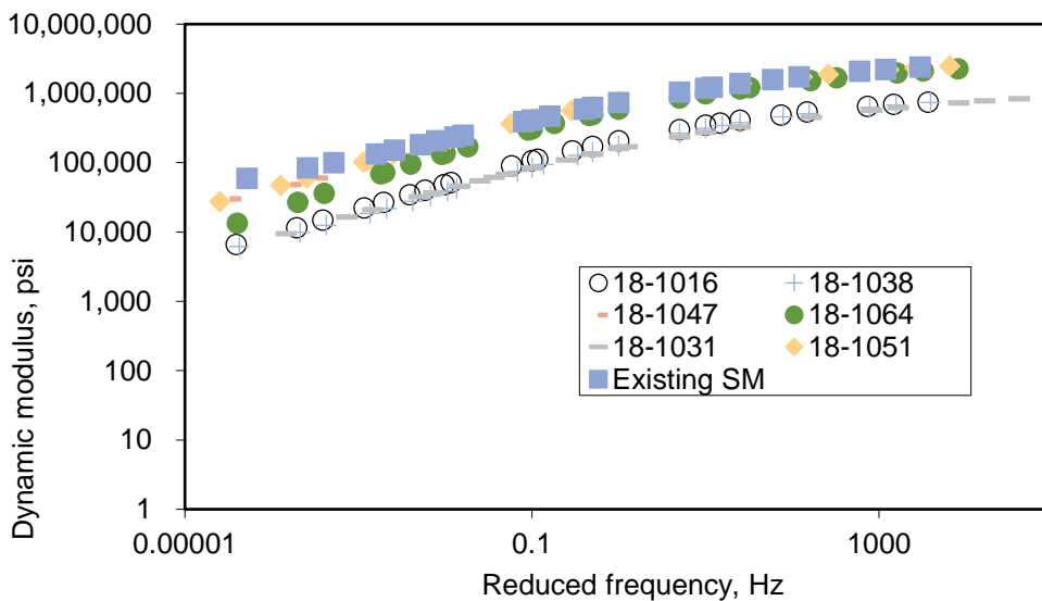
Figure 4. Dynamic Modulus Mastercurves for SMA Mixtures (Log-Log Scale). SMA = stone matrix asphalt.
