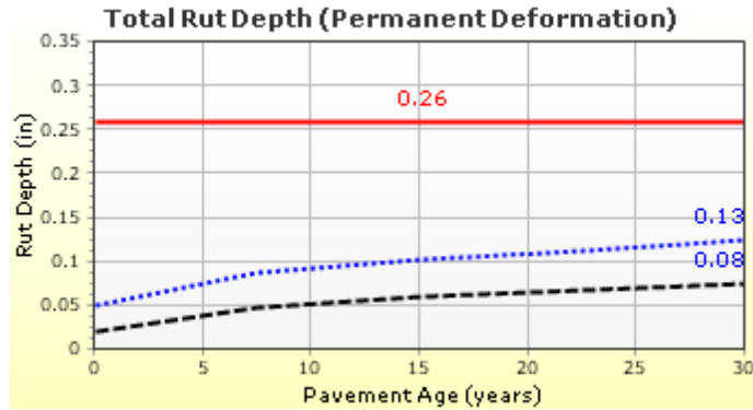
Figure C4. Rutting Prediction Using Different Rutting Coefficients: k_1 * \beta_1 = -5.03118 ; k_3 * \beta_3 = 0.3497 ; k_2 * \beta_2 = 1.5606 .
