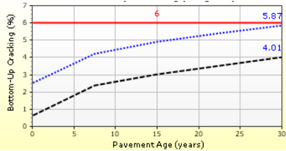
Figure B5. Predicted Rutting and Bottom-Up Cracking With Average SM-E Values From This Study and Existing Values for IM and BM. SM-E = dense-graded polymer modified; IM = intermediate mix; BM = base mix.
