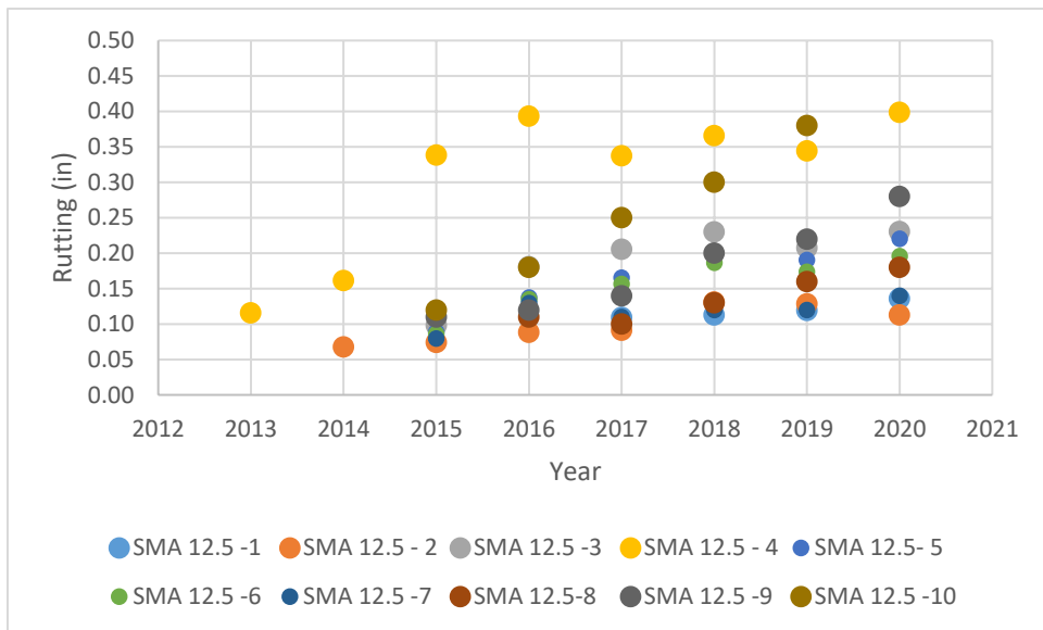
Figure 15. Field Rutting Data for SMA Mixtures (Paved From 2012-2016). SMA = stone matrix asphalt.
