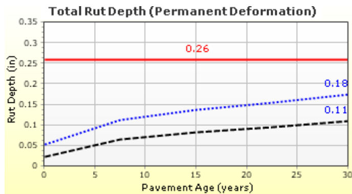
Figure C5. Rutting Prediction Using Different Rutting Coefficients: k_1 * \beta_1 = -5.03118 ; k_3 * \beta_3 = 0.3832 ; k_2 * \beta_2 = 1.5606 .
