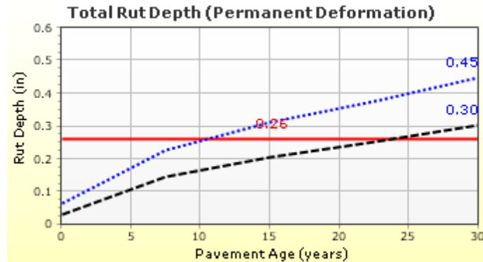
Figure C2. Rutting Prediction Using Different Rutting Coefficients: k_1 \cdot \beta_1 = -3.35412 ; k_2 \cdot \beta_2 = 1.5606 ; k_3 \cdot \beta_3 = 0.4791 .
