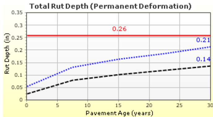
Figure C6. Rutting Prediction Using Different Rutting Coefficients: k_1 * \beta_1 = -6.708 ; k_3 * \beta_3 = 0.3832 ; k_2 * \beta_2 = 1.5606 .
