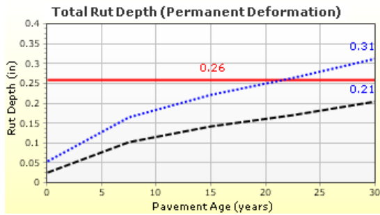
Figure B5. Predicted Rutting and Bottom-Up Cracking With Average SM-E Values From This Study and Existing Values for IM and BM. SM-E = dense-graded polymer modified; IM = intermediate mix; BM = base mix.
