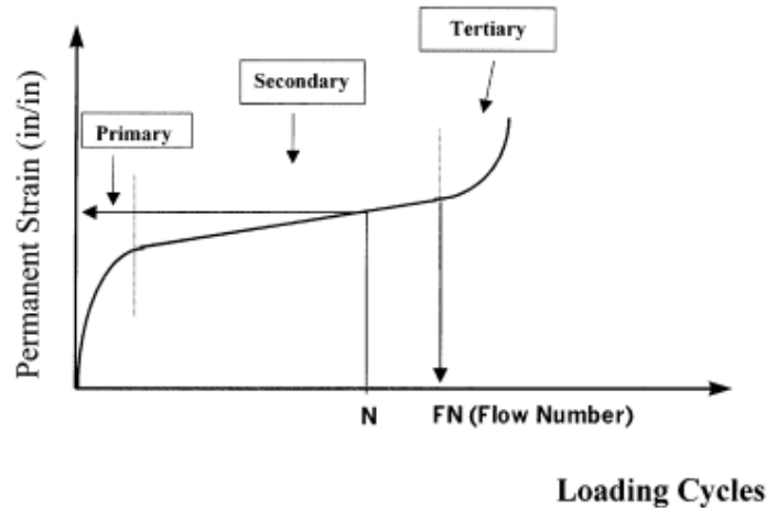
Figure 8. Example of General Relationship Between Permanent Strain and Loading Cycles
