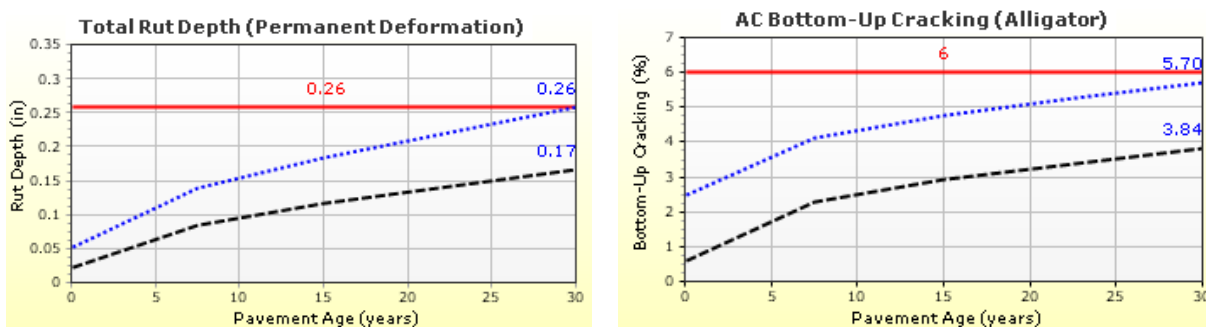
Figure B3. Predicted Rutting and Bottom-Up Cracking (With SM-E Values for Mix 18-1022 and Existing Values for IM and BM). IM = intermediate mix; BM = base mix.
