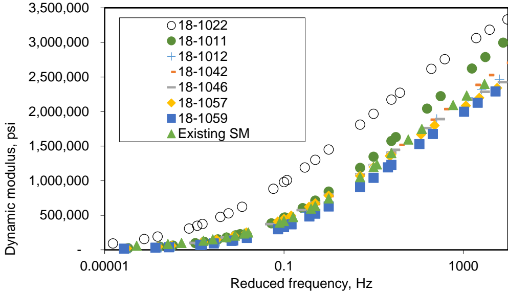
Figure 5. Dynamic Modulus Mastercurves for SM-E Mixtures (Semi-Log Scale). SM-E = dense-graded polymer modified.
