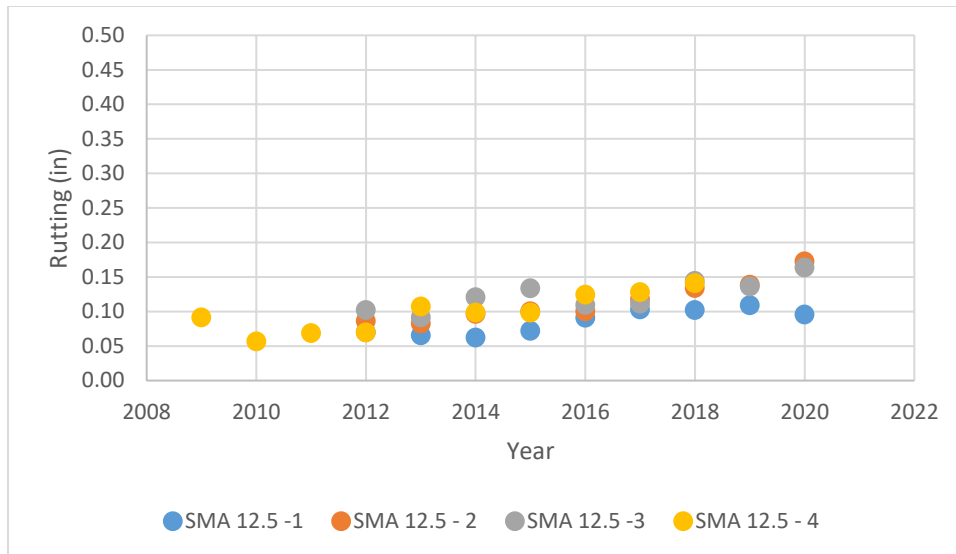
Figure 13. Field Rutting Data for SMA Mixtures (Paved Before 2011). SMA = stone matrix asphalt.
