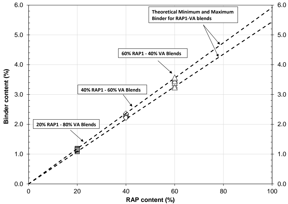
Figure A8: Binder content test results for samples prepared after bucket and pugmill mixing in the field.
