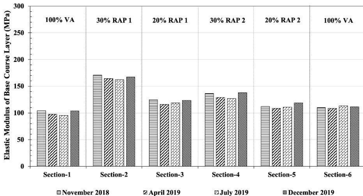
Figure 38: Average Light Weight Deflectometer (LWD) Elastic Modulus Values on Base Course Layer (Four Different Testing Period Time)
