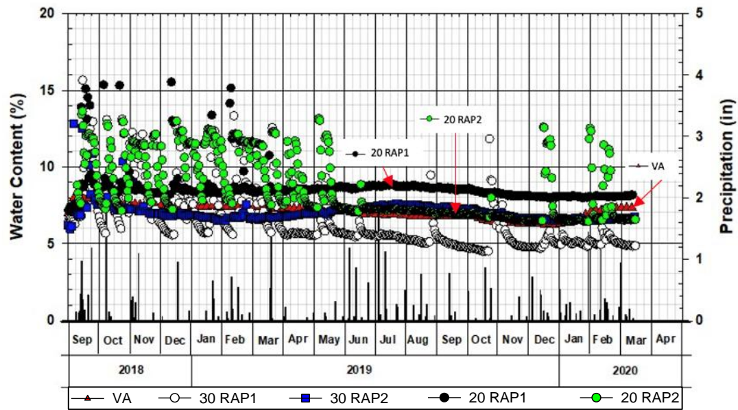
Figure 30: Changes in Field Precipitation and Moisture Contents within the Bottom of Base Course
