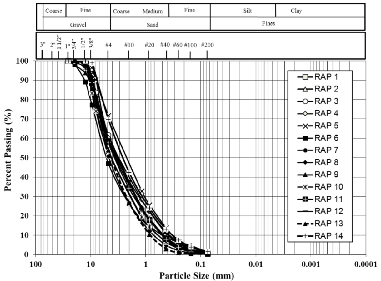
Figure 12: Grain Size Distribution of Collected Reclaimed Asphalt Pavement (RAP) Samples
