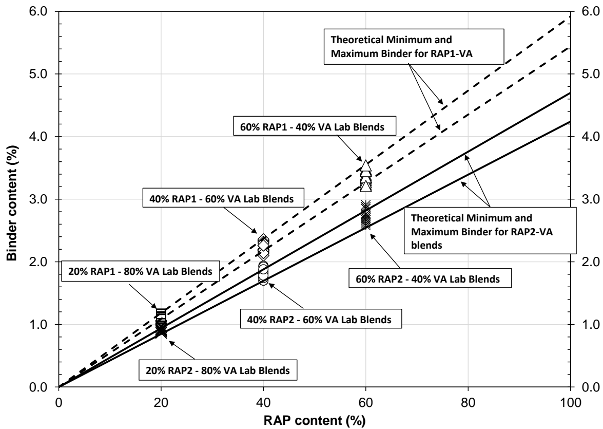
Figure A6: Blends of RAP-VA created at the GMU laboratory
