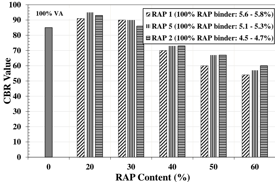
Figure 22: Evaluation of California Bearing Ratio (CBR) of Reclaimed Asphalt Pavement and Virgin Aggregate (RAP-VA) Blends Created with RAP1, 2 and 5 (Parent Rock Diabase)
