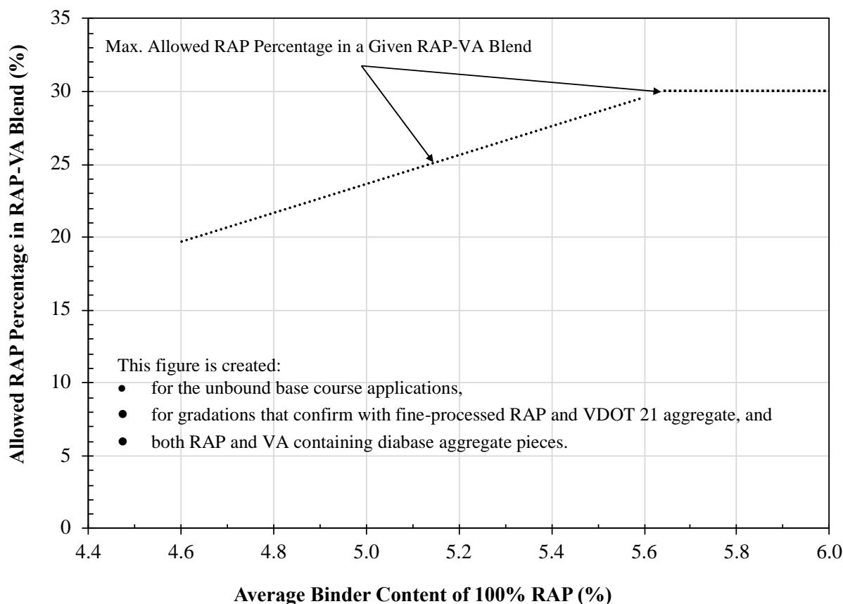
Figure 40: Relationship Between Acceptable RAP Percentage in a Given Reclaimed Asphalt Pavement and Virgin Aggregate (RAP-VA) Blends Based on Average Binder Content of RAP Used to Create the Blends
