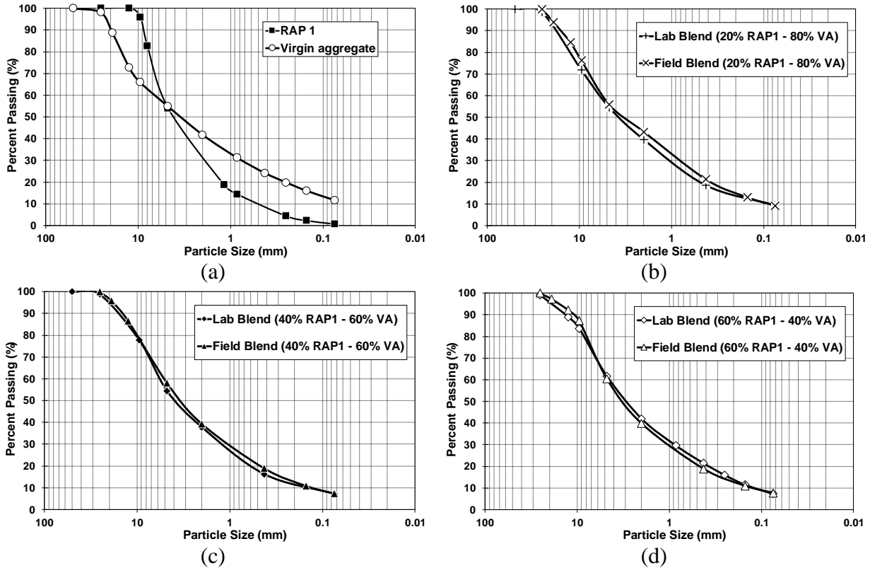
Figure A4: GSD test results for samples prepared after conveyor belt and silo mixing in the field.
