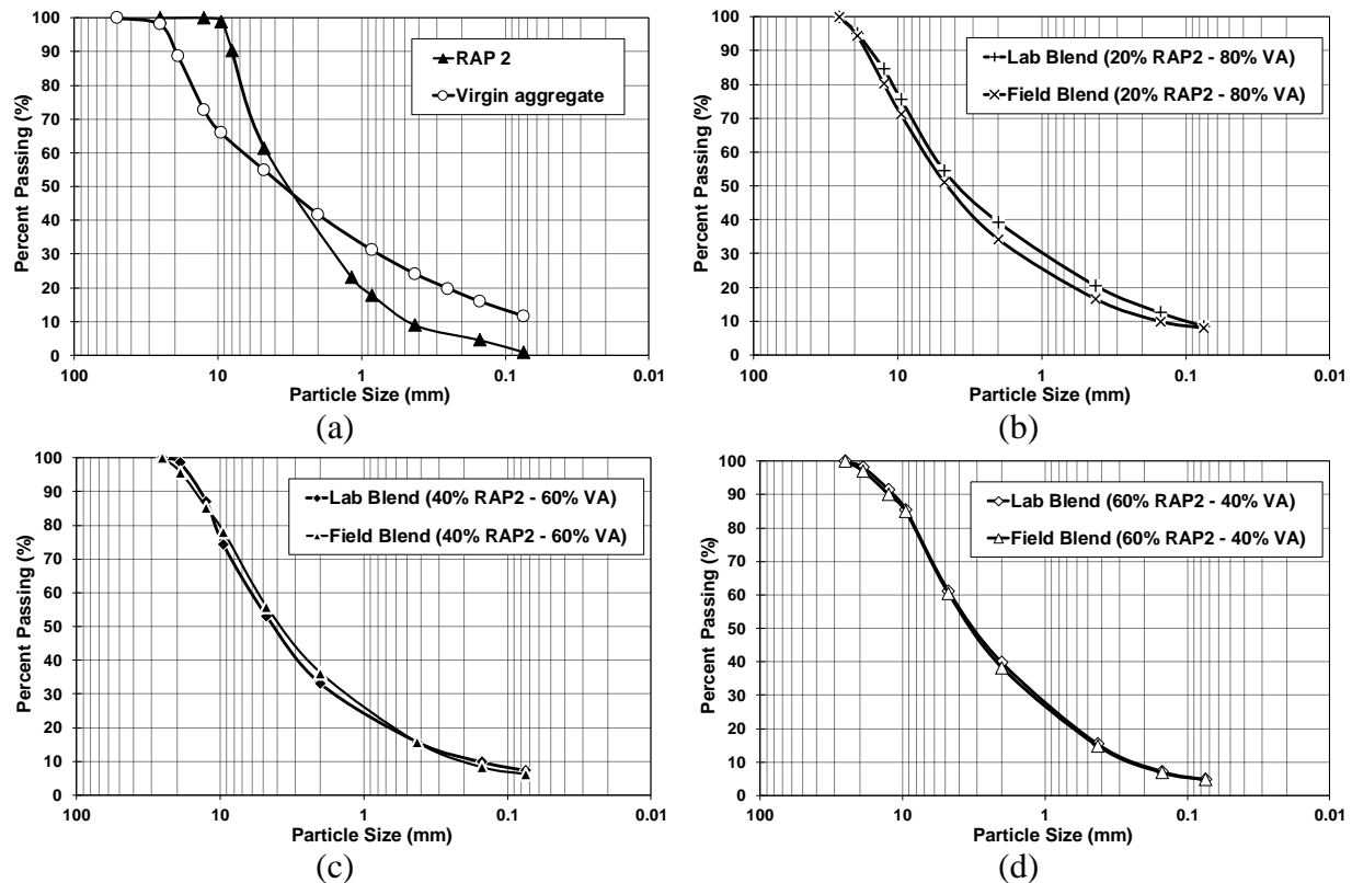
Figure A3: GSD test results for samples prepared after bucket and pugmill mixing in the field.
