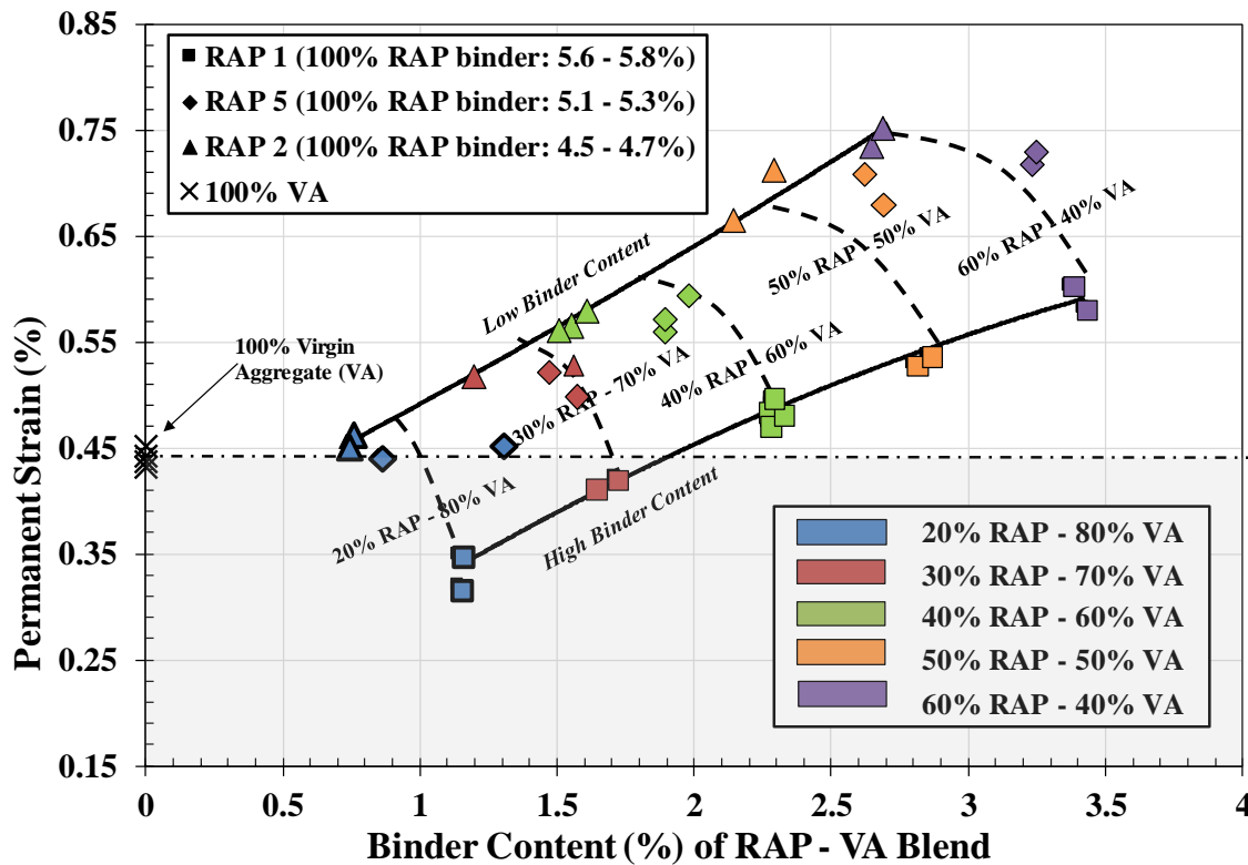
Figure 21: Relationship Between Binder Content of Reclaimed Asphalt Pavement and Virgin Aggregate (RAP-VA) and Percent Strain at the End of 100,000 Load Cycles (Predicted Using Logarithmic Models)
