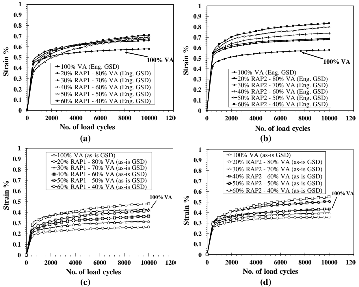
Figure 16: PD Test Results of Reclaimed Asphalt Pavements (RAP) 1 and 2 Blends with Virgin Aggregate (VA) Based on Blends Created with (a) and (b) Engineered (Eng. GSD) and (c) and (d) As-Is (as-is GSD) Mixture Design Approaches
