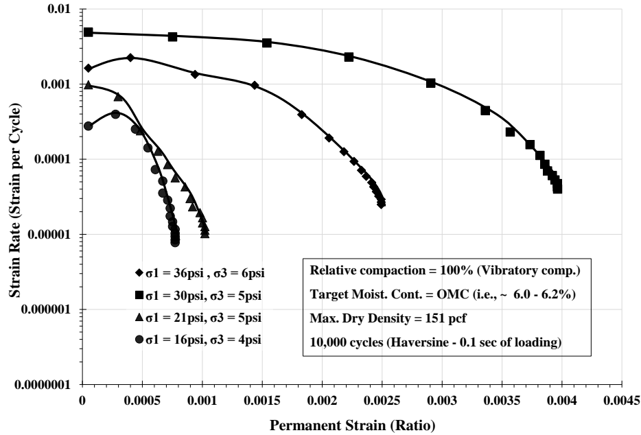
Figure 1: Determination of Stress Levels That Would Yield Maximum Strain in the Permanent Deformation Test
