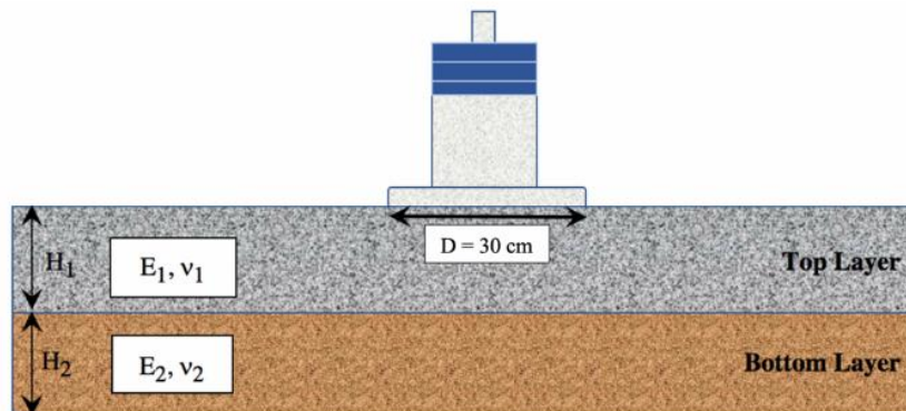
Figure 5: Schematic of the Multilayer System
