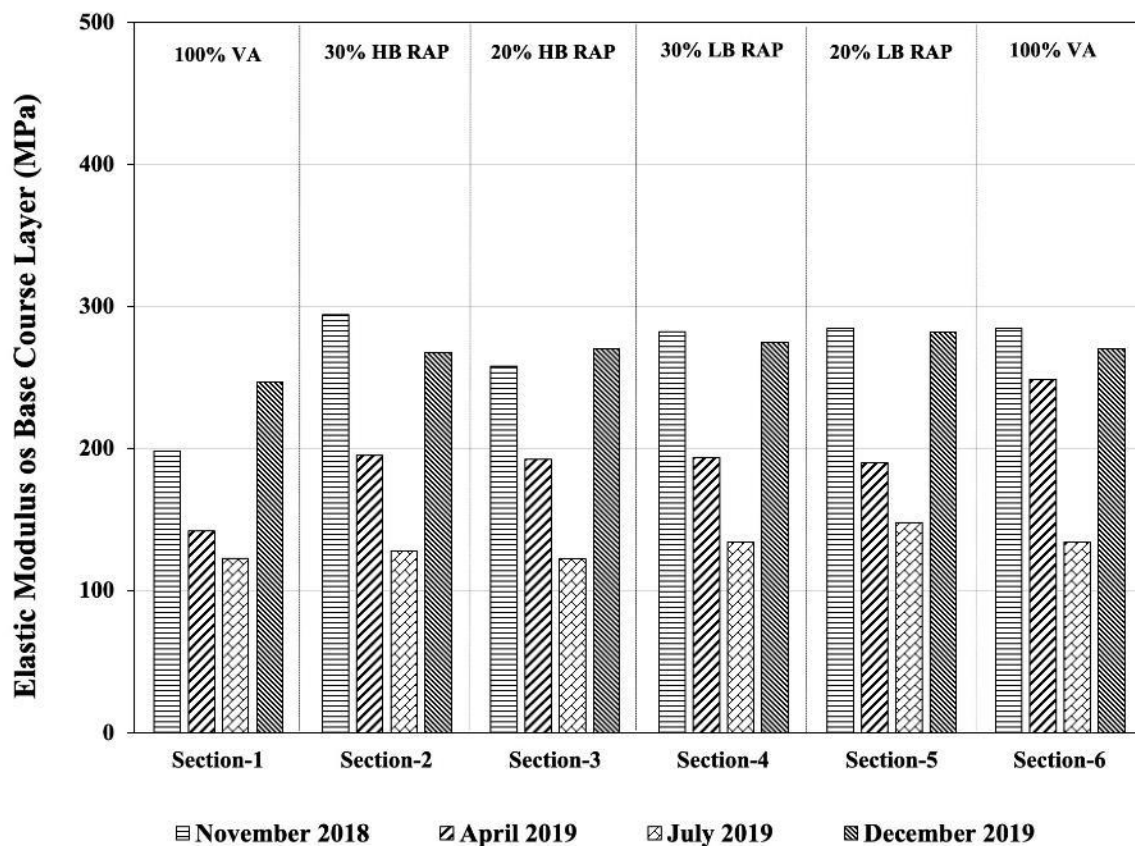
Figure 39: Average Falling Weight Deflectometer (FWD) Elastic Modulus Values of Base Course Layer (Four Different Testing Period Time)
