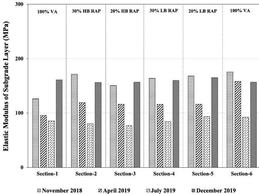
Figure 37: Average Falling Weight Deflectometer (FWD) Elastic Modulus Values on Subgrade Layer (Four Different Testing Period Time)
