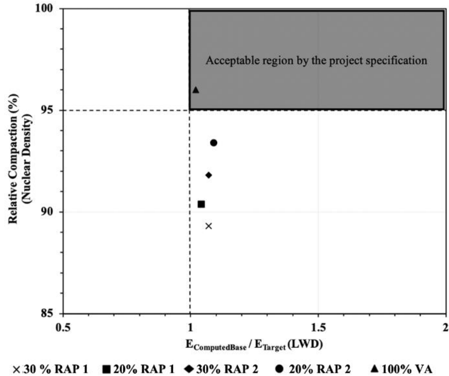
Figure 28: Comparison of Average Ratio of Computed Base Course and Target Modulus Values from Light Weight Deflectometer (LWD) Test Versus Relative Compaction Values Obtained from Nuclear Density Gauge
