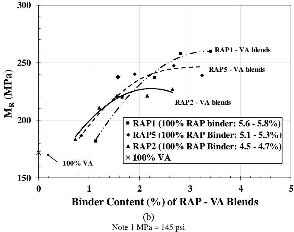
Figure 18: Evaluation of Resilient Modulus ( M_R ) of Reclaimed Asphalt Pavement and Virgin Aggregate (RAP-VA) Blends of RAP with Same Parent Rock but Different Binder Content (a) RAP Percentage and (b) Binder Content within Each Blend
