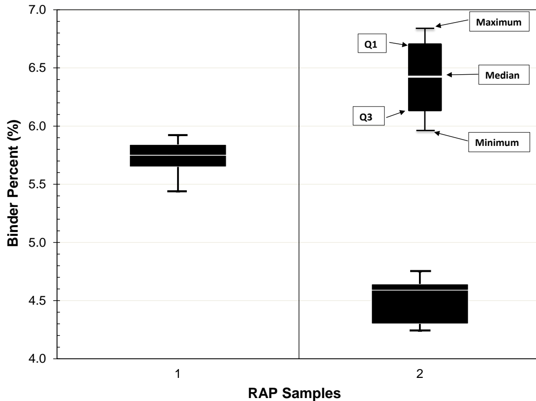
Figure A5: Statistical data on binder content for the selected RAP samples
