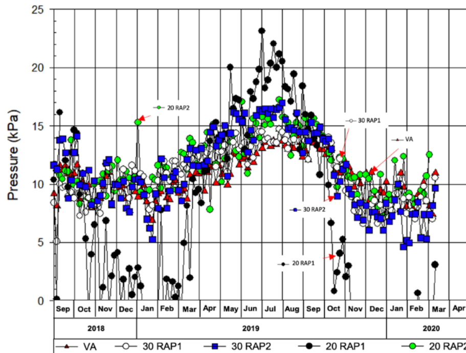
Figure 32: Changes in Vertical Earth Pressures Estimated at the Bottom of Base Course
