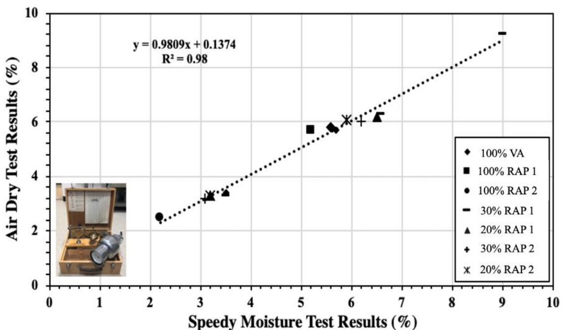
Figure 26: Results of Correlation Tests on Reclaimed Asphalt Pavement and Virgin Aggregate (RAP-VA) Blends with Speedy Moisture Test.
