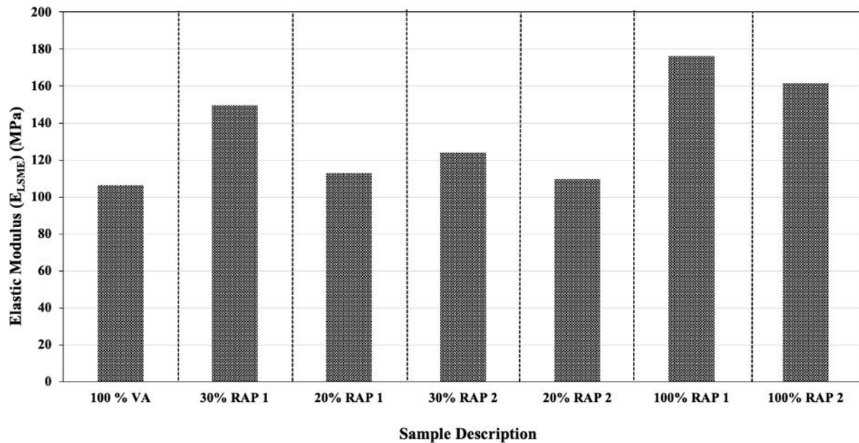
Figure 23: Light Weight Deflectometer (LWD) Test Results Performed in Large Scale Model Evaluation (LSME) Test Pit
