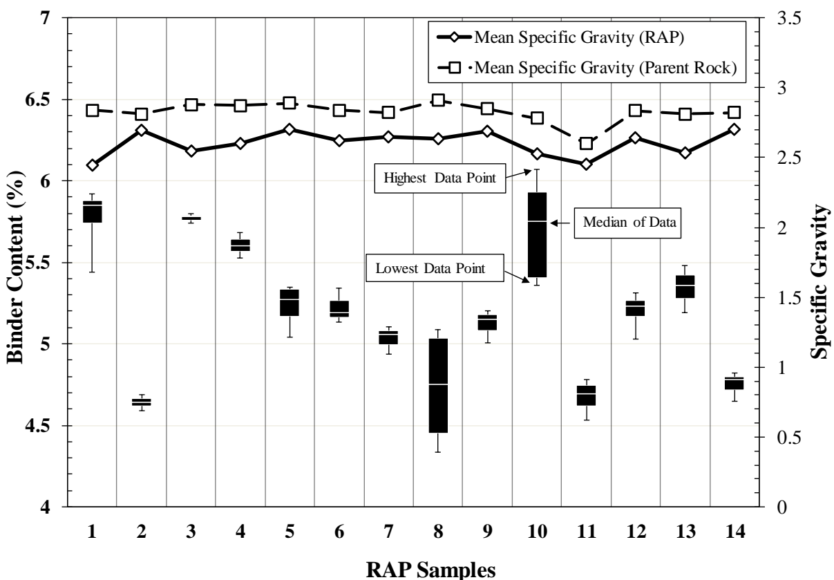
Figure 13: Binder Content and Specific Gravity of Collected 100% Reclaimed Asphalt Pavement (RAP) Samples
