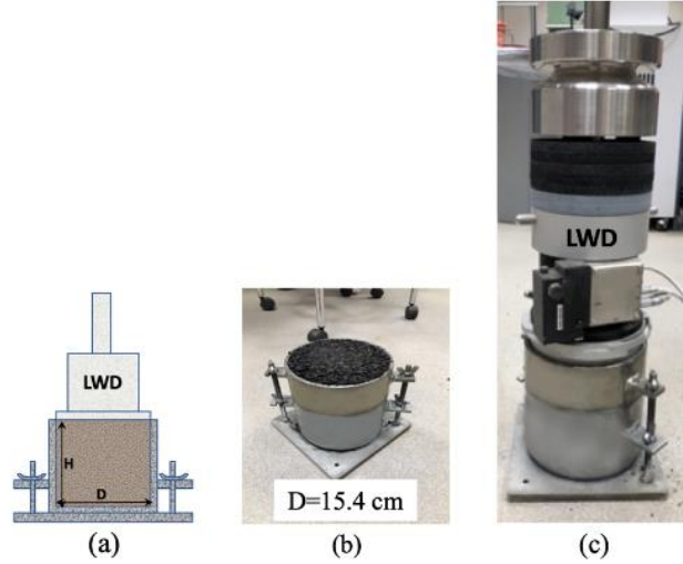
Figure 3: (a) Schematic of the Light Weight Deflectometer (LWD) Test Set-Up with Compaction Mold, (b) Compaction Mold with the Sample, and (c) Photograph of the Assembled Light Weight Deflectometer (LWD) over the Mold
