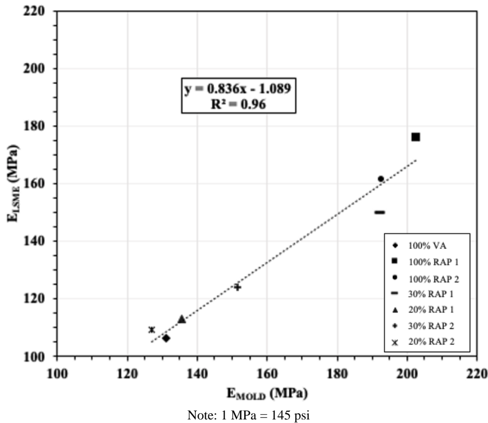
Figure 25: Scale Effects Between Large Scale Model Evaluation (LSME) - Light Weight Deflectometer (LWD) and 6-in Mold - Light Weight Deflectometer (LWD) Tests
