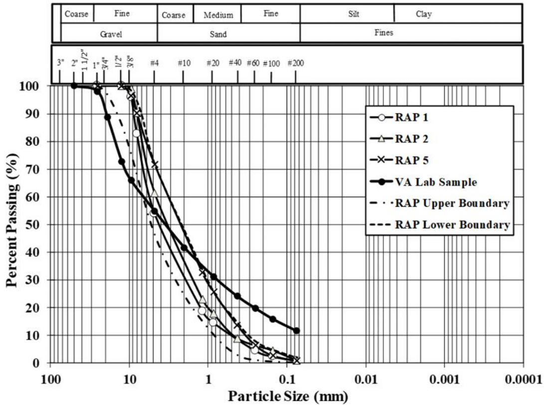
Figure 14: Grain Size Distribution of Reclaimed Asphalt Pavement (RAP) and Virgin Aggregate (VA) Samples Selected for This Study to Create RAP-VA Blends
