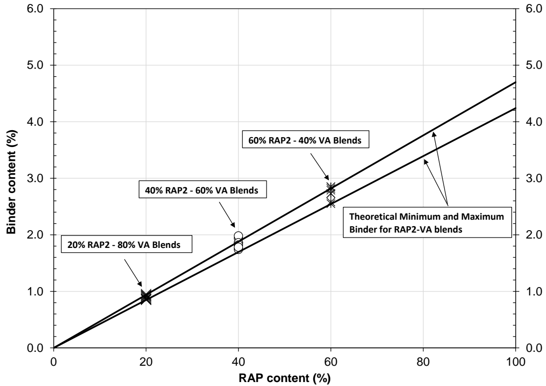
Figure A7: Binder content test results of samples prepared after conveyor belt and silo mixing in the field.
