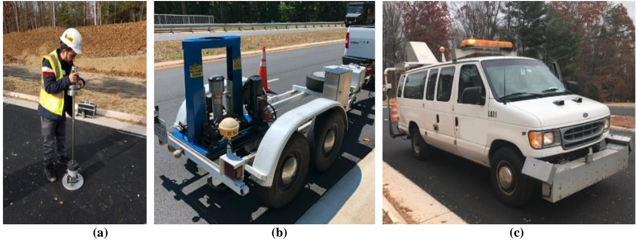
Figure 10: Testing Devices Used in This Research (a) Light Weight Deflectometer, (b) Falling Weight Deflectometer, and (c) International Roughness Index
