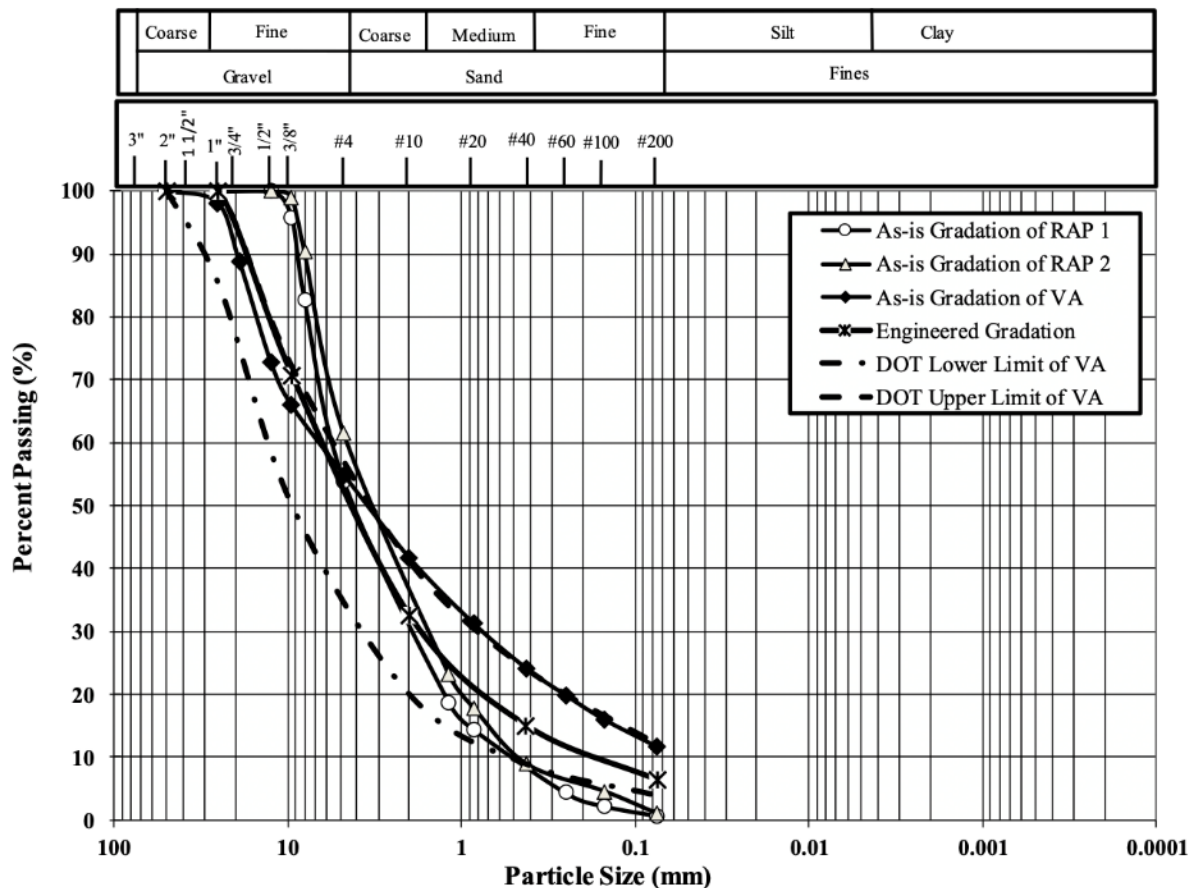
Figure 15: Grain Size Distribution of Reclaimed Asphalt Pavement (RAP) and Virgin Aggregate (VA) Samples Compared with Engineered Gradation
