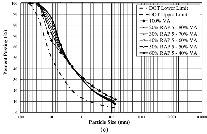
Figure 17: Grain Size Distribution of Blends with (a) RAP 1, (b) RAP 2, and (c) RAP 5 (Mixed by Weight)
