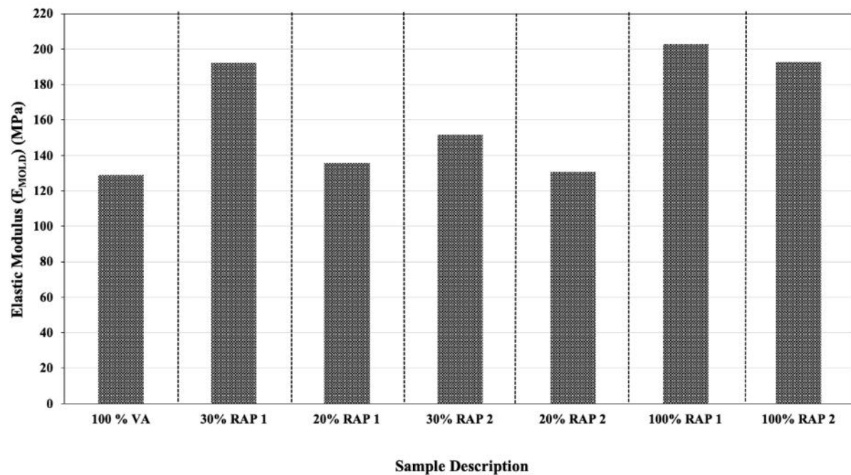
Figure 23: Light Weight Deflectometer (LWD) Test Results Performed in Large Scale Model Evaluation (LSME) Test Pit
