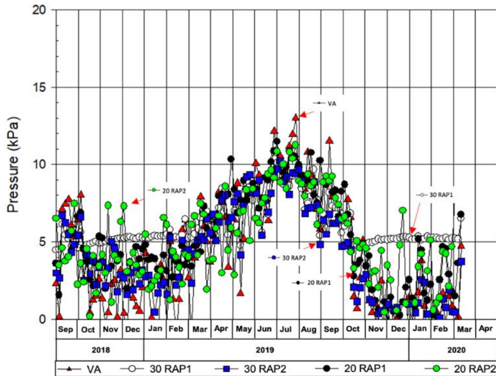
Figure 33: Changes in Vertical Earth Pressures Estimated at the Bottom of Asphalt Layer
