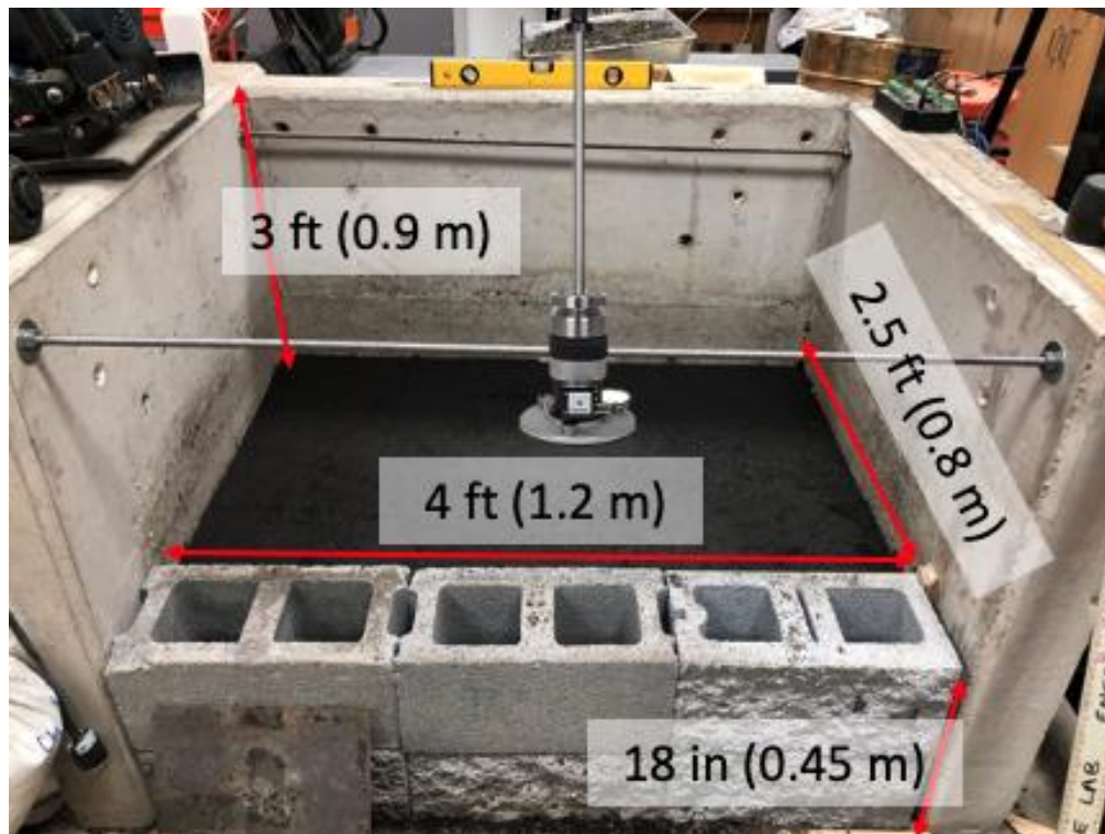
Figure 2: Large Scale Model Evaluation (LSME) Set-Up Used to Test Suitability of Light Weight Deflectometer (LWD) in George Mason University's Sustainable Geo Infrastructure (SGI) Laboratory
