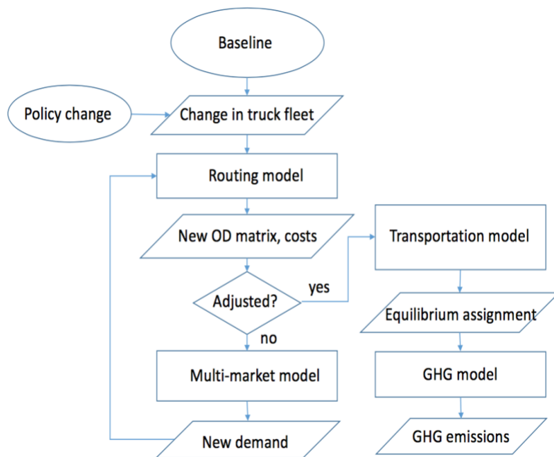
Figure 1. Model Structure
