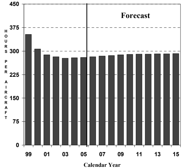
ROTORCRAFT
