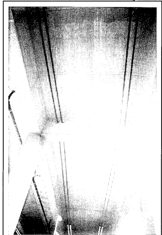
Figure 8. Underside of a typical post-tensioned concrete girder highway viaduct on the A59 route near Cologne, Germany, recently rehabilitated with external longitudinal tendons.
