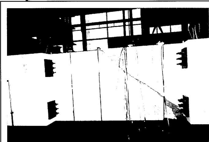
Figure 42. Carbon fiber shear reinforcing test, Swiss Federal Institute of Technology (ETH), Zurich.
