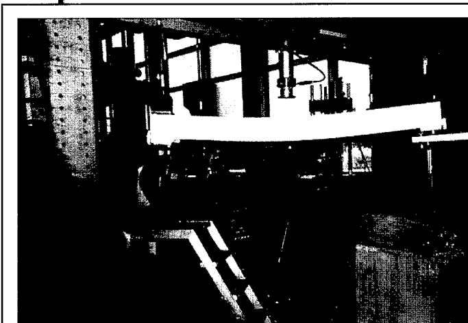
Figure 43. Fiber-reinforced concrete slab test at Swiss Federal Institute of Technology (ETH).
