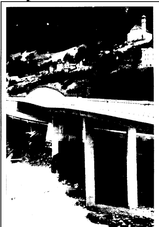
Figure 21. A main pier of the Reuss Bridge, at Wassen, was undermined by scour from excessive flash floods in 1987, but the bridge remained intact.
