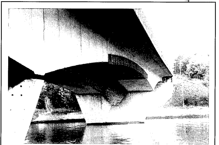
Figure 28. The Corbeil Bridge, Francilienne, Essone, France, on which external transverse post-tensioning was added to the midspan region.
