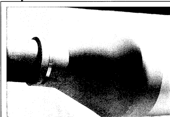
Figure 34. Cable-stay boot connects the external stay pipe to the transition pipe at the anchors on Sunniberg Bridge.
