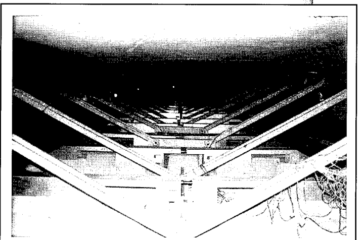
Figure 29. Internal frames on Corbeil Bridge brace the bottom slab and webs. External longitudinal tendons run inside the box near the webs.
