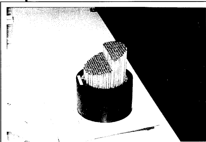
Figure 33. Cable stay of Sunniberg Bridge, Switzerland, consists of parallel wires in a matrix inside a thick-walled PE pipe.
