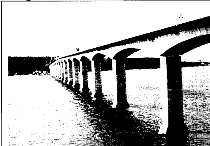
Figure 9. Sallingsund (1979) was the first bridge in Denmark built in balanced cantilever with precast segments and epoxy-glued joints.
